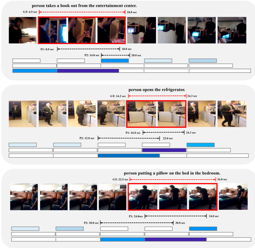
Fig. 6. At inference time, VLANet successfully retrieves the moment described by the query. Due to the limited space, only some proposals are visualized. The color indicates the attention strength. The top-2 predicted moments are visualized with the temporal boundaries. (Color figure online)
