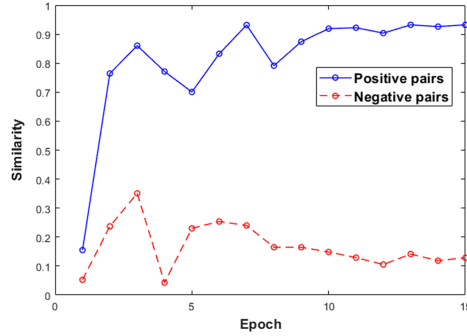
Fig. 4. The multi-modal similarity prediction by VLANet on the positive and negative pairs while training. The similarity gap increases as epoch increases. (Color figure online)
