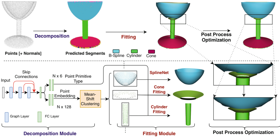
Fig. 2. Overview of PARSENET pipeline. (1) The decomposition module (Sect. 3.1) takes a 3D point cloud (with optional normals) and decomposes it into segments labeled by primitive type. (2) The fitting module (Sect. 3.2) predicts parameters of a primitive that best approximates each segment. It includes a novel SPLINE NET to fit B-spline patches. The two modules are jointly trained end-to-end. An optional postprocess module (Sect. 3.3) refines the output.
