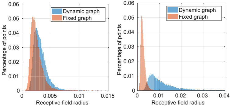
Fig. 5. Radius of receptive field of points at the output of residual block with respect to its input. Left: first residual block. Right: second residual block. Neighbor selection in the noisy 3D space for fixed graph and in the feature space for dynamic graph. Radius is measured as the 90 percentile Euclidean distance to the points in the receptive field on the clean 3D point cloud. (Color figure online)
