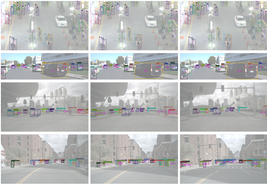
Fig. 3. Qualitative results on MOT (1st row), KITTI (2nd row), and nuScenes (3rd and 4th rows). Each row shows three consecutive frames. We show the predicted tracking offset in arrow. Tracks are coded by color. Best viewed on the screen. (Color figure online)
