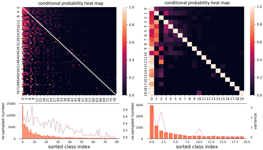
Fig. 5. In the matrix heatmap, the element in the i^{\text{th}} column, j^{\text{th}} row represents the conditional probability of class existence, p(i|j) , which is usually higher for head and medium classes. The histograms below show the data distribution after re-sampling, confirming that the imbalance is not eliminated by re-sampling. The sampling frequency for each instance is different, and the line chart shows the variance within each class. The high variance at the head indicates inner-class imbalance
