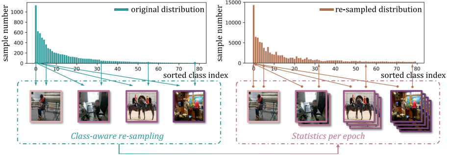
Fig. 2. Visualization of the class-aware re-sampling procedure, and the sample number distribution before (left) and after (right) re-sampling. The distribution may not necessarily be balanced due to label co-occurrence, and the unexpected sampling by associated labels introduces inner-class imbalance
