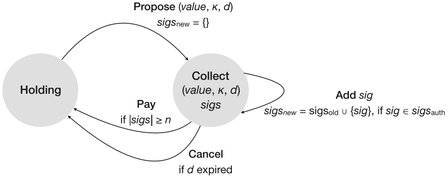
Fig. 1. Transition diagram for the multi-signature state machine; edges labelled with input from redeemer and transition constraints.
