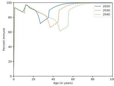
Fig. 1. Projected percentages of immune individuals by age for 2020 (solid blue line), 2030 (dashed orange line) and 2040 (dotted green line). (Color figure online)
