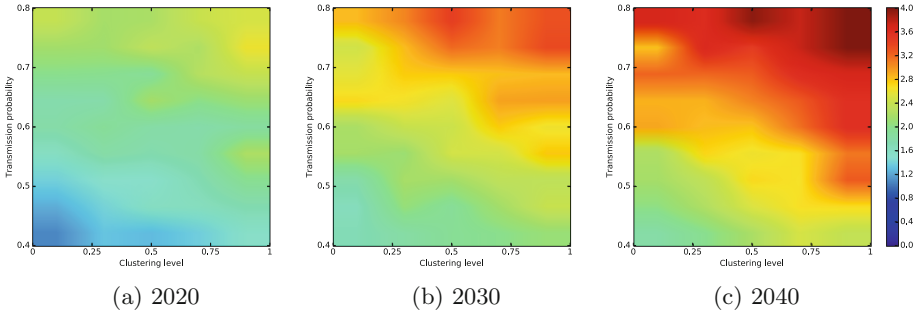
Fig. 4. Heat-maps of the Effective R by P_{\text{transmission}} and clustering level for 2020 (a), 2030 (b), and 2040 (c).
