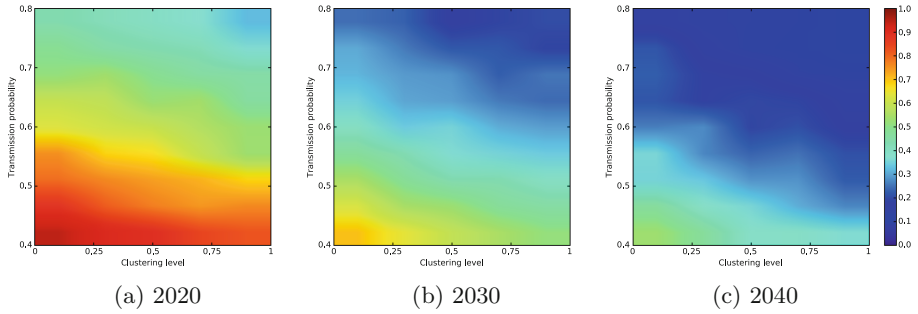
Fig. 5. Average escape probability by P_{\text{transmission}} and clustering level for 2020 (a), 2030 (b), and 2040 (c).
