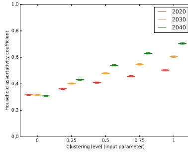
Fig. 3. Distribution of household assortativity coefficients by input clustering level for simulations for 2020 (red), 2030 (yellow) and 2040 (green). (Color figure online)
