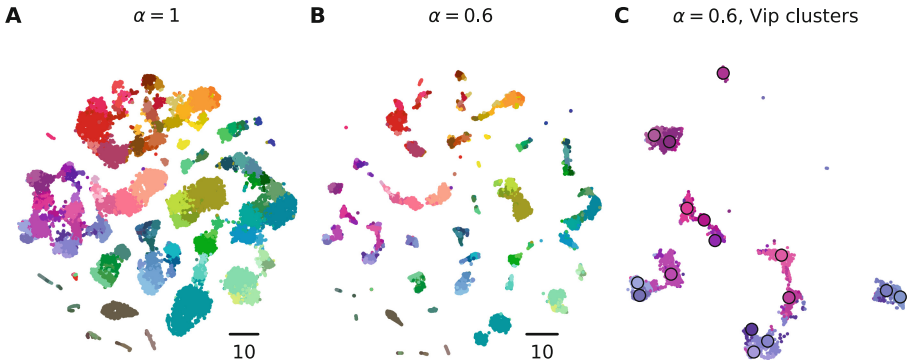
Fig. 5. Tasic et al. data set ( n = 23\,822 ). (A) Standard t-SNE visualisation ( \alpha = 1 ). Cluster ids and cluster colours are taken from the original publication [16]: cold colours for excitatory neurons, warm colours for inhibitory neurons, and grey/brown colours for non-neural cells such as astrocytes or microglia. (B) t-SNE visualisation with \alpha = 0.6 . (C) A zoom-in into the left side of panel (B) showing all Vip clusters from Tasic et al. Black circles mark cluster centroids (medians). (Color figure online)
