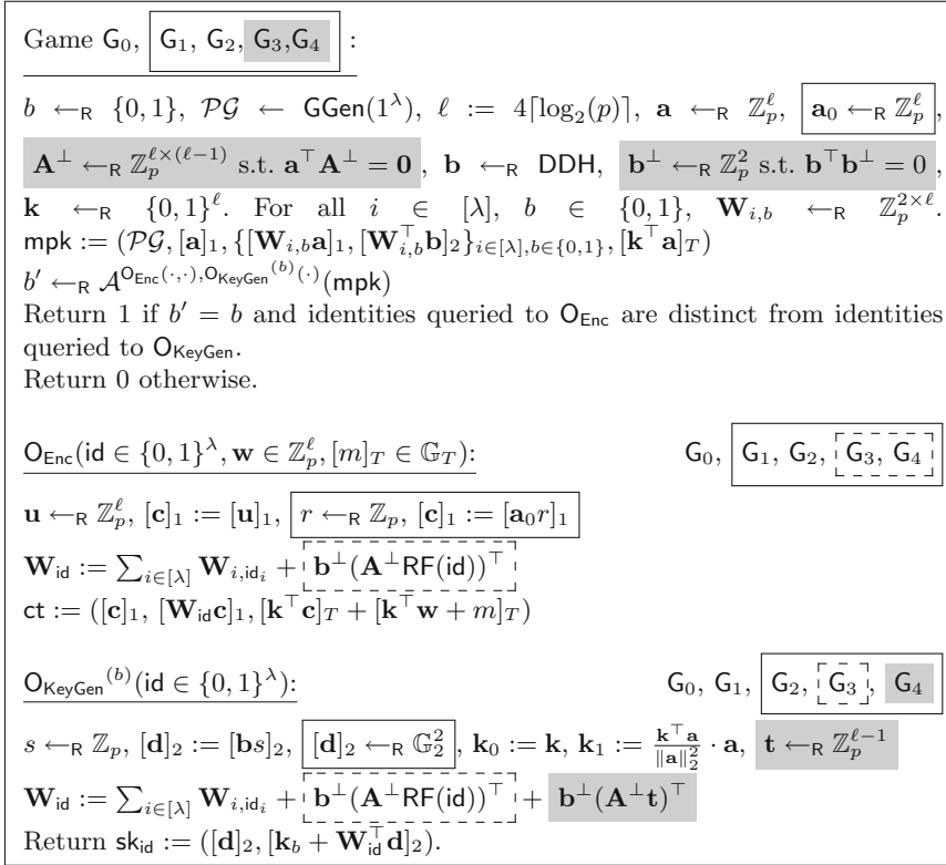
Fig. 9. Games for the proof of Property 2. In each procedure, the components inside a solid (dotted, gray) frame are only present in the games marked by a solid (dotted, gray) frame. Here, \text{RF} : \{0, 1\}^\lambda \rightarrow \mathbb{Z}_p^{\ell-1} denotes a random function that is computed on the fly.
