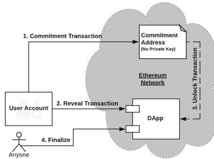
Fig. 7. Submarine Send [18]. User generates an Unlock transaction from which the commitment address is retrieved using ECDSA ECTrecover. 1. by funding the commitment address , user is committed to the transaction. 2. User sends the reveal transaction to the DApp, revealing the nature of the commitment transaction. 3. She broadcasts the unlock transaction to unlock the funds in the commitment address. 4. After the “Auction” is over, anyone can call Finalize function to finalize the process.
