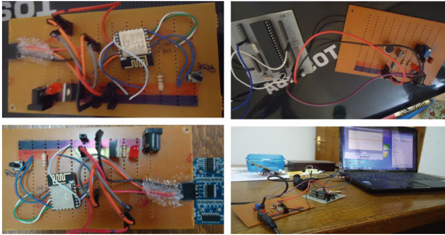
Fig. 4 Prototype of sensor installation
