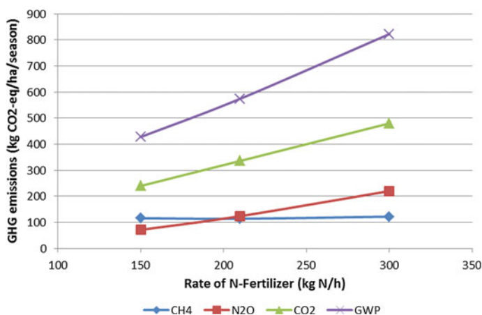
Fig. 7 Cumulative of GHG emissions from different fertilizer applications during rice growing season, GWP = Global warming potential. Source data Zhang et al. [55]
