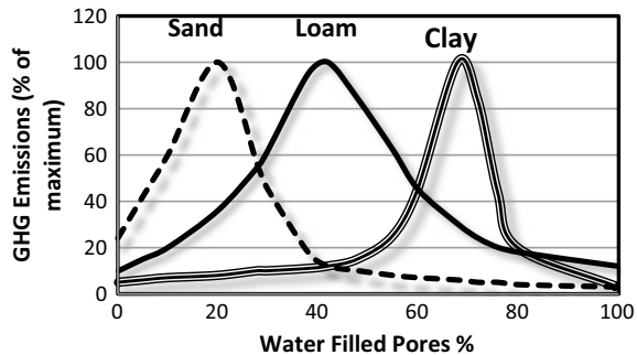
Fig. 4 The relationship between soil GHG emissions and water-filled pores from different soil textures. Based on data in Schindlbacher et al. [25] and adapted from Pilegaard [26]
