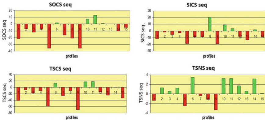
Fig. 2 Negative and positive sequestration rates of soil C and N stocks as drawn from (Table 2). Source Elbasiouny [81]. SOCS: soil organic C stock; SICS: soil inorganic C stock; TSCS: total soil C stock; TSNS: total soil N stock; seq.: sequestration
