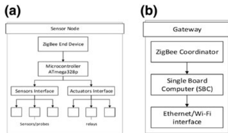
Fig. 2 WSN system in greenhouse for air, water and soil quality parameters control
