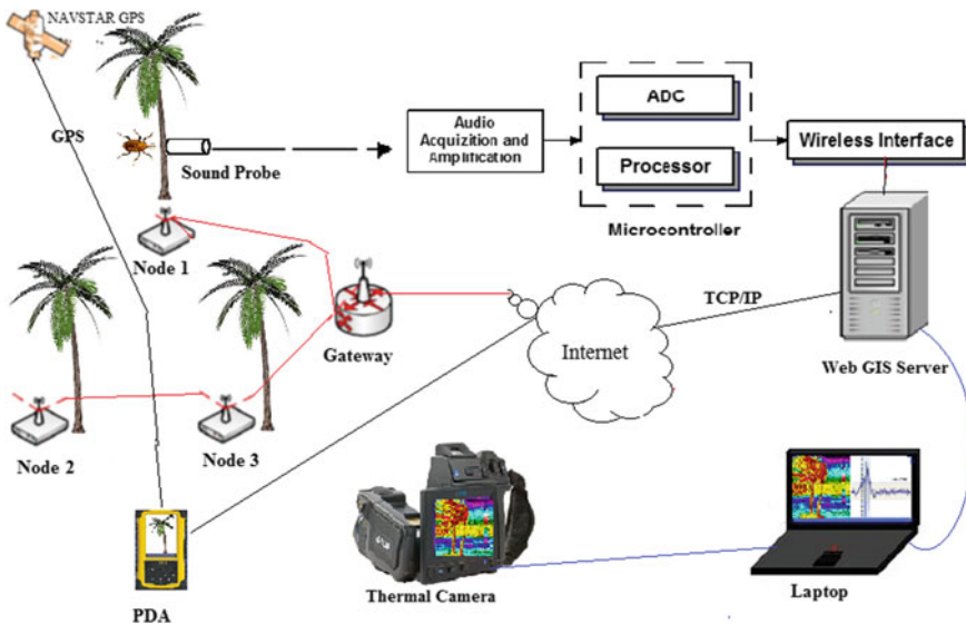
Fig. 3 A prototype block diagram for the proposed RPW detection system
