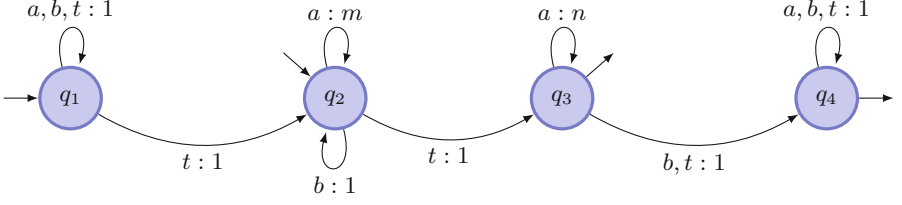
Fig. 1. Weighted automaton
