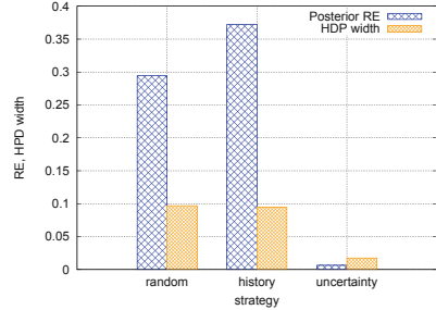
Fig. 5. Inference effectiveness.
