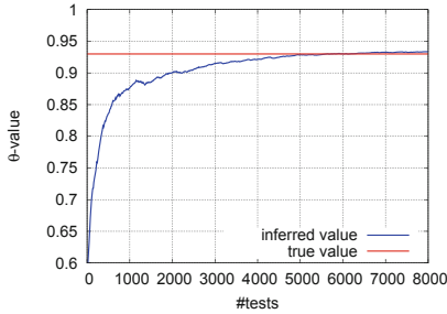
Fig. 4. Inference of a \theta parameter.
