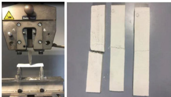
Fig. 2 Specimen for flexural strength test
