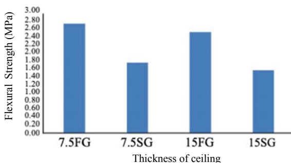
Fig. 3 Flexural strength of ceiling
