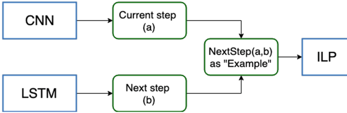
Fig. 1. A prototypical framework consisting of two components, i.e. (1) deep learning models – CNN and LSTM, and (2) ILP. In the framework, outputs of the deep learning models, instances of current and next step, are forwarded as relational predicates “Example” to an ILP system.
