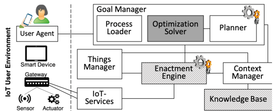
Fig. 1. Overview of our framework.
