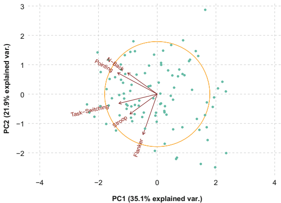
Fig. 9. Principal Component Analysis (PCA) of cognitive tests. (Color figure online)
