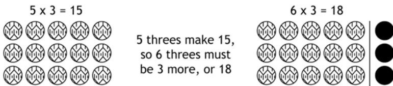
Fig. 3.6 Extending multiplication
