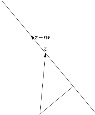
FIGURE 1. Proof of the Cauchy-Schwarz inequality
