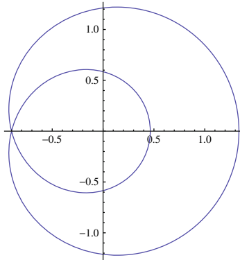
FIGURE 4. Overlapping image of unit disk
