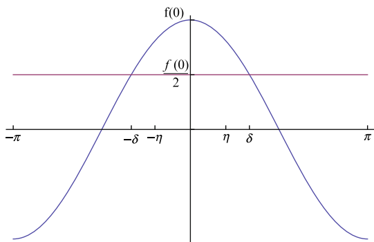
FIGURE 9. Proof of Theorem 1.12
