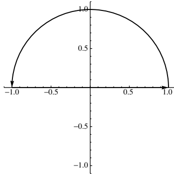
FIGURE 10. Contour used in second proof of Hilbert's inequality
