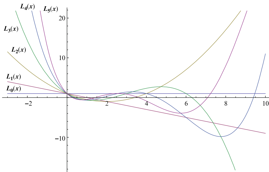
FIGURE 7. Laguerre polynomials
