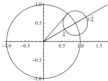
FIGURE 2. Reflection and perpendicularity
