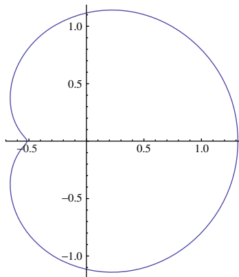
FIGURE 3. Injective image of unit disk
