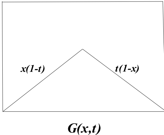
FIGURE 5. Green's function for the second derivative
