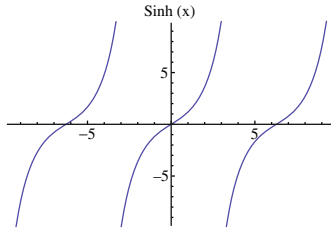
FIGURE 7. Periodic extension of hyperbolic sine
