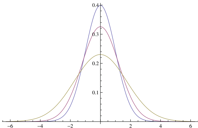
FIGURE 6. Gaussian kernel
