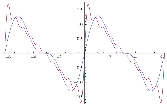
FIGURE 8. Approximations to the sawtooth function
