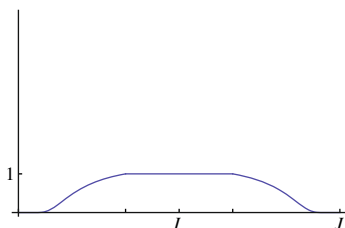
FIGURE 1. Cutoff Function
