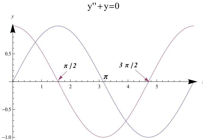
FIGURE 4. Sturm Separation
