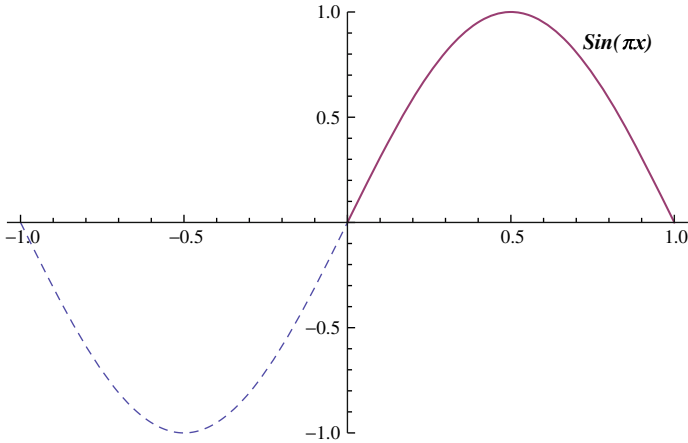
FIGURE 2. Wirtinger inequality
