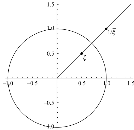
FIGURE 1. Reflection in the circle
