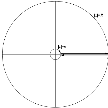
FIGURE 4. Contour used to evaluate C_p
