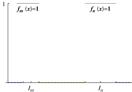
FIGURE 3. Example 1.3
