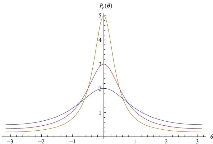
FIGURE 5. Poisson kernel
