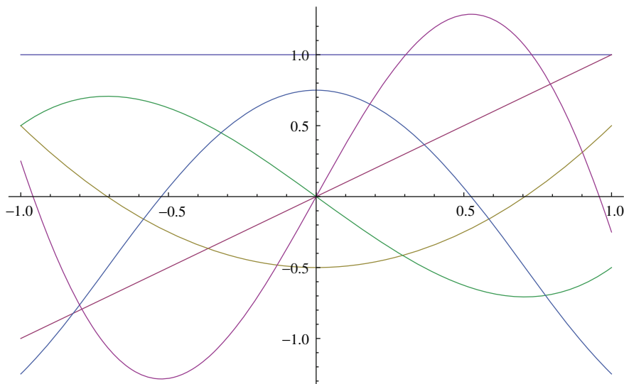
FIGURE 2. Scaled Hermite polynomials
