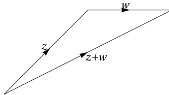
FIGURE 2. Triangle inequality
