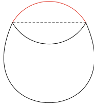
FIGURE 1. Convexity and the isoperimetric inequality
