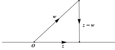
FIGURE 3. Orthogonal projection
