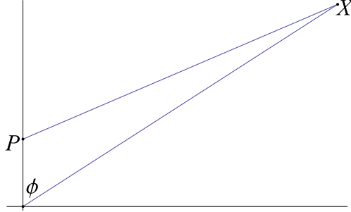
FIGURE 8. The co-latitude \phi
