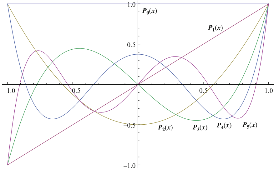
FIGURE 6. Legendre polynomials
