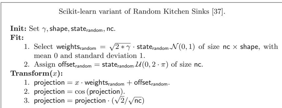
Fig. 2. RBF sampler.
