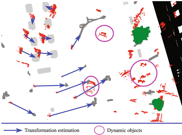
Fig. 5. Illustration of the output of the proposed object matching algorithm based on the fingerprint minutiae approach [14]. Red points mark the objects observed in the RMB Lidar frame. (Color figure online)
