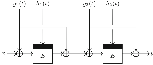
Fig. 1. Tweakable block cipher XHX2.
