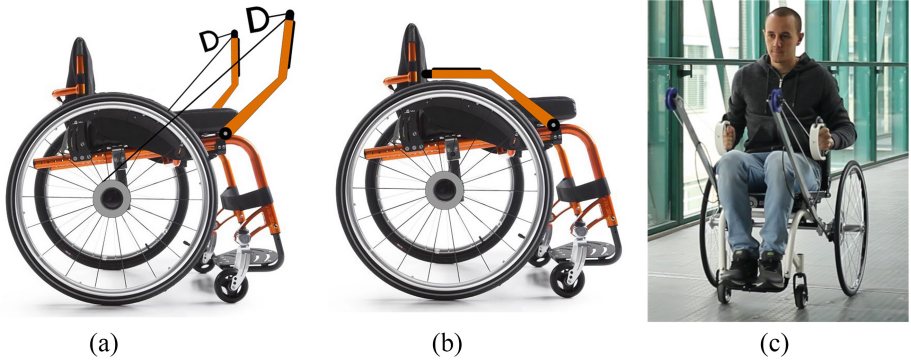
Fig. 8. Folding system of the cable traction system (a) and (b), Handwheelchair.q testing by one of the Authors (c)
