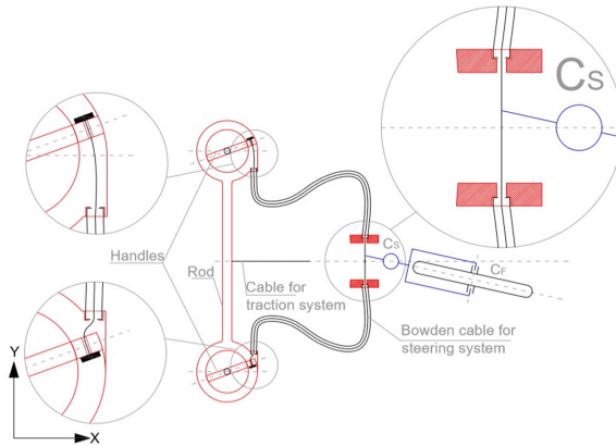
Fig. 10. Steering system
