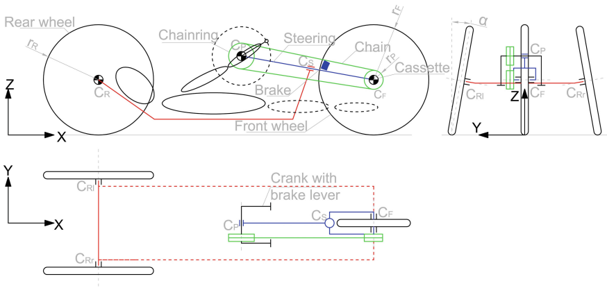
Fig. 3. Hand bike for categories H1–H4
