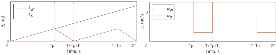
Fig. 6. Angular position and angular speed respectively of wheel (W) and pulley (P)
