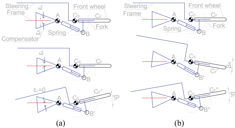
Fig. 2. Steering mechanism for race field (a) and for road race (b)
