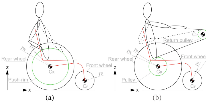
Fig. 7. User movement: Push-rim (a), Innovative (b)
