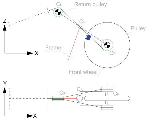
Fig. 12. Traction cable setup for Handbike.q
