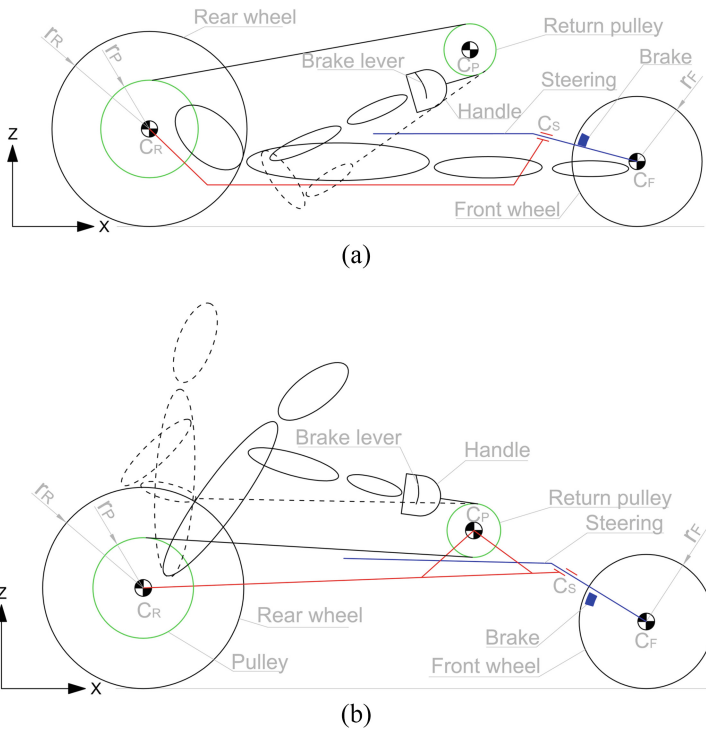
Fig. 9. Racing Handwheelchair.q for H1-H4 (a) and for H5 (b)
