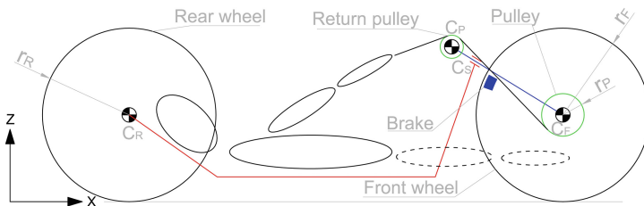
Fig. 11. Handbike.q for categories H1–H4
