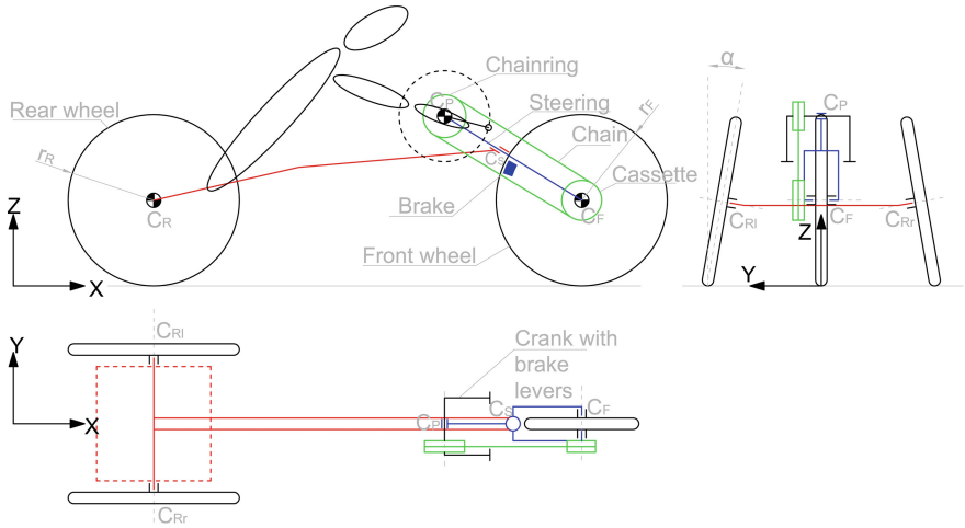
Fig. 4. Hand bike for categories H5
