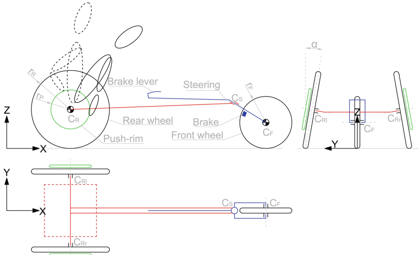
Fig. 1. Functional scheme of racing wheelchair
