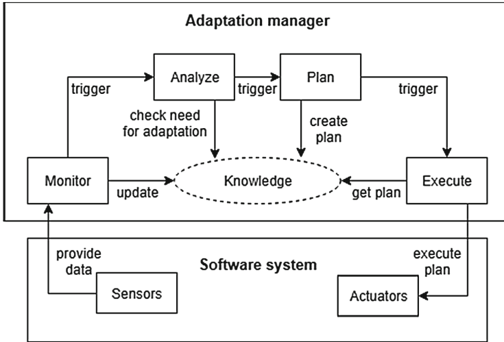
Fig. 1. The MAPE-K model [5].
