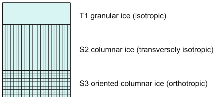
Fig. 2.1 Typical depth profile of first-year sea ice
