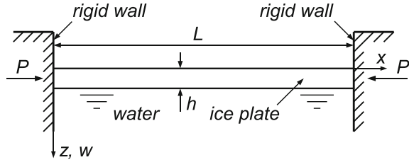
Fig. 4.14 Floating ice plate of thickness h and span L constrained by vertical rigid walls at its ends
