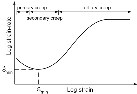
Fig. 3.8 Strain-rate dependence on strain during creep of polycrystalline ice under constant stress and temperature
