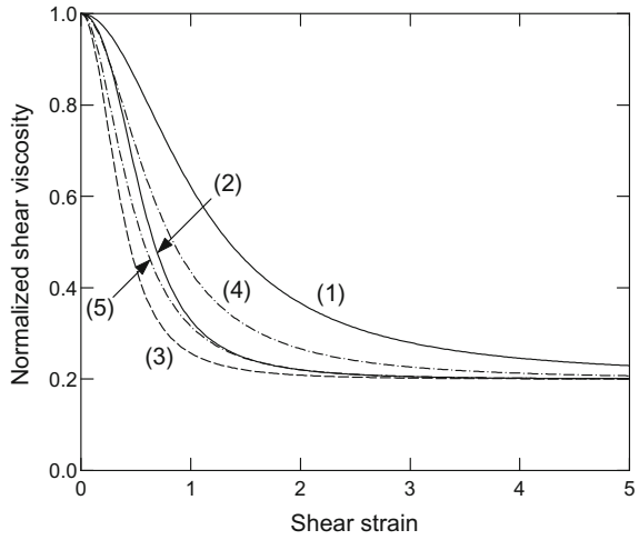
Fig. 7.11 Evolution of the normalized shear viscosity \mu_{13}/\mu_0 with the strain \kappa in simple shear started from an isotropic state ( \lambda_1 = \lambda_3 = 1 ) for different response functions \hat{f}(b_r) (cold ice)
