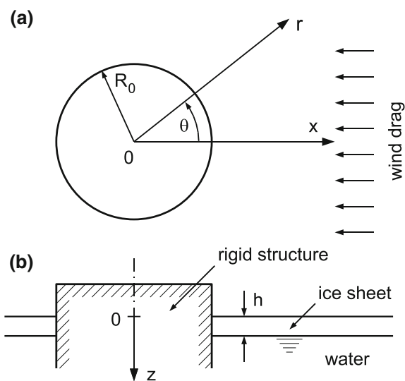
Fig. 4.24 Geometry of the problem and cylindrical polar coordinates: a plane view, b ice sheet cross-section
