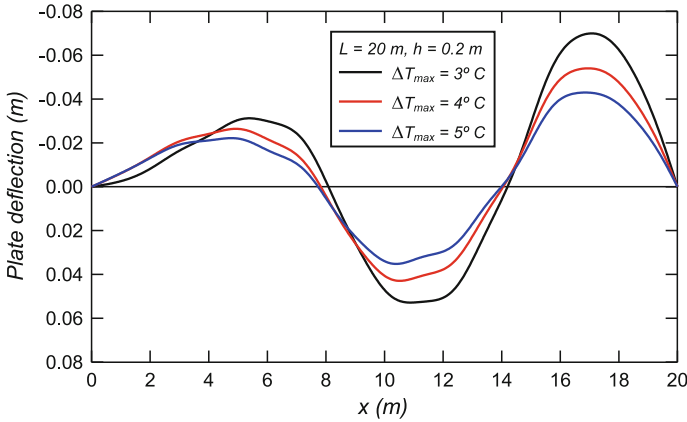
Fig. 4.18 Plate deflection curves w(x) at corresponding failure times t = t_f for different temperature amplitudes \Delta T_{max} , for the plate of thickness h = 0.2\text{ m} and span L = 20\text{ m} . Reprinted with permission from Staroszczyk (2018), Fig. 7. Copyright 2018 by Elsevier
