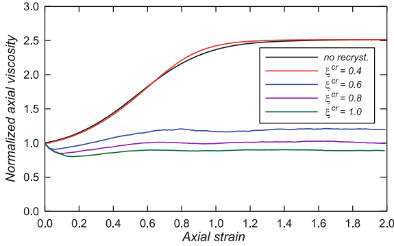
Fig. 6.23 Variation of the normalized macroscopic axial viscosity \mu_{33}/\mu_0 with the axial strain \varepsilon_{33} = \lambda_3 - 1 in uniaxial tension of recrystallizing ice, for different levels of the critical strain-rate invariant \xi_{eq}^{cr} = D_{eq}/\dot{D}_{eq} . Predictions of the SR-D model
