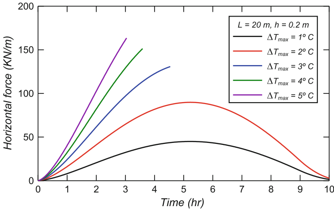
Fig. 4.19 Evolution of the horizontal force P(t) exerted by ice on the rigid walls for different values of the maximum temperature increase \Delta T_{max} , for the plate of thickness h = 0.2\text{ m} and span L = 20\text{ m} . Reprinted with permission from Staroszczyk (2018), Fig. 9. Copyright 2018 by Elsevier
