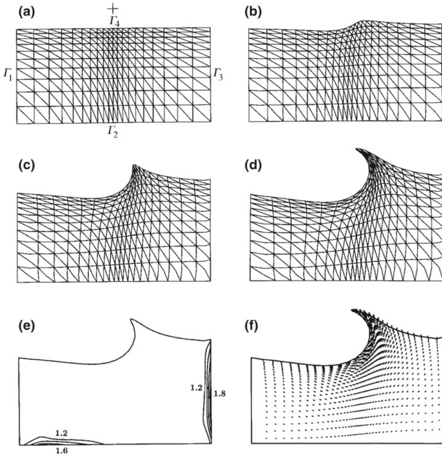
Fig. 5.9 Evolution of a rectangular ice pack driven by a geostrophic vortex wind, for the non-linearly viscous fluid rheology with a bounding envelope. Free-slip conditions are adopted at the solid boundaries \Gamma_1 , \Gamma_2 and \Gamma_3 . a Finite-element mesh at the start of simulation, with the cross representing the wind vortex centre; b , c and d the mesh after one, three and five days, respectively; e the ice thickness distribution after five days; f the ice velocity vector field after five days. Reprinted from Morland and Staroszczyk (1998), Fig. 10, with permission of the Royal Society of London
