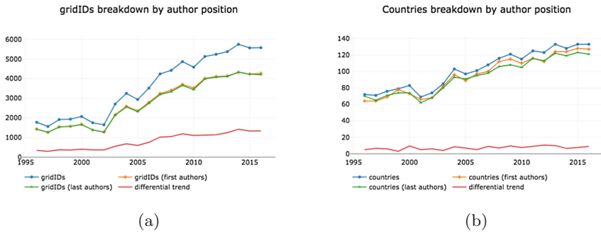
Fig. 2. Institutions and countries breakdown according to author position (Color figure online)
