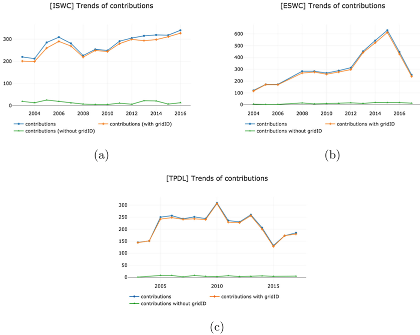
Fig. 4. Trends of contributions with and without resolved affiliations
