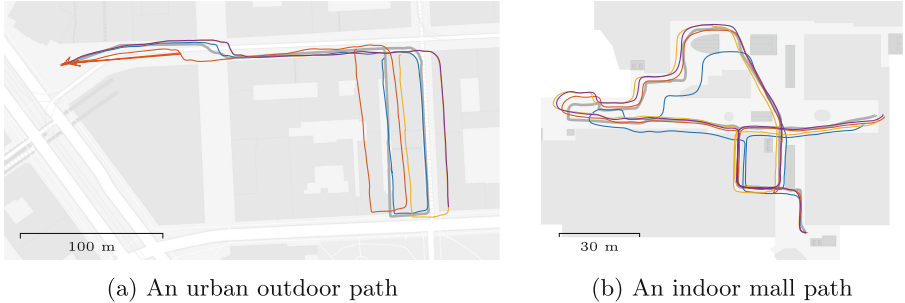
Fig. 6. Example paths showing ground-truth (—), ARKit (—), ARCore (—), Tango/Raw (—), and Tango/Area learning (—) that stopped prematurely in (a). Map data © OpenStreetMap. The ground-truth fix points were marked on an architectural drawing. ROVIO and PIVO diverge and are not shown.
