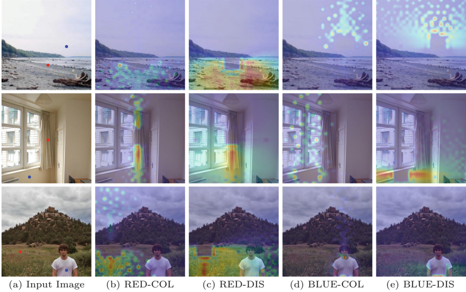
Fig. 6. Visualization of learned masks by PSANet. Masks are sensitive to location and category information that harvest different contextual information. (Color figure online)
