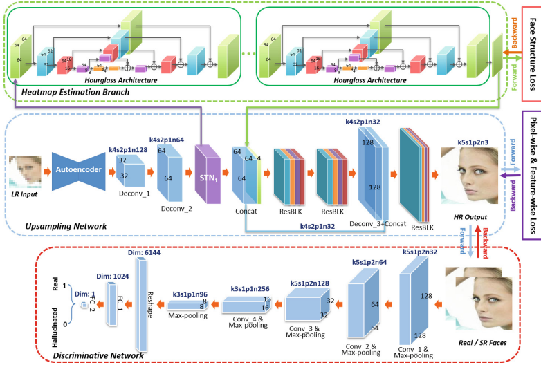
Fig. 2. The pipeline of our multi-task upsampling network. In the testing phase, the upsampling branch (blue block) and the heatmap estimation branch (green block) are used. (Color figure online)
