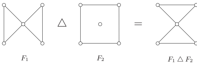
Fig. 2.4. The symmetric difference of two graphs
