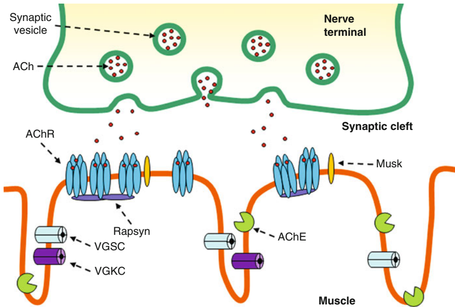
Fig. 1 The structure of the neuromuscular junction (NMJ) and the major components involved in neuromuscular transmission. The acetylcholine ( ACh )-containing vesicles are located at the nerve terminal allowing rapid release of ACh upon stimulation. The released ACh binds to the AChRs causing the opening of the ion channel, depolarization of the muscle membrane (EPSP), and subsequent activation of voltage-gated sodium channels ( VGSCs ) to initiate the action potential. Activation of the adjacent voltage-gated potassium channels ( VGKCs ) repolarizes the muscle membrane. Eventually, the ACh is hydrolyzed by acetylcholinesterase ( AChE ) and the signal is terminated. The muscle membrane has extensive folds with the AChRs densely packed at the top of the folds, via rapsyn. Muscle-specific kinase ( MuSK ) is a key player in agrin-induced AChR clustering and in the maintenance of NMJ structure
