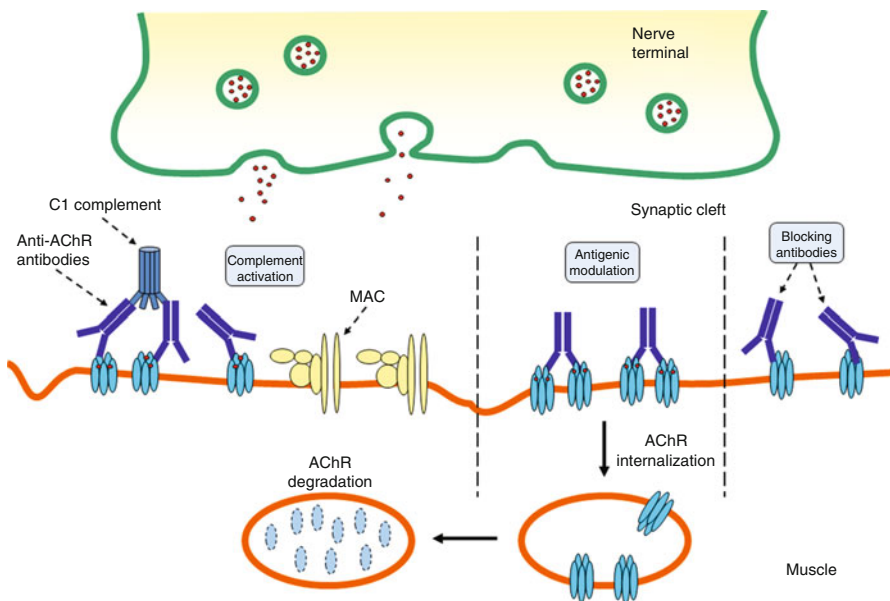
Fig. 3 The three major ways of anti-AChR action at the neuromuscular junction. Complement activation leads to the formation of membrane attack complexes (MACs) on the muscle membrane and destruction of the typical junctional folds ( left ); cross-linking of the acetylcholine receptors (AChRs) by the autoantibodies causes antigenic modulation, receptor internalization, and subsequent degradation ( center ); and blocking antibodies directly inhibit acetylcholine binding to its binding site on the AChRs ( right ). Notice the overall change of the characteristic morphology of the neuromuscular junction
