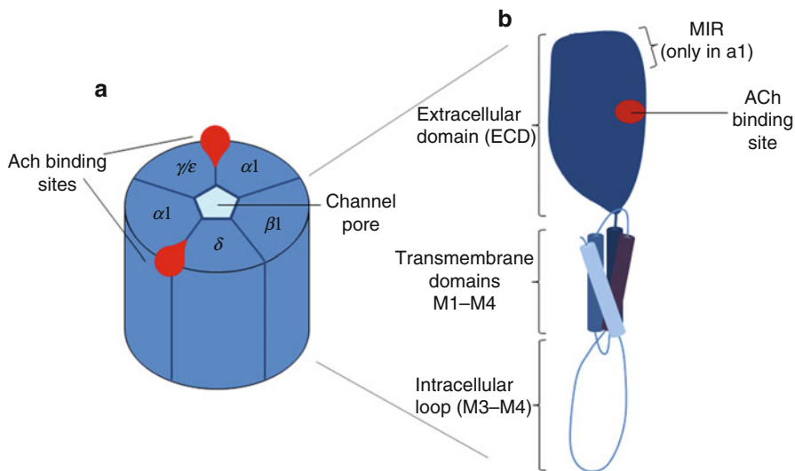
Fig. 2 The muscle nicotinic acetylcholine receptor (AChR). (a) The receptor is a transmembrane ion channel formed by five homologous subunits. Depending on whether the receptor is embryonic or adult, it contains a \gamma or \epsilon subunit, respectively. Each of the ligand binding sites is located at the interface between an \alpha 1 subunit and the \delta or \gamma/\epsilon subunits. Binding of acetylcholine ( ACh ) causes opening of the central pore allowing the passage of ions. (b) Longitudinal view of an AChR subunit, with its ECD, four transmembrane domains, and the large M3–M4 cytoplasmic loop. The location of the main immunogenic region (MIR – only present on the \alpha 1 subunit) and the ACh binding site is shown
