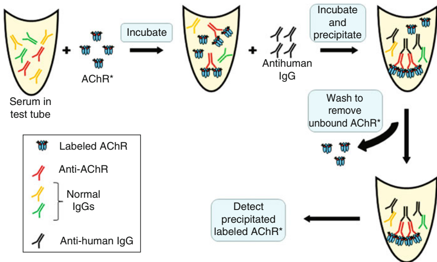
Fig. 4 Schematic representation of the RIPA assay for the detection of anti-AChR autoantibodies from MG patients' sera. The serum of each patient is mixed in a test tube with I^{125} -labeled human acetylcholine receptor (AChR*) and incubated to allow the anti-AChR antibodies to bind to the AChRs. Then antihuman IgG is added, and the whole complex is precipitated with centrifugation. The pellet is washed and measured for radioactivity, which is proportional to the precipitated AChRs and thus to the anti-AChR antibodies present in the serum
