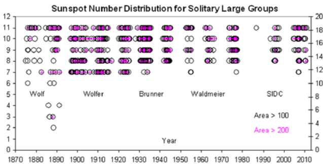
Fig. 33 For days where only one group was observed, the sunspot number (if less than 12) for that day (i.e. for that solitary group) is plotted if the projected area of the group is larger than 100 \mu\text{Hemisphere} (circles) and larger than 200 \mu\text{H} (pink “+” symbols). The right-hand scale is for sunspot number divided by 0.6, i.e. on the original Wolf scale
