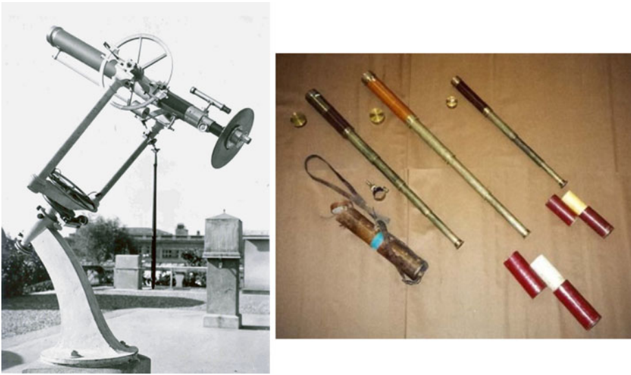
Fig. 5 The original instruments used by R. Wolf. On the left , the standard “4-foot” 80 mm Fraunhofer refractor, pictured here as it was set up at the Zürich Observatory (image source: Library of the ETH Zürich, Image Archive, http://www.e-pics.ethz.ch , Record N° Ans-05063-001). On the right , the three smaller portable refractors (apertures of 30 and 40 mm) used by Wolf while he was travelling
