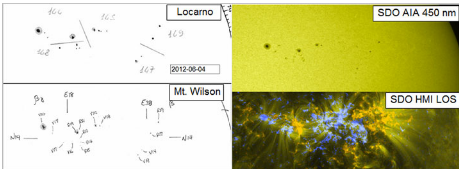
Fig. 46 Groups and spots observed 4th June 2012 at Locarno (five groups; upper left ), MWO (two groups; lower left with polarities indicated), SDO AIA at 450 nm ( upper right ), and their magnetic fields ( blue positive, orange negative; lower right ). The two MWO groups are marked by the latitudes and longitudes of the centroids (N14, E18 and N14, E38)
