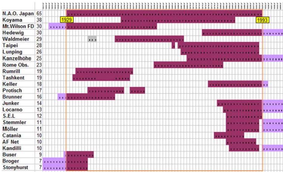
Fig. 25 Coverage and observers for the Koyama Backbone (1921–2000)
