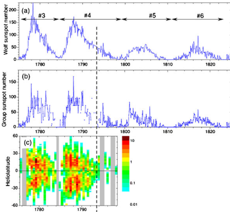
Fig. 15 Sunspot activity in the late 18th and early 19th century: (a) Monthly mean Wolf SN. (b) Monthly mean GN. (c) Reconstructed sunspot butterfly diagram. The color scale on the right gives the density (in \text{year}^{-1} \text{deg}^{-1} ) of sunspots in latitude-time bins and gray bars indicate that no latitudinal information is available. Each bin covers 2^\circ in latitude and six months in time. The vertical dashed line marks the start of the “lost” cycle, late in 1793 (from Usoskin et al. 2009)
