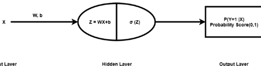
Figure 4-5. Chart of logistic regression model
