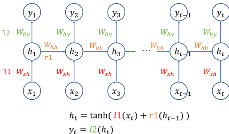
Figure 9-1. An RNN
