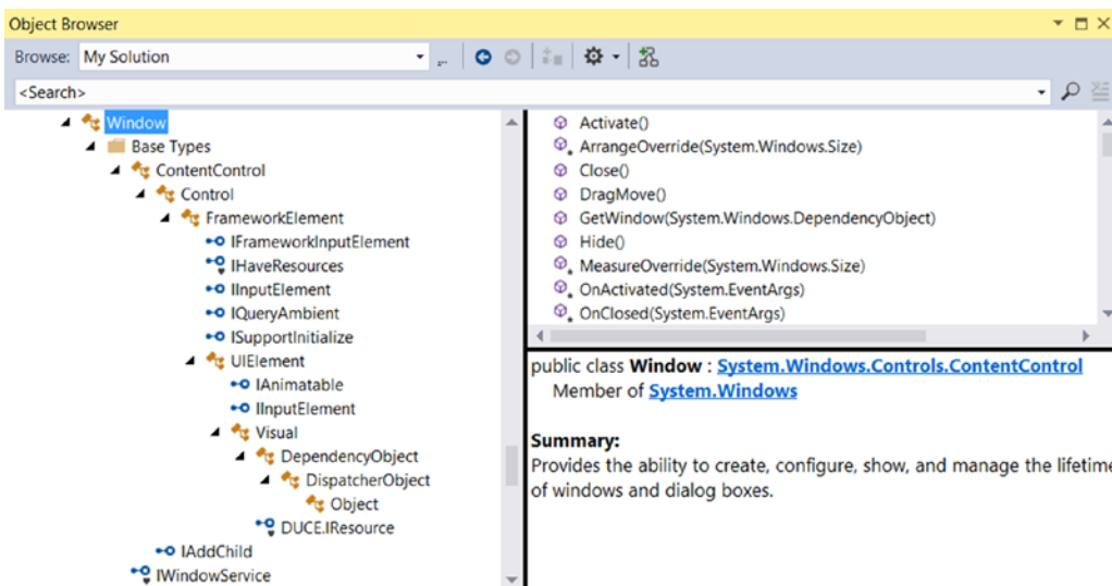
Figure 26-5. The hierarchy of the Window class
