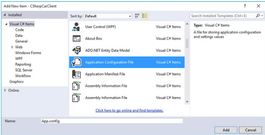
Figure 14-11. Inserting a new XML configuration file
