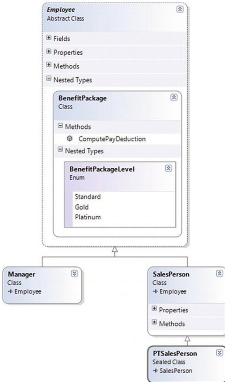
Figure 6-6. The Employee hierarchy
