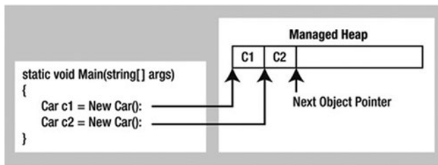
Figure 13-2. The details of allocating objects onto the managed heap
