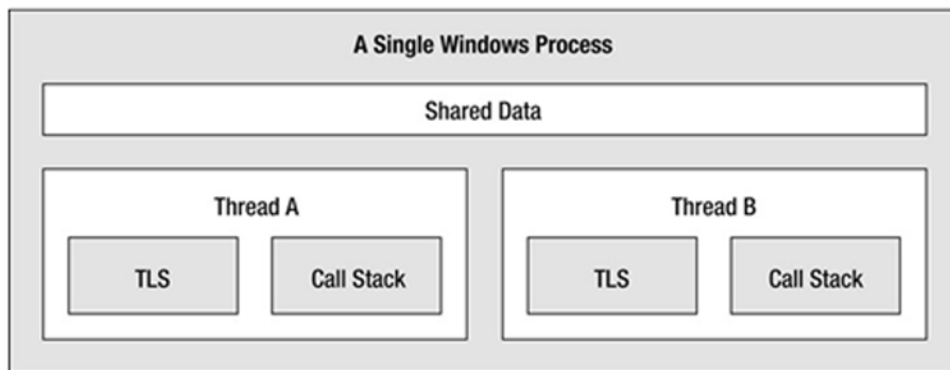
Figure 17-2. The Windows process/thread relationship
