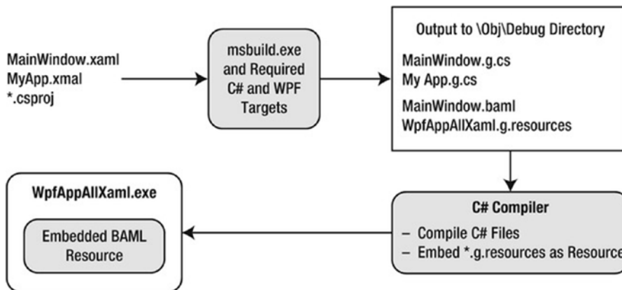
Figure 26-11. The XAML-to-assembly compile-time process
