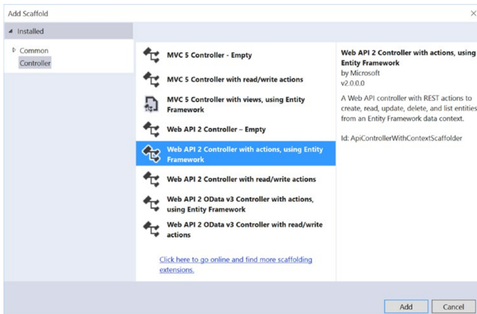
Figure 34-33. Adding a new Web API 2 Controller
