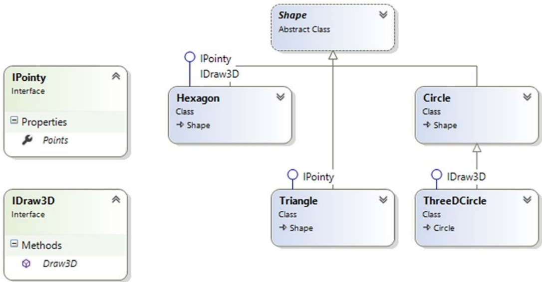
Figure 8-3. The updated shapes hierarchy
