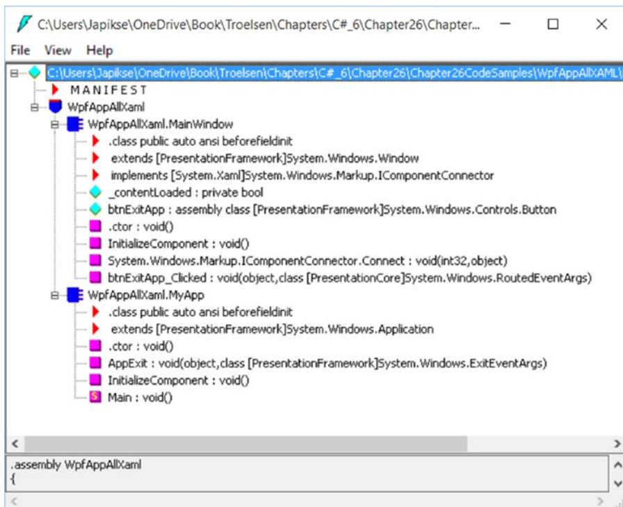
Figure 26-9. Transforming XAML into a .NET executable? Interesting . . .
