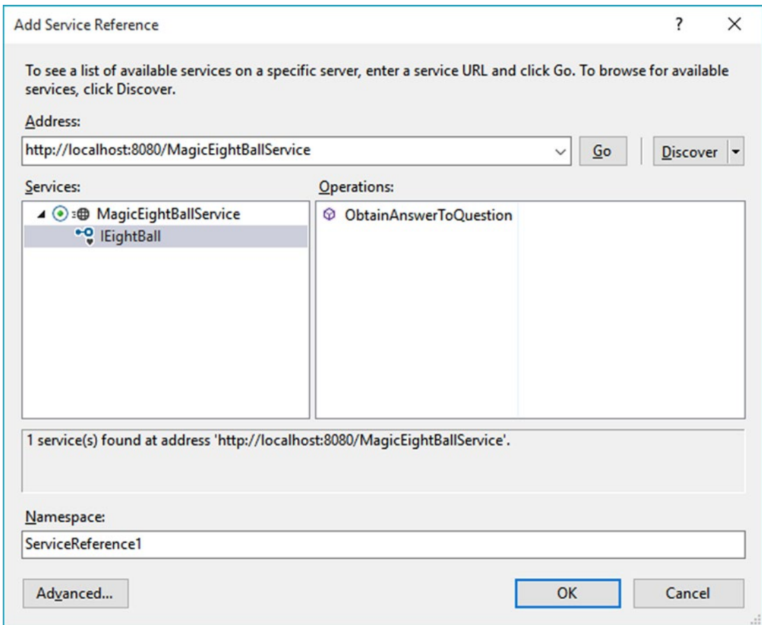
Figure 25-7. Generating the proxy files using Visual Studio
