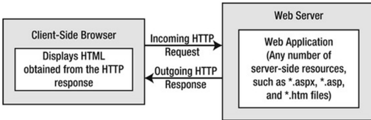
Figure 31-1. The HTTP request/response cycle
