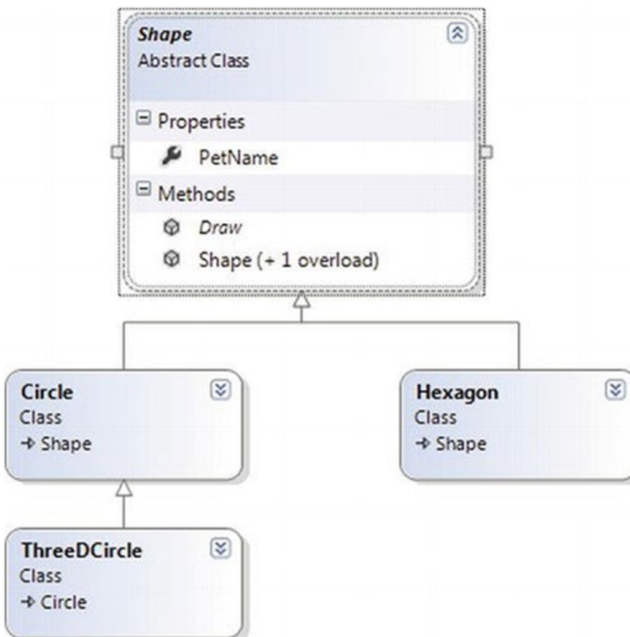
Figure 6-7. The shapes hierarchy
