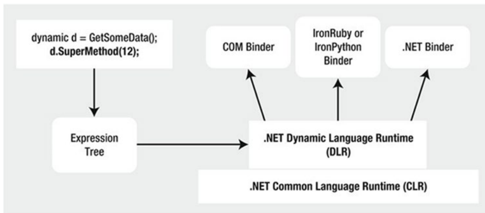
Figure 16-2. Expression trees capture dynamic calls in neutral terms and are processed by binders
