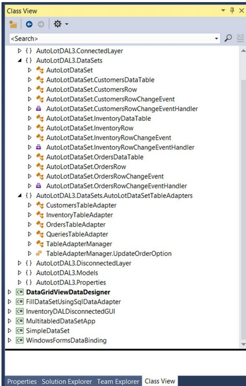
Figure 22-27. The autogenerated strongly typed data of the AutoLot database
