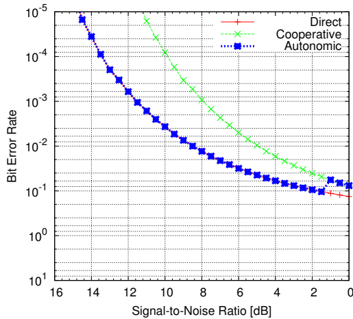
Fig. 5.11 Autonomic reaction at the threshold of BER = 0.100
