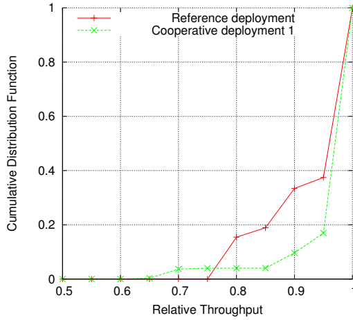
Fig. 6.8 CDF for scenario No 1
