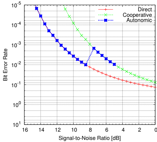
Fig. 5.10 Autonomic reaction at the threshold of BER = 0.010
