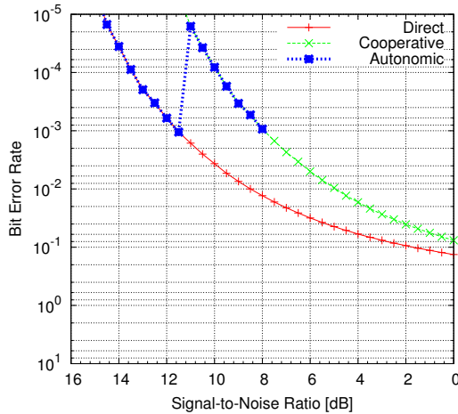
Fig. 5.9 Autonomic reaction at the threshold of BER = 0.001
