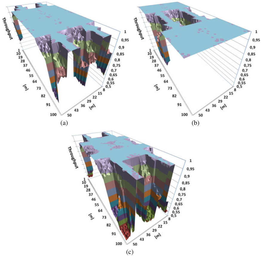
Fig. 7.8 Relative throughput for: (a) Deployment A, (b) Deployment B, (c) Deployment C
