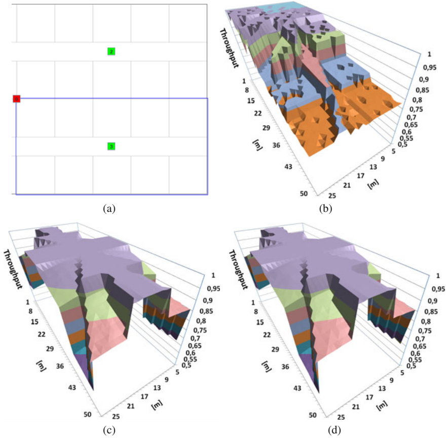
Fig. 6.3 Deployment of FRNs (a) and relative user throughput for direct transmission (b), single path relaying via FRN3 (c) and FRN2-FRN3 cooperation (d)
