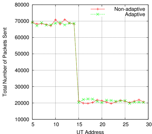
Fig. 3.9 Total number of packets sent for buffer length equal to 60
