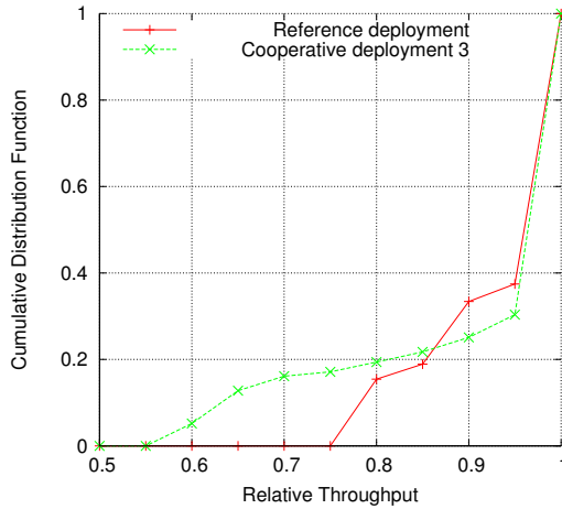
Fig. 6.10 CDF for scenario No 3
