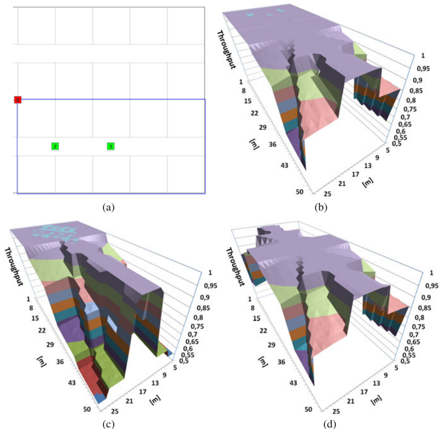
Fig. 6.4 Deployment of FRNs (a) and relative user throughput for FRN2-FRN3 cooperation (b), single path relaying via FRN2 (c) and single path relaying via FRN3 (d)
