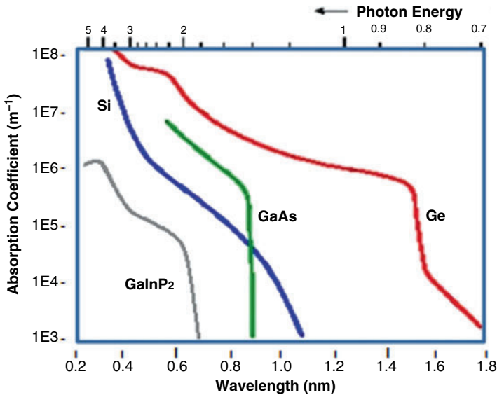
Fig. 7.18 Absorption coefficient spectra of GaInP 2 , GaAs, Ge, and Si
