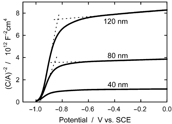
Fig. 3.14 Mott–Schottky curves for 40, 80, and 120 nm dense anatase \text{TiO}_2 films on ITO, made by electron beam evaporation of \text{TiO}_{2-x} . The curves are recorded at a modulation frequency of 10 kHz and an amplitude of 5 mV, using a scan rate of 1 mV/s. The electrolyte was a 0.5 M KOH solution (pH 13.7). The electrode surface area is 7.0 \text{ mm}^2 for all three samples, and the capacitance values are normalized with respect to surface area. Reproduced from ref. [50] with permission from The Electrochemical Society
