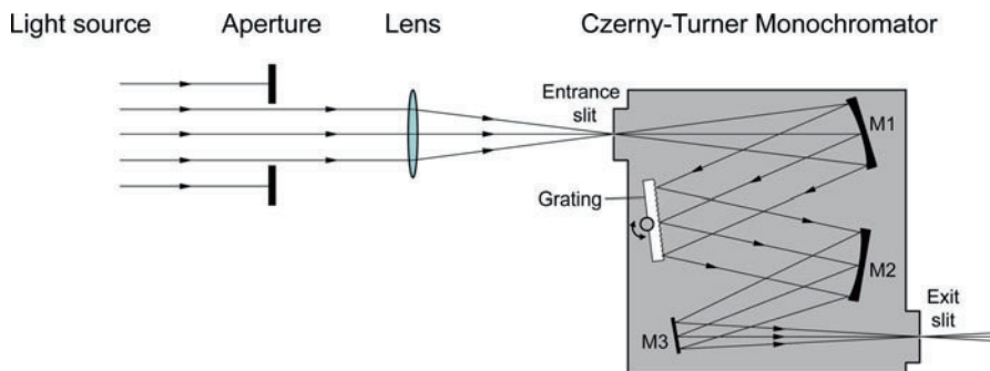
Fig. 3.8 Schematic diagram of a Czerny–Turner monochromator illuminated by a focused beam of light. The diffraction grating consists of a highly reflecting planar surface in which sawtooth-shaped grooves are etched. Mirrors M1 and M2 are concave-shaped, mirror M3 is a planar mirror that directs the light to the exit slit. The aperture in front of the lens prevents overfilling of the mirror, which would result in stray light inside the monochromator
