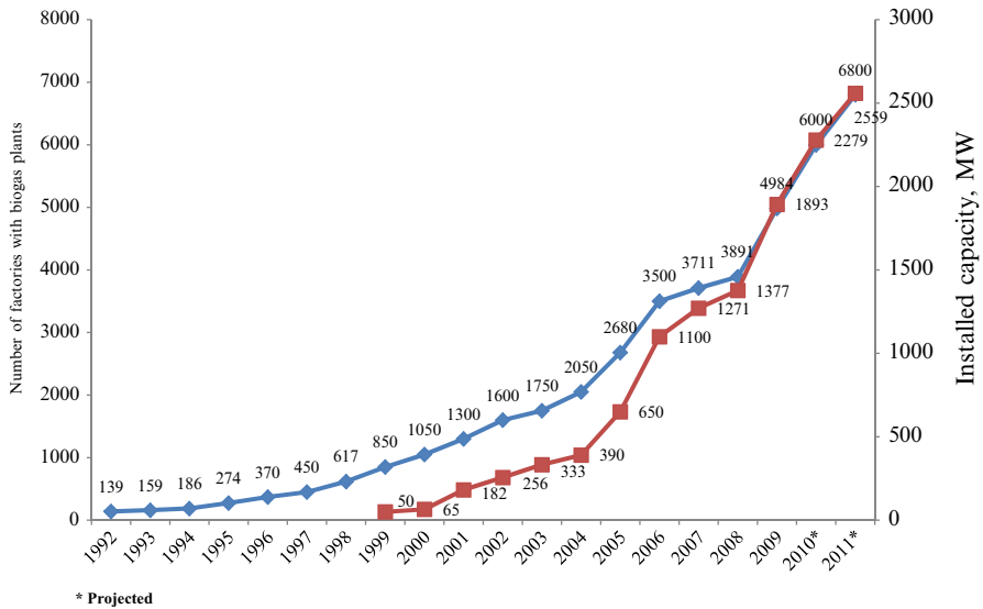
Fig. 2.6 Biogas plants in Germany (dx) and the rise in biogas-based power generation (dx) (adopted from Stolpp 2010)
