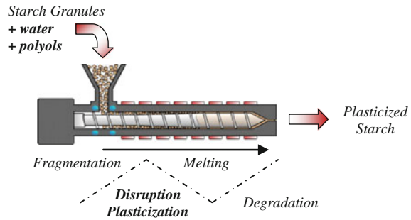
Fig. 2.4 Schematic representation of the starch extrusion process
