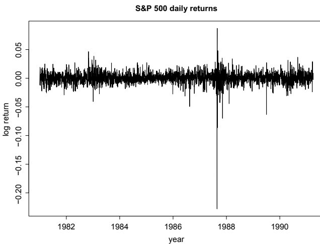
Fig. 4.1. Daily log returns on the S&P 500 index from January 1981 to April 1991. This data set is the variable r500 in the SP500 series in the Ecdat package in R. Notice the extreme volatility in October 1987.
