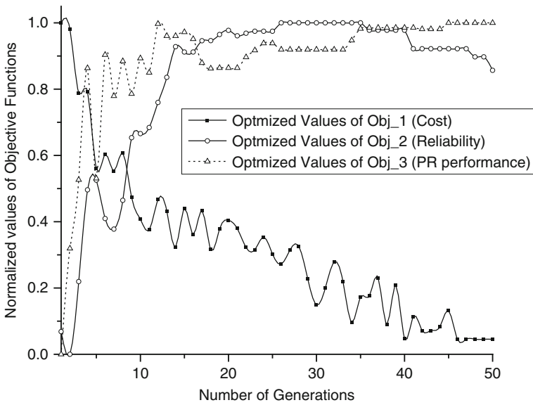
Fig. 17.11 Average optimized values of different objective functions in the first front of MOGA-IC with NSGA-II for 50 generations
