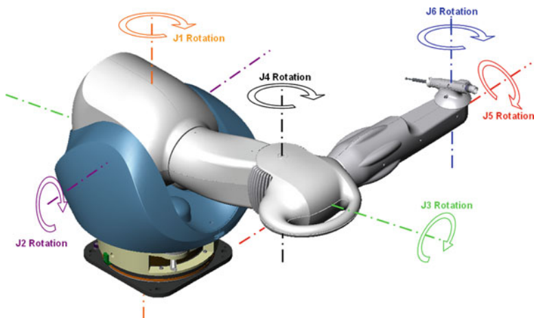
Fig. 10.5 Joint motion definitions of the RIO ® robotic arm
