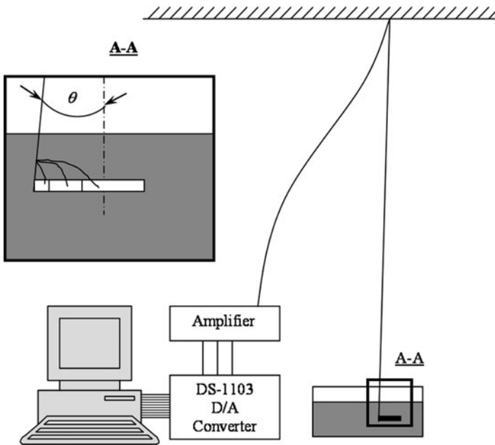
Fig. 16.7 Illustration of the experimental system (Copyright 2007 IEEE.)
