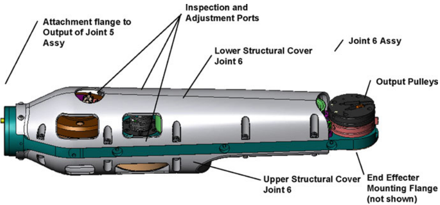
Fig. 10.7 Joint 6 arm assembly
