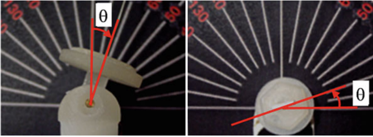
Fig. 14.28 Experimental setup for the angle measurement ( Left : bending angle, Right : rotation angle) (© 2009 IEEE), reprinted with permission [48]
