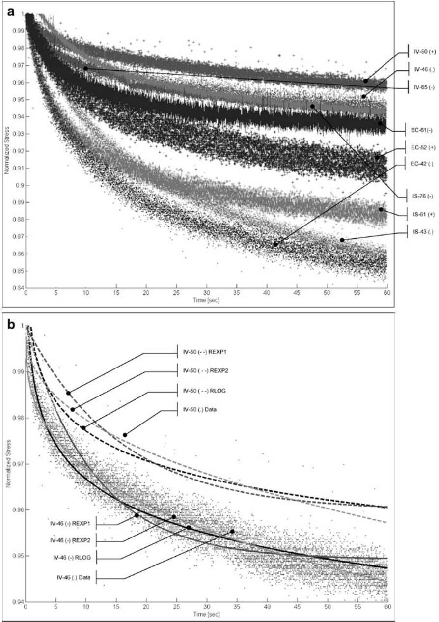
Fig. 24.6 Normalized stress-relaxation curves as a function of time for one liver tested with the MEG: (a) three different testing conditions ( IV in-vivo, IS in-situ, EC ex-corpus) and strain levels (indicated in the legends as a two-digit numeral [% strain]); (b) measured data and phenomenological models of two strain levels. Their measures of fit: 46% strain [REXP1 ( R^2 = 0.8948 , RMSE = 0.0042 ), REXP2 ( R^2 = 0.9261 , RMSE = 0.0030 ), RLOG ( R^2 = 0.9084 , RMSE = 0.0034 )], and strain 50% [REXP1 ( R^2 = 0.9387 , RMSE = 0.0026 ), REXP2 ( R^2 = 0.9526 , RMSE = 0.0021 ), RLOG ( R^2 = 0.9140 , RMSE = 0.0028 )]
