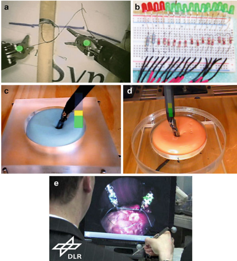
Fig. 18.11 (a) Small dots augmented over the surgeon's visual workspace display forces during a suturing task [29]. (b) External LED array displaying force levels [34], ©IEEE 2007. (c) Bar graph overlaid on visual workspace to display estimated forces during an exploration task [24], ©IEEE 2008. (d) Bar graph is aligned with da Vinci tool shaft and tracks its motion with proper disparity and depth perception, while displaying estimated forces [12], ©IEEE 2009. (e) 3D colored arrows indicated the force vector applied by the surgical instrument (courtesy DLR, see [37] for details)
