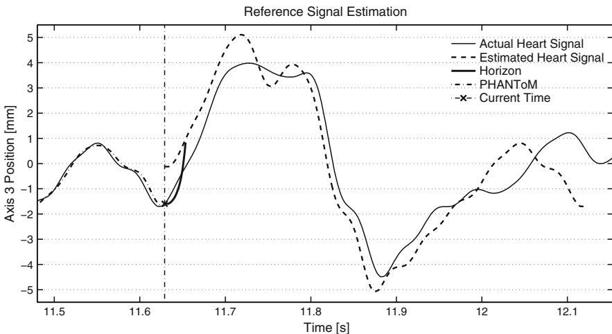
Fig. 22.4 Reference Signal Estimation during control action. Observe the horizon signal where the offset between the current position and estimated signal is added gradually starting from current time to horizon steps ahead (© IEEE 2007), reprinted with permission
