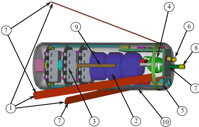
Fig. 16.2 Conceptual assembly drawing of a swimming micro robot for neurosurgery. The components of the robot are: (1) Three swimming tails, (2) Power source (here 3 Renata ZA10 batteries in series), (3) Packaged IC for command control and communication, (4) Antenna, (5) Endoscopic Camera, (6) LEDs, (7) Force sensors, (8) Tool for intervention, (9) Localization sensor (here an Aurora magnetic tracker receiving coil), (10) Casing (Transparent in the drawing to show the internal components) (Copyright 2008 IEEE)
