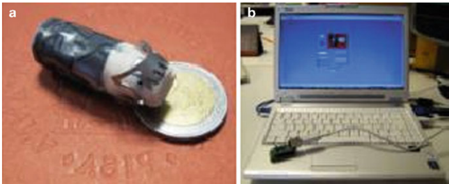
Fig. 14.19 (a) A picture of the clipping capsule having the OTSC clip loaded. (b) HMI and USB transceiver ( bottom left corner ) allowing wireless communication with the capsule (© 2008 Georg Thieme Verlag KG), reprinted with permission [24]
