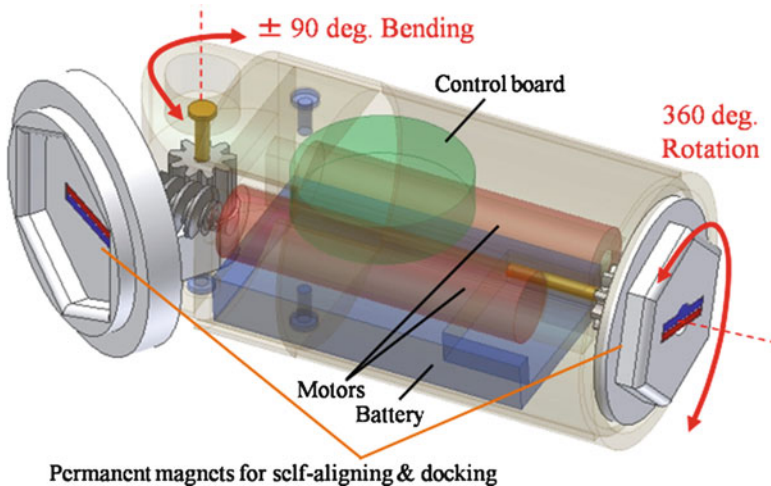
Fig. 14.24 Design of the structural module (© 2009 IEEE), reprinted with permission [48]
