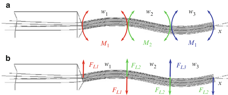
Fig. 16.4 A three section swimming tail with actuators that apply: (a) torques M_i or (b) forces F_{Li}
