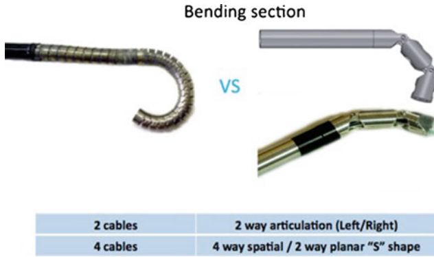
Fig. 30.6 Illustrating the bendable design of the robot scope
