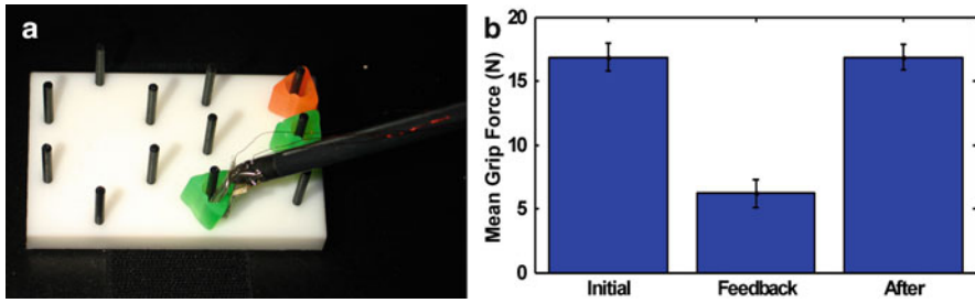
Fig. 19.5 (a) Single-hand peg transfer task showing grasping and transfer of a rubber piece using the da Vinci robotic system. (b) The mean grip forces exerted by an expert subject during each block of the peg transfer test. Error bars indicate standard error of the mean. (© 2009 IEEE), reprinted with permission
