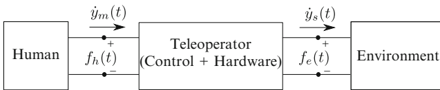
Fig. 18.6 The human and environment may be modeled as one-port terminations on the two-port teleoperator network model
