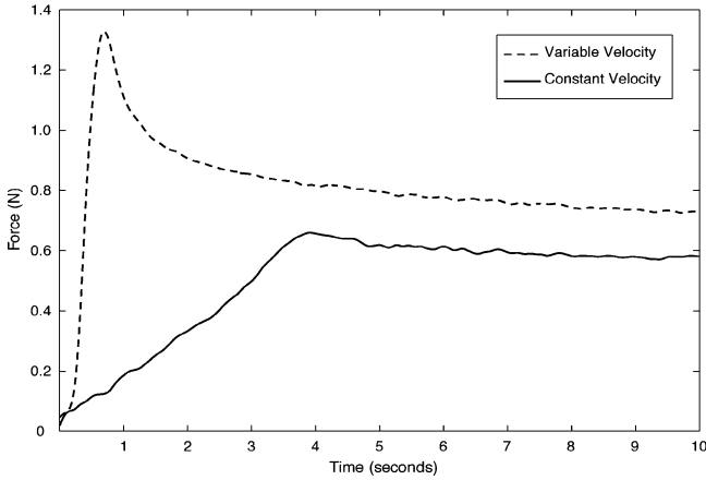
Fig. 20.3 Sample force response of variable-velocity and constant-velocity palpation to a depth of 9 mm
