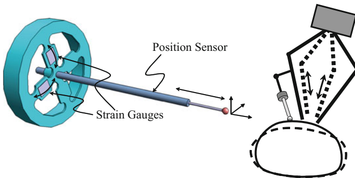
Fig. 22.9 Whisker Sensor Design 2. Left: One linear position sensor and a cross ( × ) shaped flexible structure with strain gauges are used to measure the three-dimensional position of the sensor tip. Right: Sensor is attached to the robot arm to measure the displacement between the heart and the surgical tools (© IEEE 2008), reprinted with permission
