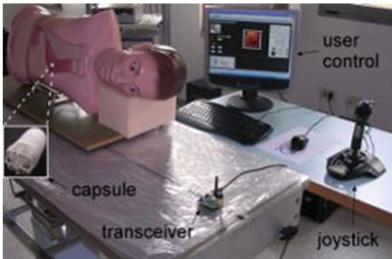
Fig. 14.10 The external unit of the system and the endoscopic capsule located in a upper torso simulator (© 2009 Taylor & Francis) [15]
