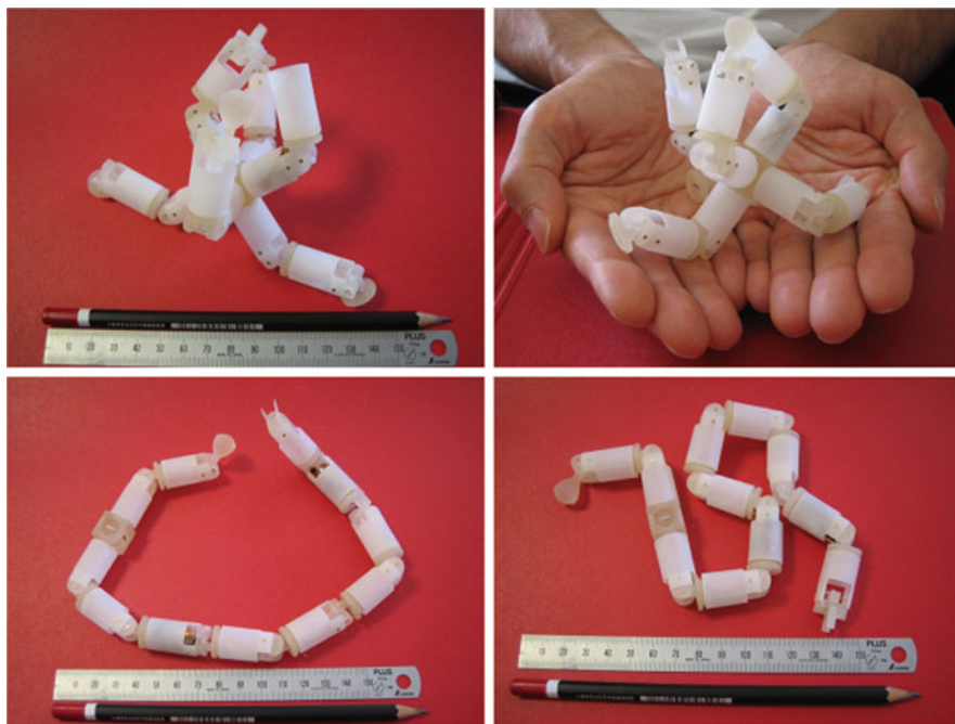
Fig. 14.27 Assembled modules and possible topologies (© 2009 IEEE), reprinted with permission [48]
