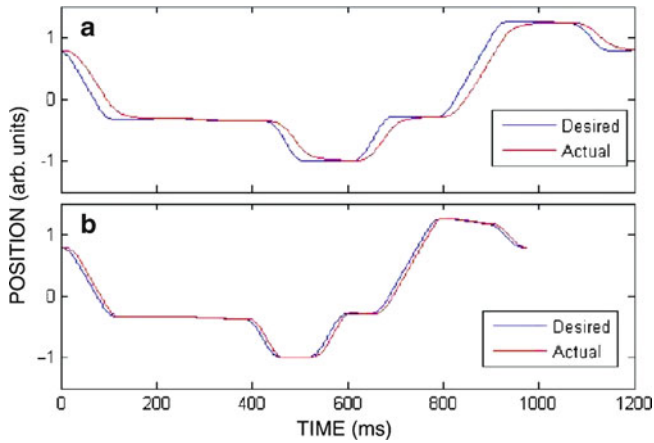
Fig. 3.13 SNS Joint-2 position versus time. (a) without a compensation filter; (b) with a compensation filter
