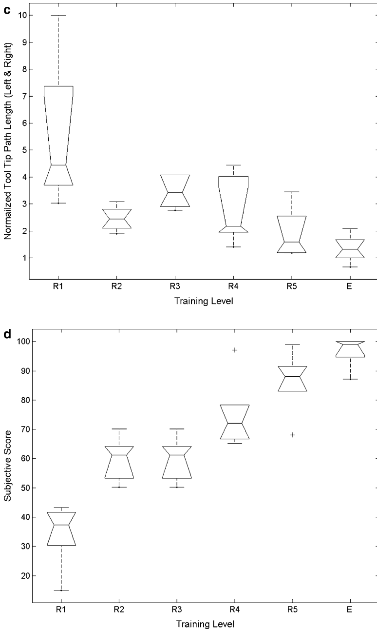
Fig. 25.8 (continued) (c) normalized path length of the two tool tips. The average task completion time of the expert group is 98 s and the total path length of the two tools is 3.832 m. The subjective performance index is based on visual scoring by an expert surgeon normalized with respect to experts' performance (d)
