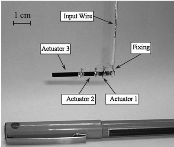
Fig. 16.6 The up-scaled swimming tail (Copyright 2007 IEEE.)
