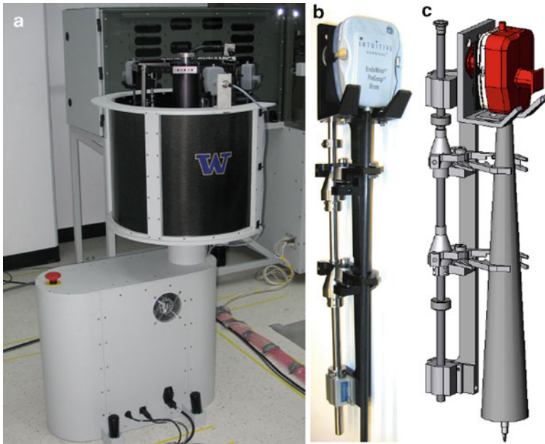
Fig. 3.16 Tool rack subsystem (a) overview; (b) tool holder grasping a surgical tool; (c) CAD display of tool holder grasping a surgical tool under permissible angular misalignment
