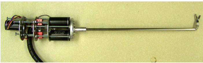
Fig. 7.9 Complete surgical instrument
