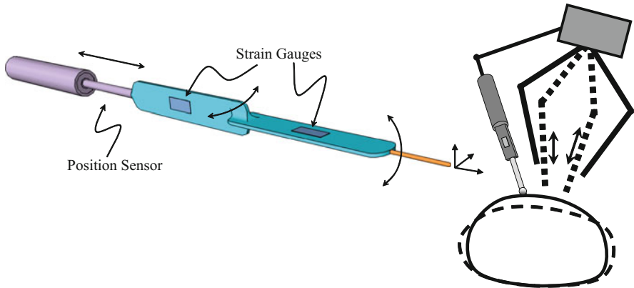
Fig. 22.8 Whisker Sensor Design 1. Left: One linear position sensor and two orthogonally placed flexure beams with strain gauges are used to measure the three-dimensional position of the sensor tip. Right: Sensor is attached to the manipulator base to provide continuous contact even when the surgical tools are not in close proximity, and to measure the heart position (© IEEE 2008), reprinted with permission
