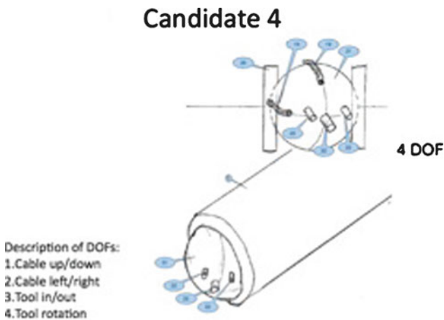
Fig. 30.11 Mechanism of “wire and sphere” movements and description of the degrees of freedom
