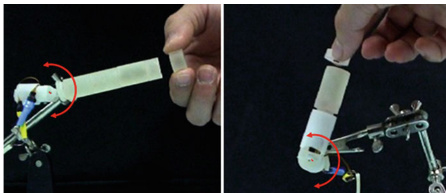
Fig. 14.31 Torque measurement ( Left: bending, Right: rotation ) (© 2009 IEEE), reprinted with permission [48]
