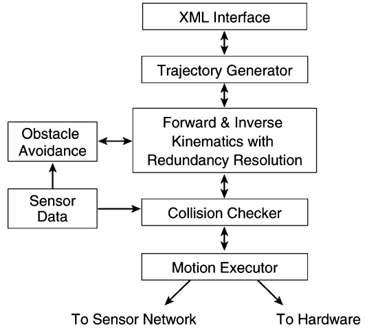
Fig. 3.12 Scrub nurse subsystem motion planner
