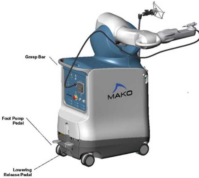
Fig. 10.9 Robotic arm assembly
