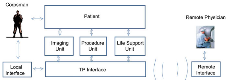
Fig. 3.25 TP-2 high level architecture
