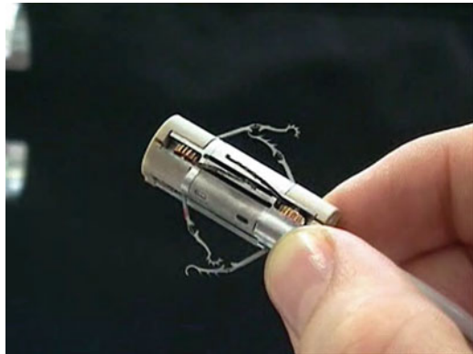
Fig. 14.3 A picture of the complete legged capsule integrating the legs
