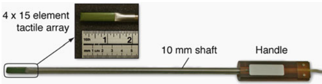
Fig. 20.4 The Tactile Sensing Instrument (TSI)
