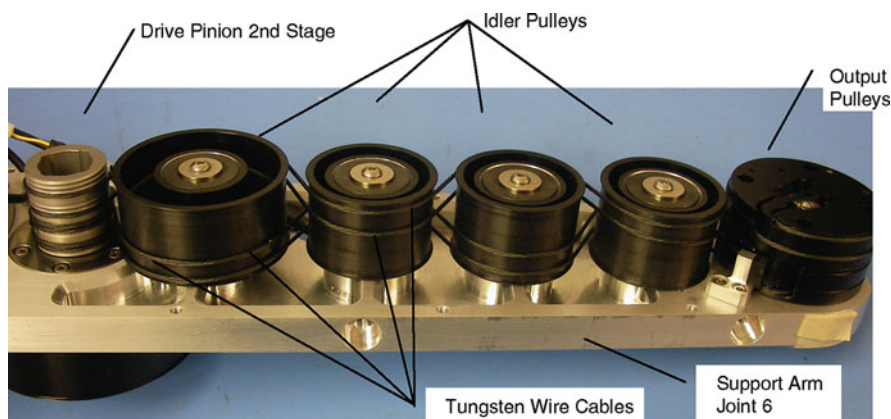
Fig. 10.6 Joint 6 assembly second stage cable drive
