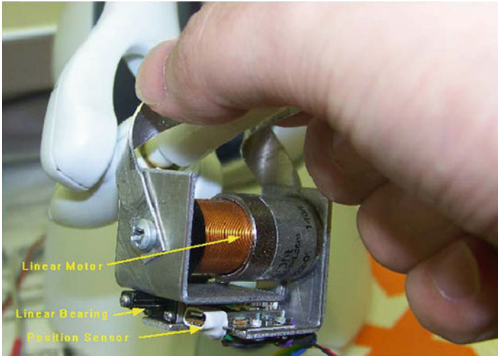
Fig. 7.11 Grip force feedback actuator assembly in teleoperation handle
