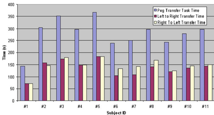
Fig. 7.18 Manual and teleoperated peg transfer task completion times
