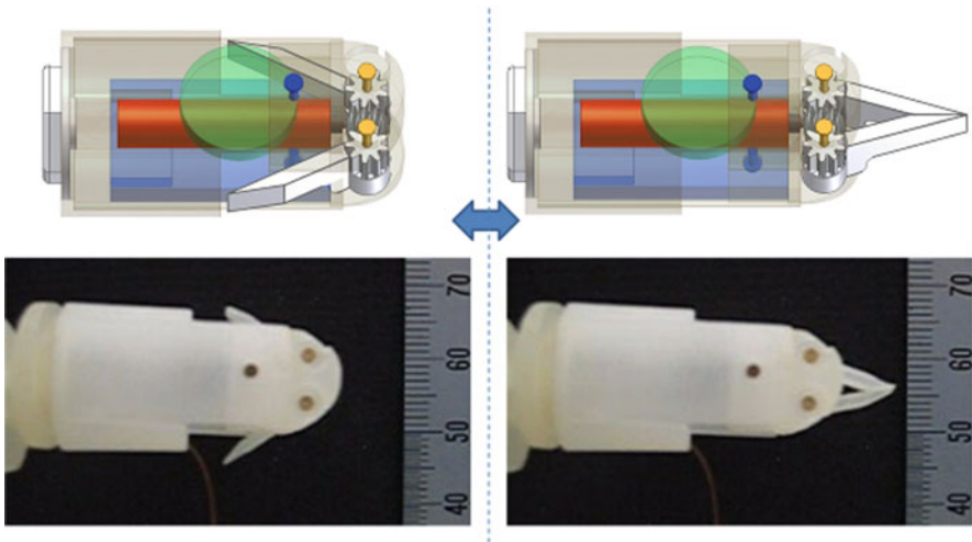
Fig. 14.26 Design and prototype of the biopsy module ( Left : for ingestion, Right : for operation) (© 2009 IEEE), reprinted with permission [48]
