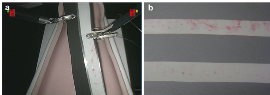
Fig. 19.4 (a) Grasping of the tissue phantom with the da Vinci robotic system. The left grasper passed the neoprene phantom; the right grasper (with mounted sensors) passed the neoprene phantom with attached pressure-indicating film. Marks appeared on the film at grasping locations; color intensity of the marks was proportional to the grasping force. (b) Pressure-indicating film resulting from a grasping trial without tactile feedback ( top ) and with tactile feedback ( bottom ). These results indicate that less force was applied to the film with tactile feedback. (© 2008 IEEE), reprinted with permission
