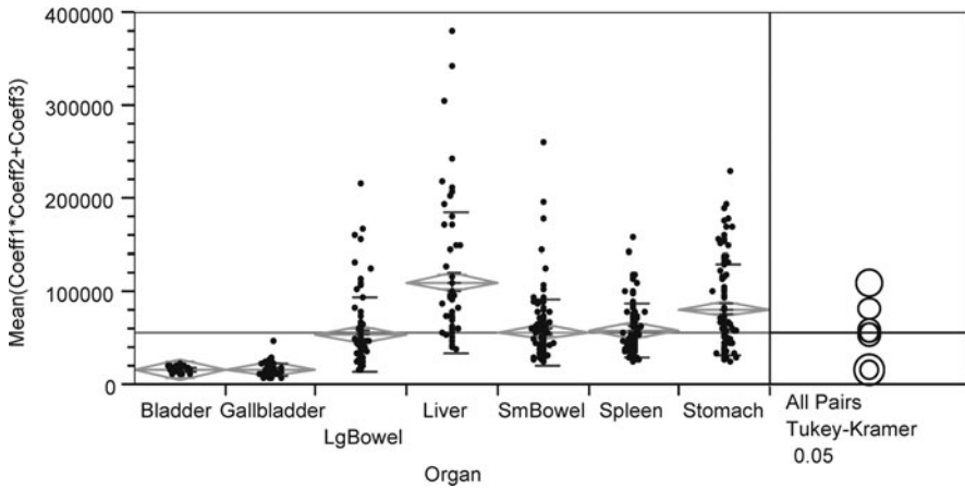
Fig. 24.9 The stiffness indicator scalar b \times a + g of the EXP2 phenomenological model plotted for various organs for measured elastic data. The right-hand side of the plot depicts the results from post hoc Tukey-Kramer HSD analysis. The radius of the circle represents the region of confidence (95%)
