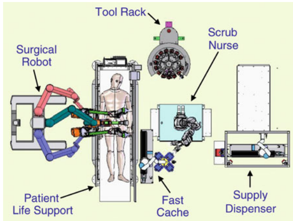
Fig. 3.6 Layout of trauma pod main components
