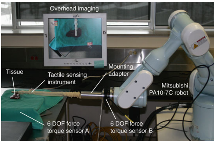
Fig. 20.5 Robotic experimental setup for tissue palpation with the TSI
