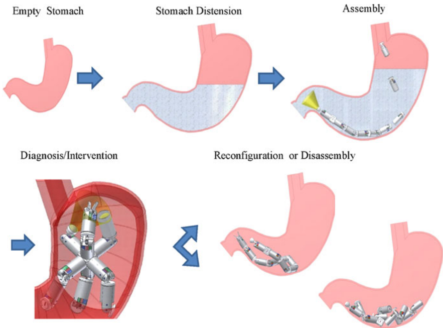
Fig. 14.23 Procedures for the multi-capsule surgical robotic system
