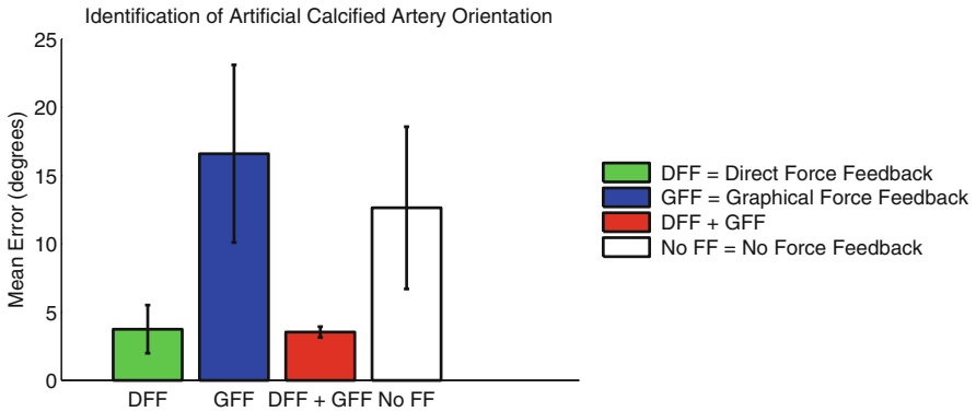
Fig. 18.13 Palpation task performance under various feedback conditions. In contrast to the suture manipulation task shown in Fig. 18.12, graphical feedback in this task does not improve surgeon subject performance over no force feedback [12], ©IEEE 2009
