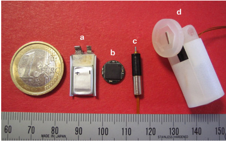
Fig. 14.25 Components of the prototype ((a): Li-Po battery, (b): control board, (c): motor, (d): casing) (© 2009 IEEE), reprinted with permission [48]
