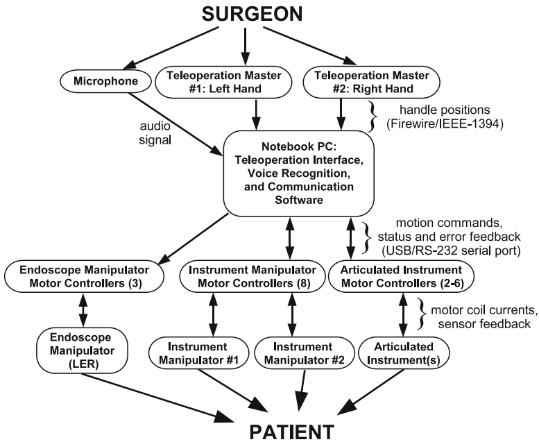
Fig. 7.2 Schematic of communication between modular components of surgical robot system prototype
