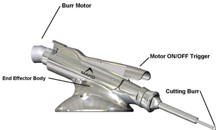
Fig. 10.8 End effector assembly
