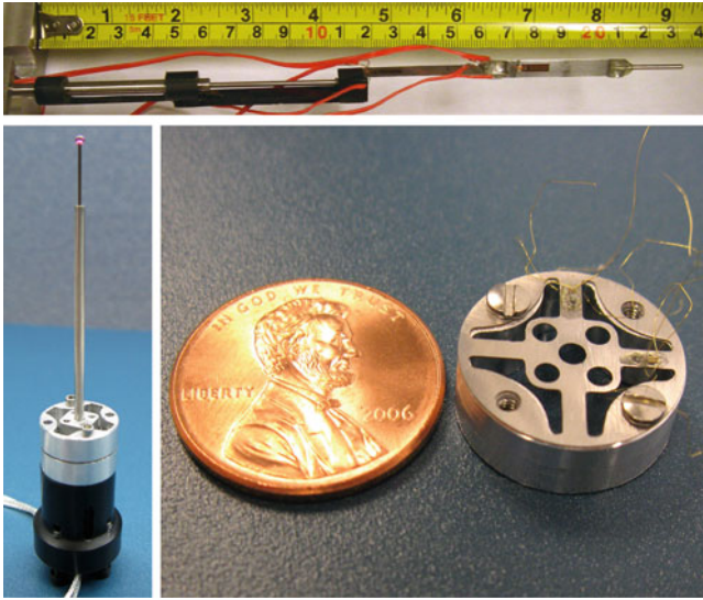
Fig. 22.10 Top – Whisker Sensor Design 1 prototype is shown. Overall length of the sensor when the linear stage is fully retracted and extended are 213 and 239 mm, respectively. Its largest diameter is 12.5 mm. Bottom Left – Whisker Sensor Design 2 is shown. Overall length of the sensor when the linear stage is uncoiled is 60.0 mm. Its largest diameter is 15.3 mm. Bottom Right – Flexure part of the Design 2 shown next to a cent. (© IEEE 2008), reprinted with permission
