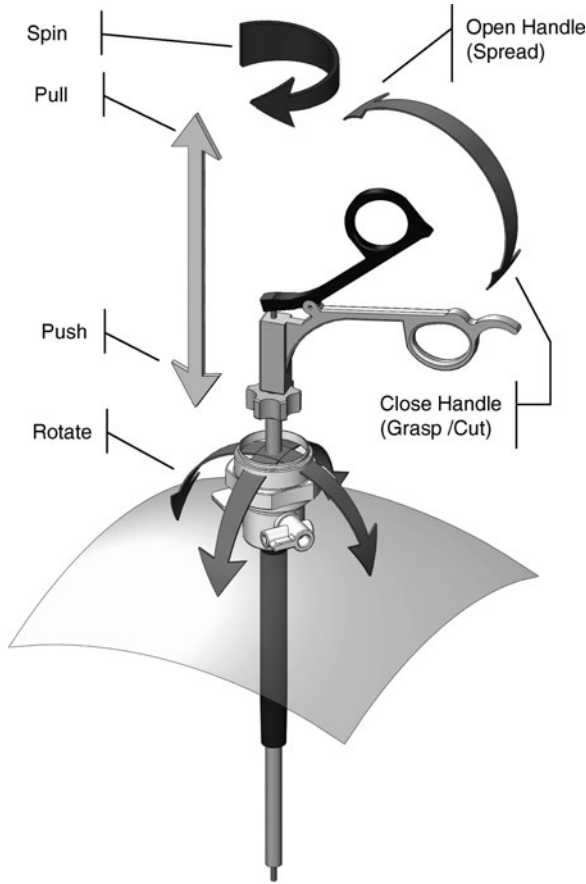
Fig. 25.3 Definition of the five degrees of freedom – DOF (marked by arrows ) of a typical MIS endoscopic tool. Note that two DOF were separated into two distinct actions (Open/Close handle and Pull/Push), and the other two were lumped into one action (Rotate) for representing the tool tip tissue interactions (omitted in the illustration). The terminology associated with the various DOF corresponds with the model state definitions (Table 25.1)
