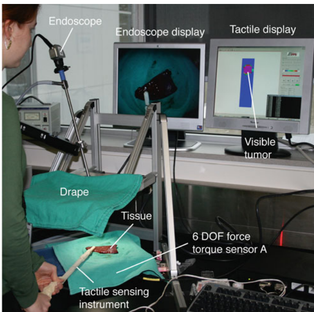
Fig. 20.6 Experimental setup for manual testing of TSI
