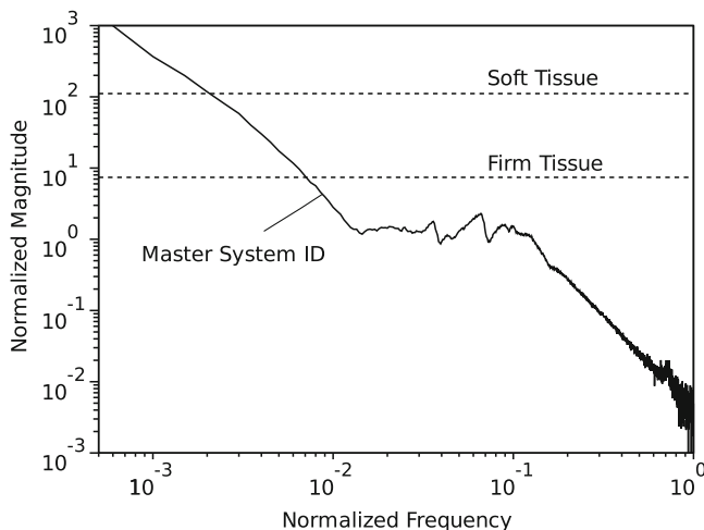
Fig. 18.7 Experimental frequency response of a surgical teleoperator master interface in one degree of freedom. Frequency responses of representative soft and hard tissue stiffnesses are overlaid for reference
