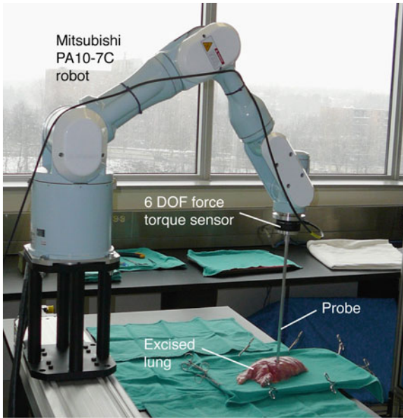
Fig. 20.1 Experimental setup showing the Mitsubishi PA10-7C robot with the palpation probe mounted at the end-effector through a force/torque sensor
