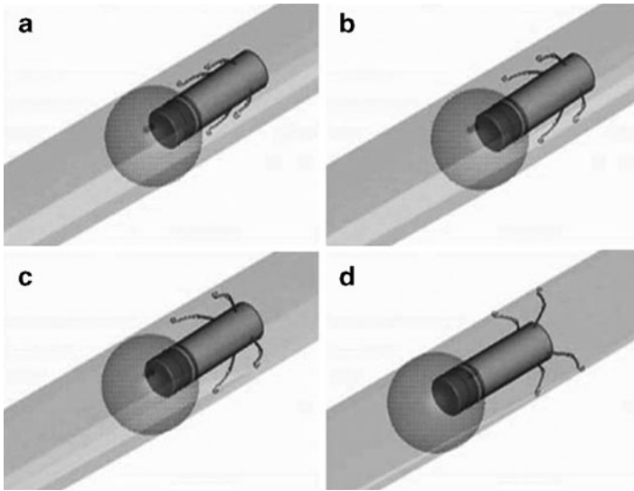
Fig. 14.1 Different positions of the legs in the simulation (© 2008 IEEE), reprinted with permission [11]
