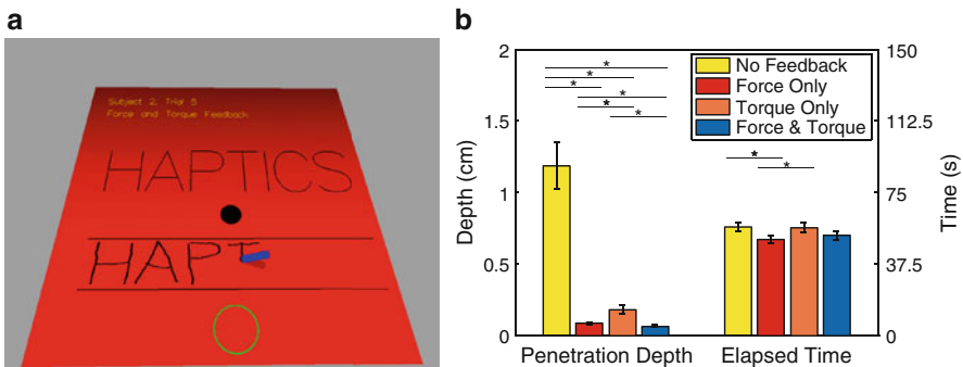
Fig. 18.10 Importance of torque feedback in a 6-DOF system. (a) A screen shot of the virtual “paper” that subjects draw on. (b) Average depth and elapsed time for the transcribing the word “HAPTICS”. Average depth into the virtual wall is significantly increased for the No Feedback condition. The performance of with the Force Only and Force & Torque conditions is similar. Lines with stars above connect conditions that have statistically significantly different means [39], ©IEEE 2009
