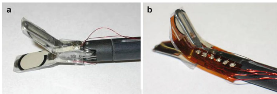
Fig. 19.3 Cadiere graspers with single-element sensors ( left ) and 3 \times 2 array ( right ) (© 2008 IEEE), reprinted with permission
