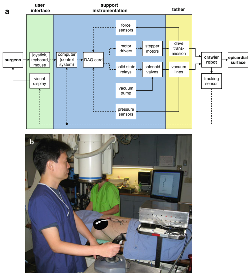
Fig. 5.2 (a) Schematic diagram of the HeartLander system, which comprises the user interface, the support instrumentation, and the tethered crawling robot. Mechanical flow is indicated by solid lines , while data flow is shown by broken lines . (b) Photograph of the operating room during animal testing, showing the surgeon interacting with the HeartLander system. The approximate heart shape and robot location inside the body have been illustrated for clarity
