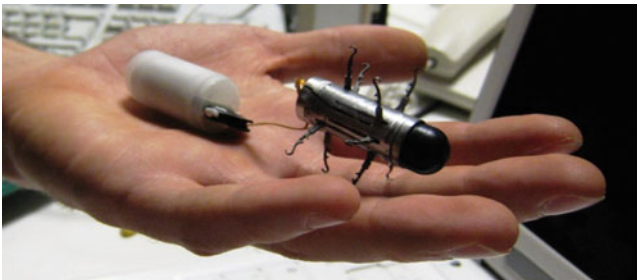
Fig. 14.4 Prototype of 12-leg endoscopic capsular robot. The plastic rear module contains a battery power supply, and will be optimized and miniaturized in future studies (© 2009 IEEE), reprinted with permission [13]
