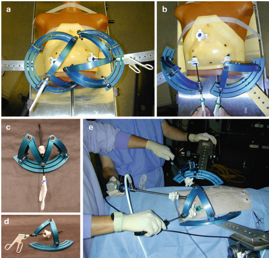
Fig. 8.12 Aluminum Mock-up with adjustable link length and base length. The surgical endo-scope tool is inserted into a guide located at mechanism apex in a configuration that allow to test different design candidates in a real minimally invasive surgical setup. (a) Parallel Configuration (b) Serial Configuration (c, d) Two configurations tested in a MIS setup. (e) Testing the make up in an animal lab. Although the robot manipulator will be teleoperated, in this evaluation the surgeon guides these passive mock-ups in order to evaluate the range of motion
