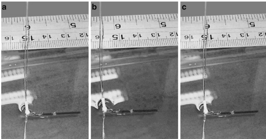
Fig. 16.8 Propulsion experiment: (a) power off; (b) power on with calculated phase shifts; (c) power on with 0 phase shifts (Copyright 2007 IEEE.)
