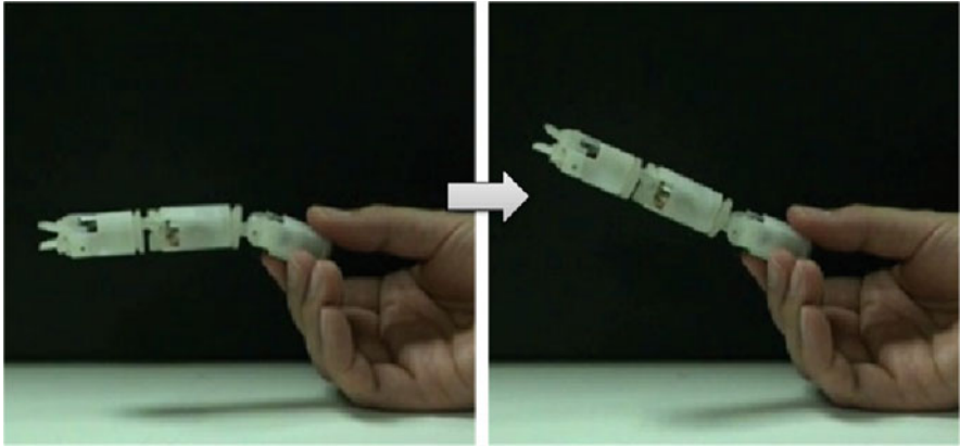
Fig. 14.32 Lift up of the two modules (© 2009 IEEE), reprinted with permission [48]
