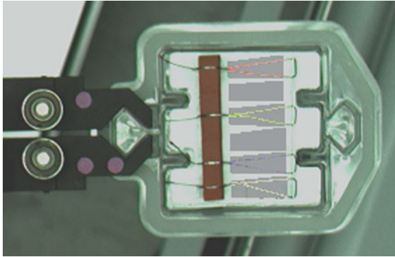
Fig. 3.21 Suture supply tray, held by an SNS gripper with three purple fiducial marks
