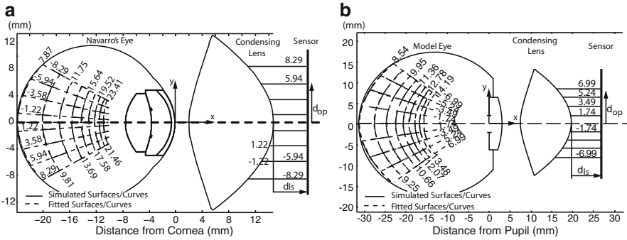
Fig. 13.21 Simulation of the isofocus surfaces and isopixel curves for (a) indirect ophthalmoscopy with Navarro’s eye, and (b) indirect ophthalmoscopy with the model eye [31] (©IEEE 2009), reprinted with permission. The different isofocus surfaces correspond to the distance from the lens to the sensor ( d_{ls} ), for uniform sensor steps of (a) \sim 1.95 mm, and (b) \sim 0.7 mm. The isopixel curves correspond to pixel distances from the optical axis ( d_{op} ), for uniform steps of (a) \sim 2.25 mm, and (b) \sim 1.75 mm
