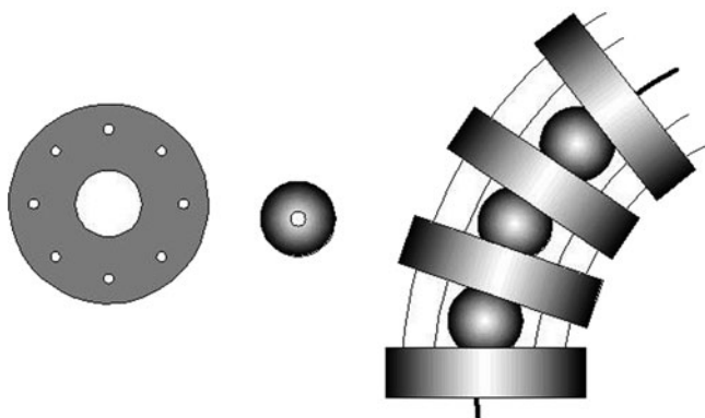
Fig. 7.7 Flexible spine structure for articulated instrument wrist
