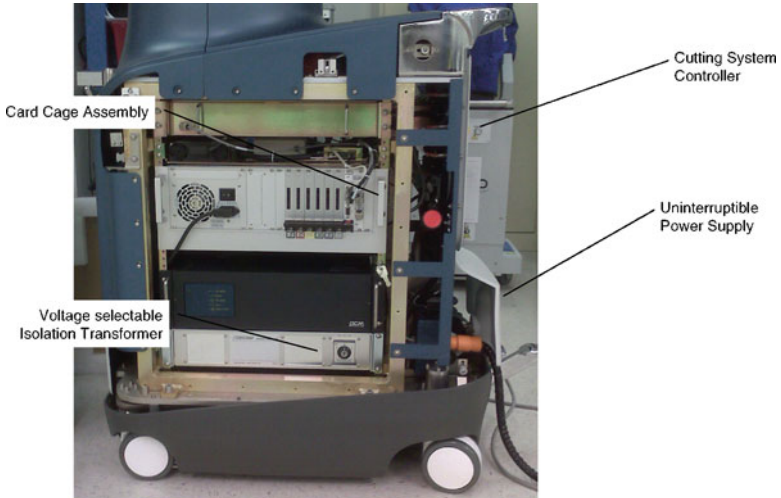
Fig. 10.10 Robotic arm electronics
