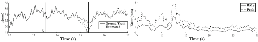
Fig. 21.12 (Top) The original heart motion is slowly damped from t_0 to t_1 to 50% of its original amplitude. (Bottom) The prediction error plot for a 1 second prediction horizon indicates the fast filter adaptation to the amplitude change
