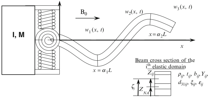
Fig. 16.3 Illustration of the swimming micro robot's tail divided into three sections (Copyright 2007 IEEE.)
