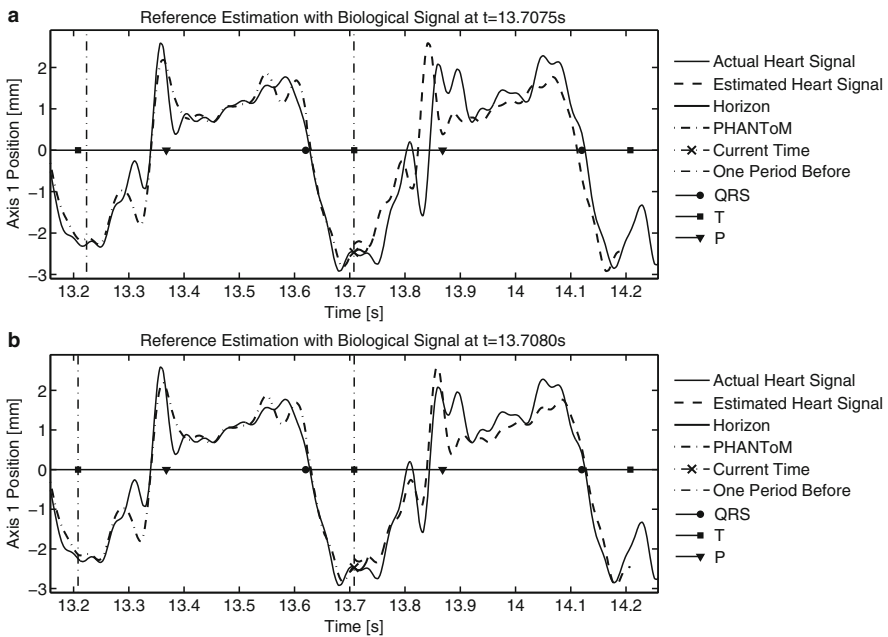
Fig. 22.6 Reference Estimation with Biological Signal. (a) Just before T Wave was detected: Estimated Heart Signal did not fit well with the Actual Heart Signal. T Wave detection was shown with filled square markers. (b) T Wave has been detected: Heart Period and Estimated Signal were adjusted. Observe that the beginning of the previous heartbeat period marker [- - -] ( t \approx 13.22 s) was shifted back in time ( t \approx 13.21 s) as a result of the increase in the heartbeat period. Accordingly, Estimated Heart Signal was changed to adjust with the new period. RMS estimation error was decreased from 0.887 mm to 0.456 mm with the shift (© IEEE 2007), reprinted with permission
