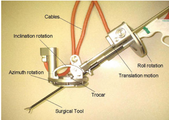
Fig. 7.4 Instrument manipulator holding manual instrument
