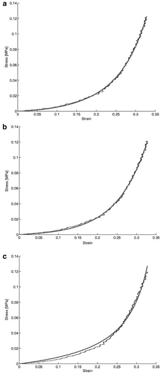
Fig. 24.5 Measured data and phenomenological models of liver tissue under compression loading. The same in-vivo data measured by the MEG was fit with various models. The measures of fit for these models are: (a) EXP2, R^2 = 0.9989 , RMSE = 1.5048E3 ; (b) EXP, R^2 = 0.9984 , RMSE = 1.5166E3 ; (c) INV, R^2 = 0.9931 , RMSE = 3.0291E3
