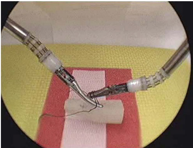
Fig. 7.16 FLS suturing task
