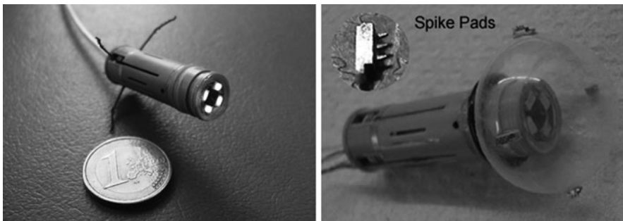
Fig. 14.2 Left : overall view of the four legged capsule prototype. Right : capsule with frontal balloon and a detail of the spike pads (© 2008 IEEE), reprinted with permission [11]
