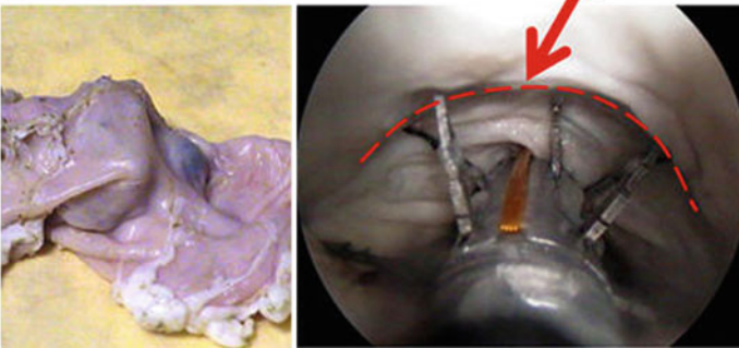
Fig. 14.7 Evaluation of colon wall distension when four (a) or six (b) legs are included in a single leg set. External views of the capsules in the colon are shown in the left images , while endoscopic views of the capsules inside the lumen are shown on the right (© 2009 IEEE), reprinted with permission [13]
