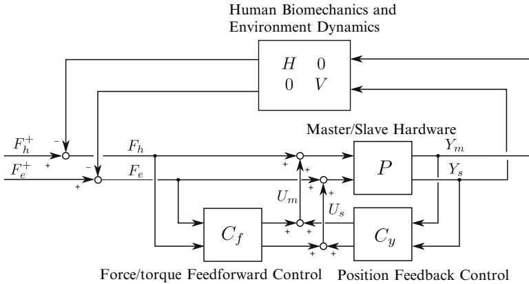
Fig. 18.4 Four-channel control framework for force feedback teleoperation. When C_f and C_y have non-zero off-diagonal terms both force and position measurements are exchanged between the master and slave. Four communication channels are then required to communicate these signals between the master and slave
