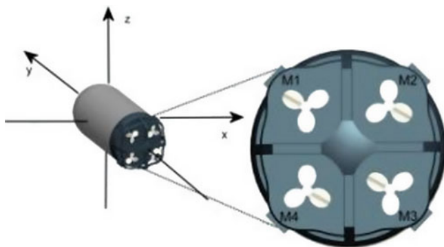
Fig. 14.9 Schematic representation of the capsule and its four propellers (© 2009 Taylor & Francis) [15]
