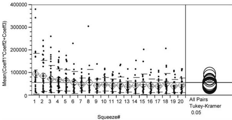
Fig. 24.10 The stiffness indicator scalar b \times a + g of the EXP2 phenomenological model plotted as a function of loading cycle for measured elastic data. The right-hand side of the plot depicts the results from post hoc Tukey-Kramer HSD analysis. The radius of the circle represents the region of confidence (95%)
