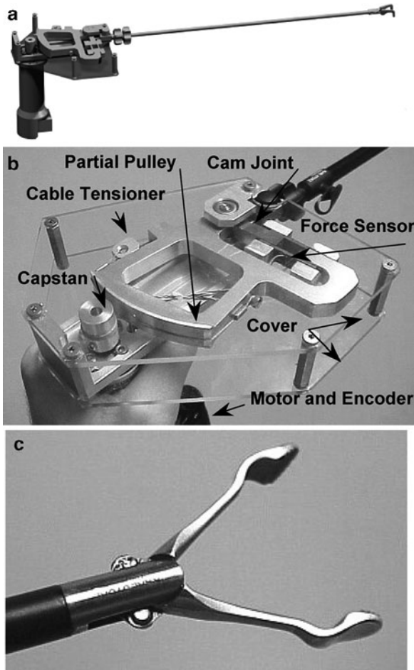
Fig. 24.1 The Motorized Endoscopic Grasper (MEG): (a) rendered CAD drawing of MEG (protective top cover not shown), (b) close-up photograph of the MEG’s drive mechanism, (c) close-up photograph of the MEG’s Babcock grasper end effector
