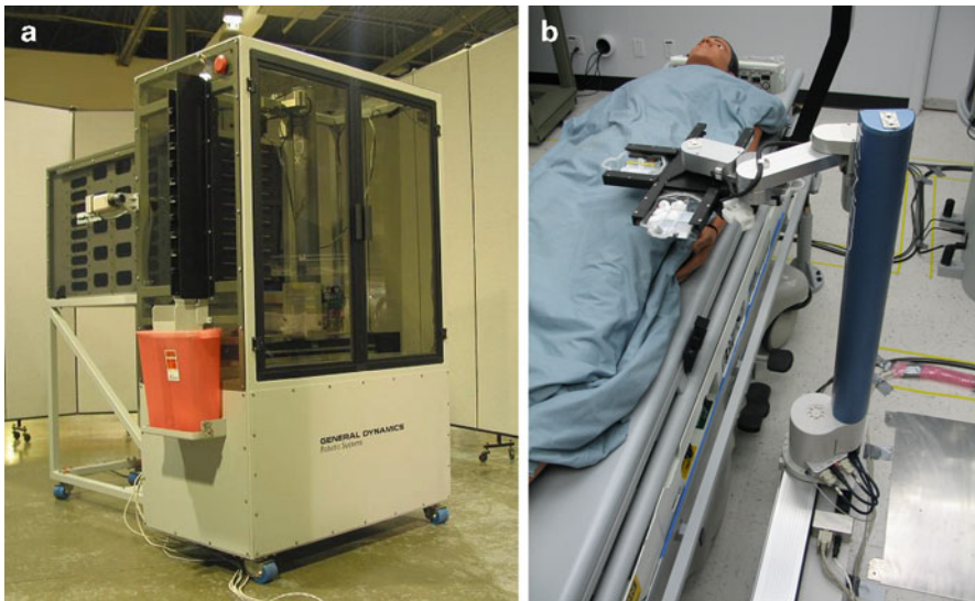
Fig. 3.14 Supply dispensing subsystem. (a) main unit; (b) fast cache (near patient)
