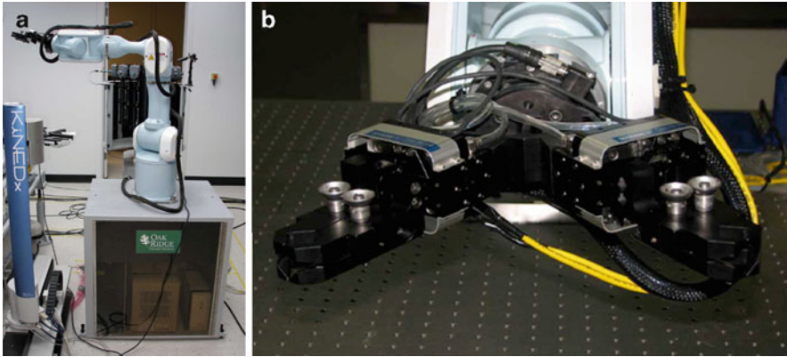
Fig. 3.10 Scrub nurse subsystem. (a) Mitsubishi PA10 robot on a pedestal base; (b) dual gripper end-effector
