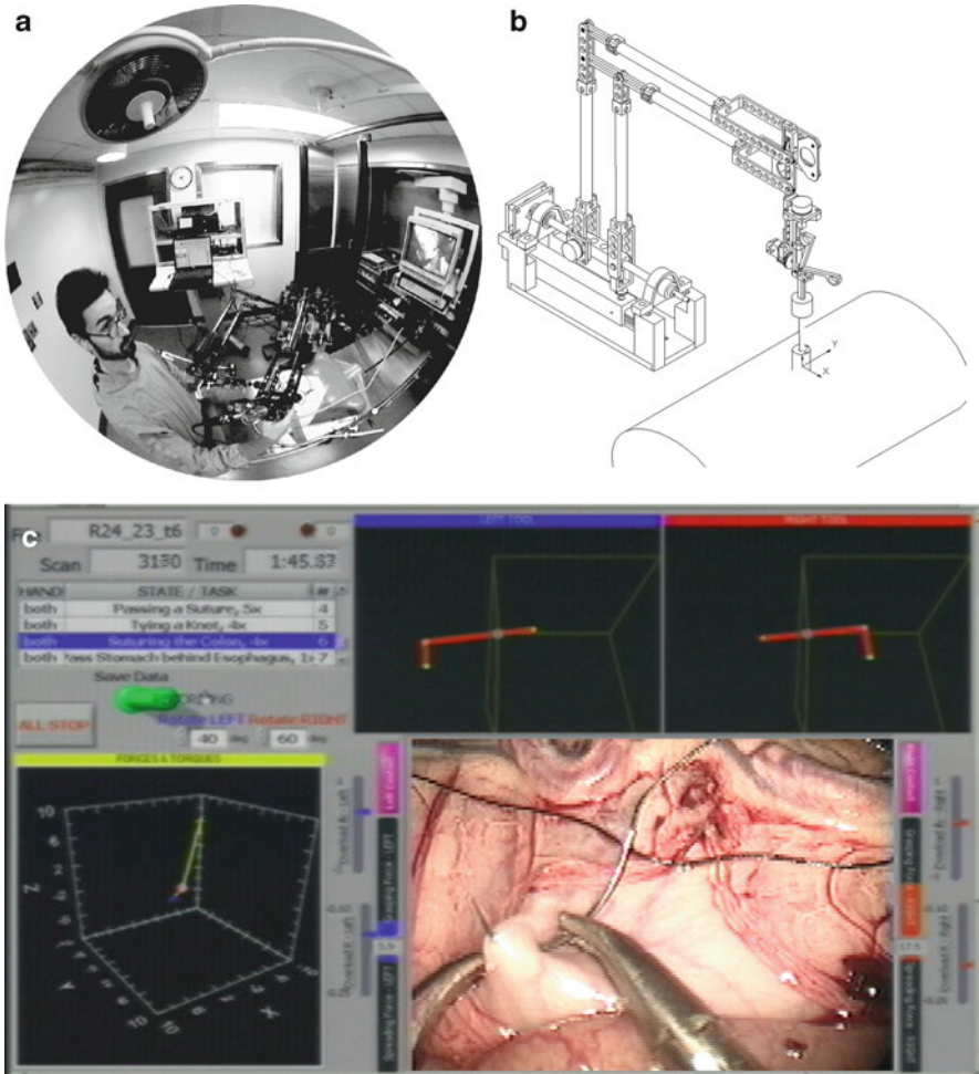
Fig. 25.2 The BlueDRAGON system (a) The system integrated into a minimally invasive surgery operating room (b) CAD drawing of the BlueDRAGON four bar mechanism and its coordinate system properly aligned with the MIS port. (c) Graphical user interface (GUI) incorporating visual view of the surgical seen acquired by the endoscopes video camera ( bottom right ) and real-time information measured by the BlueDRAGONS. On the top right side of the GUI, a virtual representation of the two endoscopic tools are shown along with vectors representing the instantaneous velocities. On the bottom left a three dimensional representation of the forces and torque vectors are presented. Surrounding the endoscopic image are bars representing the grasping/spreading forces applied on the handle and transmitted to the tool tip via the tool’s internal mechanism, along with virtual binary LED indicating contact between the tool tips and the tissues
