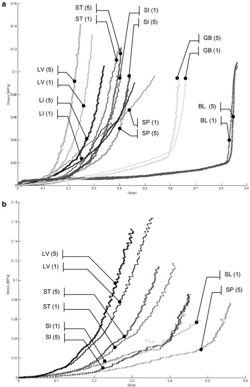
Fig. 24.3 Stress-strain curves for all organs under study, as measured with the MEG at 5.4 mm/s loading velocity (first and fifth cycles shown): (a) in-vivo, (b) ex-corpis. Organs' legends: BL bladder, GL gallbladder, LI large intestine, LV liver, SI small intestine, SP spleen, ST stomach. The loading cycle number (1 or 5) is defined in the brackets
