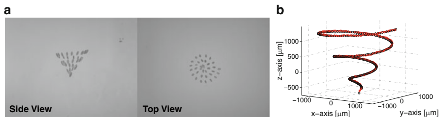
Fig. 13.15 Demonstration of automated pose control (©IEEE 2010), reprinted with permission. Both time-lapse image sequences (a) show a 500- \mu\text{m} -long microrobot following a spiral trajectory keeping its orientation constantly pointing at the vertex of the spiral. Way points ( black circle ) and tracker data ( red plus ) are shown in the isometric graph (b). Average trajectory-completion time: 33.4 s
