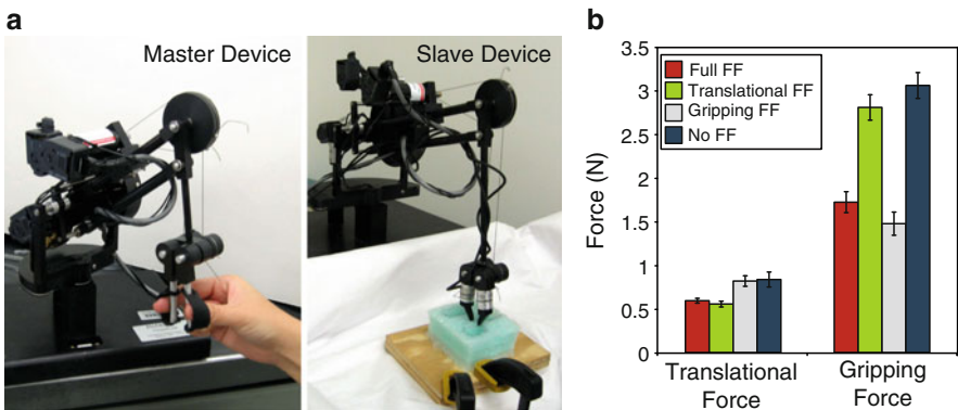
Fig. 18.9 Grip force feedback experiment. (a) A 4-DOF telemanipulator, consists of two PHANTOM haptic devices with added gripping mechanism [41], ©IEEE 2007. (b) Average applied force for 5 subjects performing the peg-in-hole task. Applied translational forces were only affected by force feedback in the translational DOFs. Similarly, applied grip force was only affected by feedback given in the gripping DOF [40]
