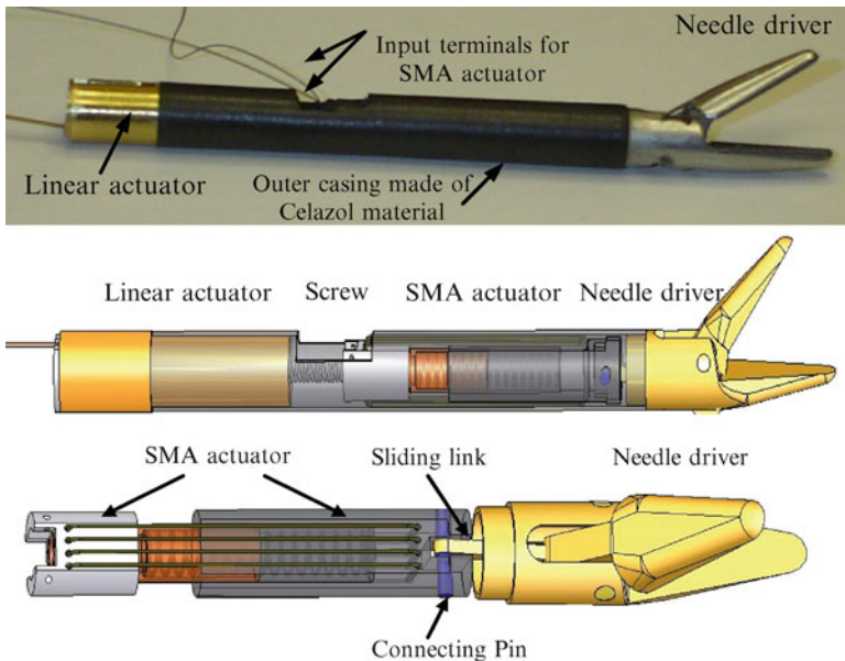
Fig. 22.11 The second generation design prototype. Top – Photograph of the prototype. Middle – CAD model of the design. Bottom – CAD model of the assembly of SMA actuator and the needle driver (© IEEE 2007), reprinted with permission
