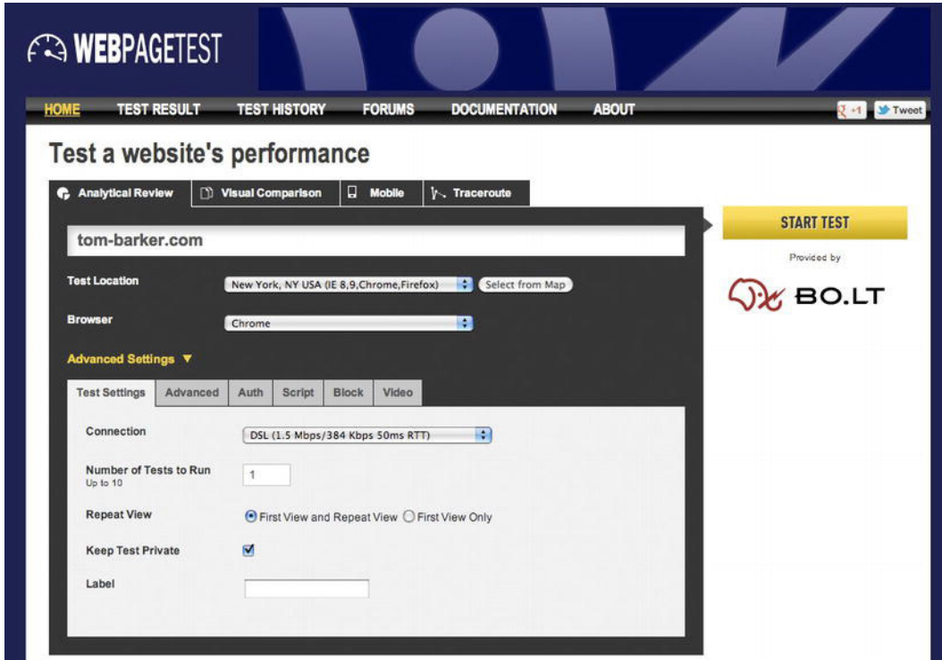
Figure 2-11. Webpagetest.org
