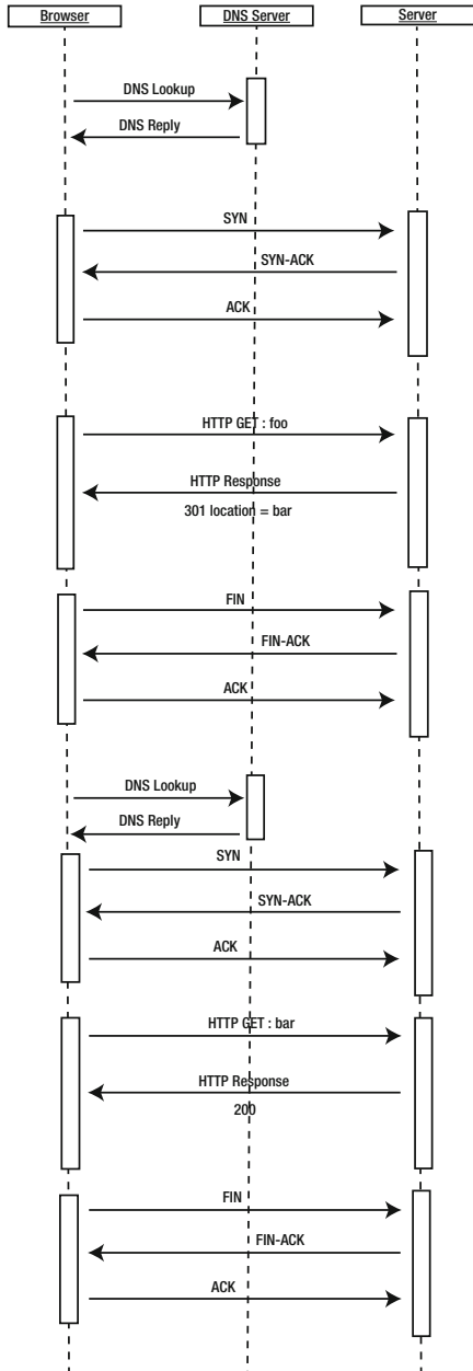
Figure 5-5. HTTP Redirect
