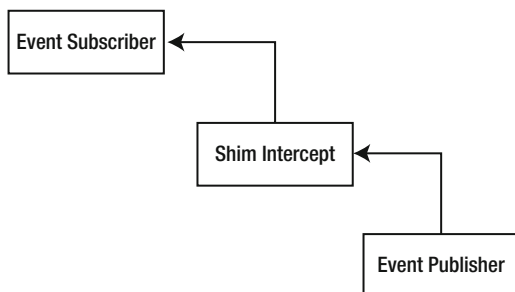
Figure 5-9. Intercept
