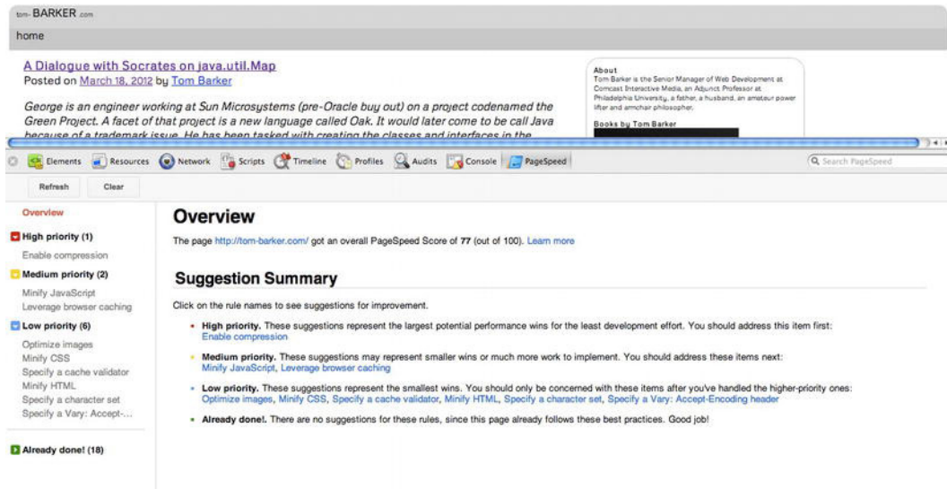
Figure 2-10. Page Speed results
