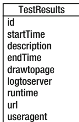
Figure 4-5. TestResults object diagram
