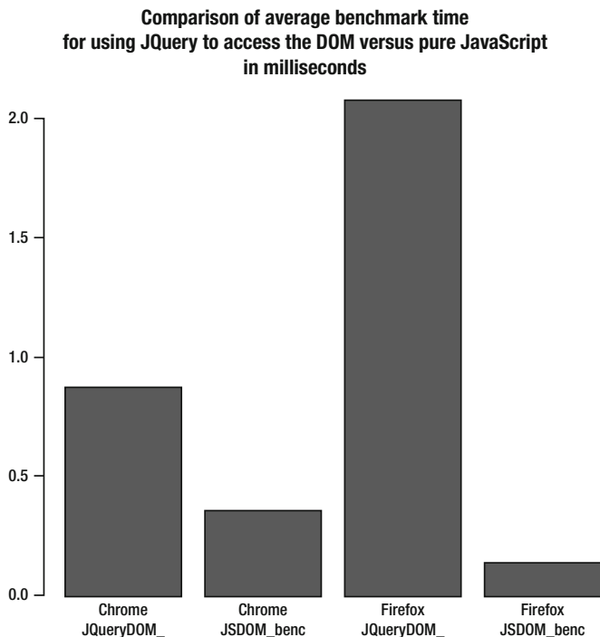
Figure 7-6. Comparison of benchmark results for DOM interaction with JQuery and with JavaScript, by browser
