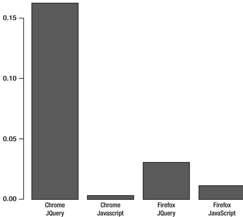
Figure 7-5. Comparison of benchmark results for looping with JQuery versus looping with core JavaScript, by browser
