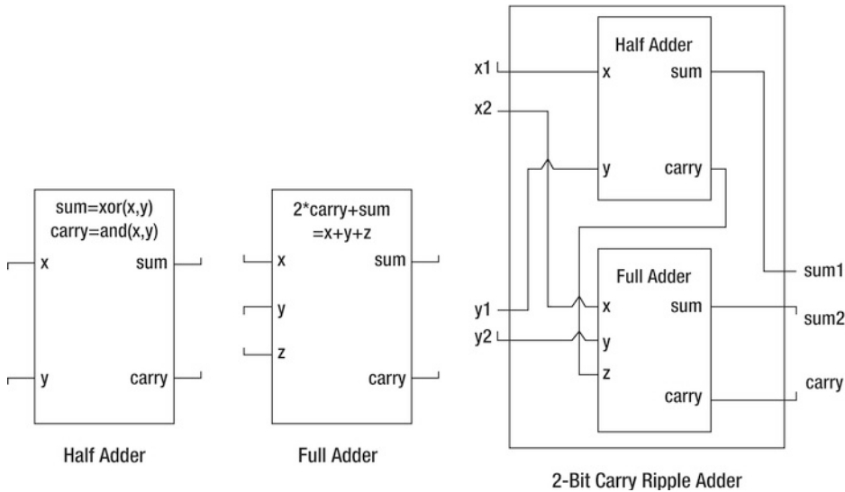
Figure 12-1. Three simple hardware circuits
