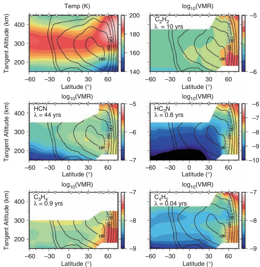
Fig. 13.10 Cross sections of temperature (upper left panel) and composition from CIRS mid-infrared limb sounding. Composition is given as a volume mixing ratio and the position of the observed limb profiles are denoted by the inverted triangles at the top of each plot. Contours indicate the vortex zonal wind speeds (in \text{m s}^{-1} ) derived by Achterberg et al. (2008a) and blue dashed lines show the region with the steepest horizontal potential vorticity gradient, which indicates a dynamical mixing barrier. Altitudes with low signal-to-noise or where the atmosphere becomes opaque are not plotted. Note that southern latitudes are toward the left of each panel. VMR denotes the volume mixing ratio and \lambda is the photochemical lifetime at 300 km (after Teanby et al. 2008)
