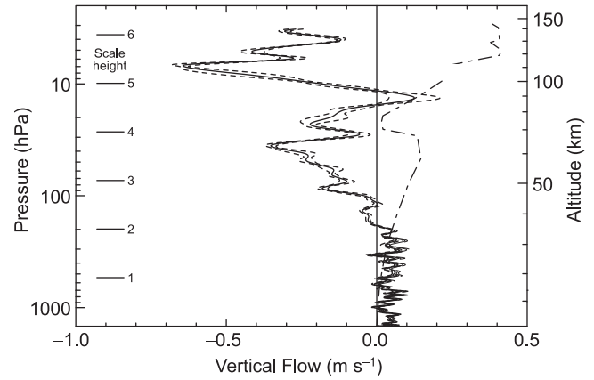
Fig. 13.11 Solid curve: vertical atmospheric velocity along the descent trajectory of the Huygens probe. Dashed curves: the error envelope. Dot-dashed curve: Zonal wind derived from the Huygens DWE, scaled down by a factor of 1/250 (after Mäkinen et al. 2006)
