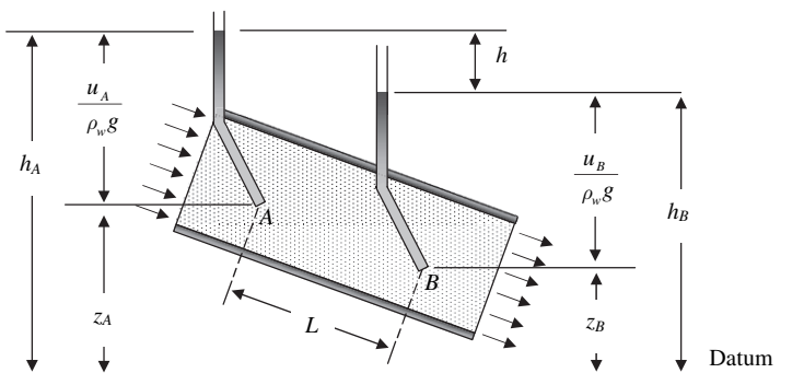
Fig. 2.6 Head loss as water flows through a porous media. Where u = pore water pressures, h = heads, z & L = distances
