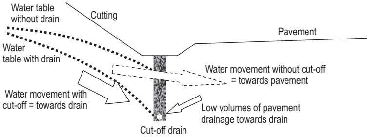
Fig. 13.23 Cut-off drain operation
