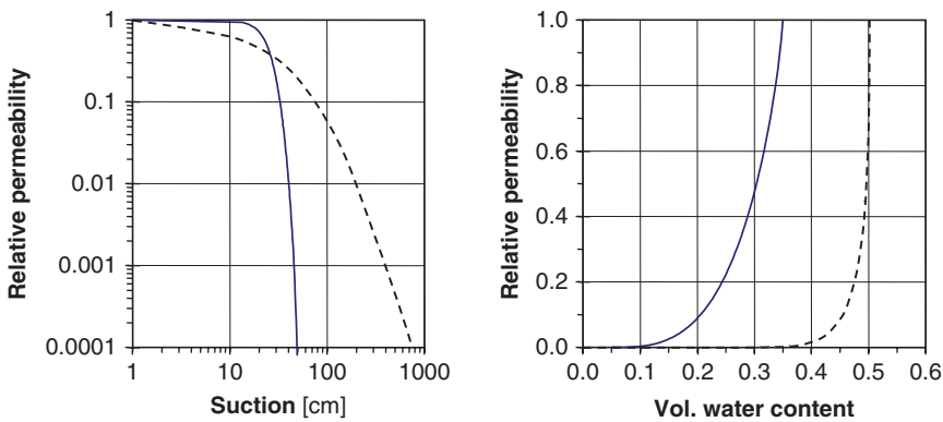
Fig. 2.11 Water-relative permeability for a coarse ( unbroken line ) and fine grained ( dotted line , mostly to the right in each figure) soil using van Genuchten’s equation. The parameters used to plot the curves are given in Table 2.2
