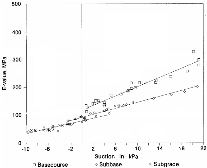
Fig. 10.20 E-values versus granular material suction measured at three depths (Krarp, 1995). Reproduced by permission of the Danish Road Institute
