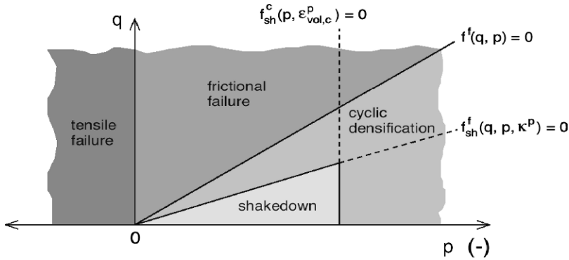
Fig. 9.7 Map of various response regimes in (p, q) plane during cyclic loading (Suiker and de Borst, 2003). Copyright John Wiley & Sons Limited. Reproduced with permission
