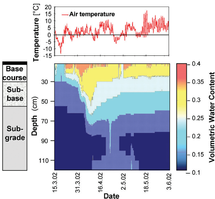
Fig. 8.9 Volumetric water content ( right scale ) during a spring thaw period for a thin pavement structure with an granular base course. The air temperature is also shown, top, as well as a cross section through the low volume pavement structure
