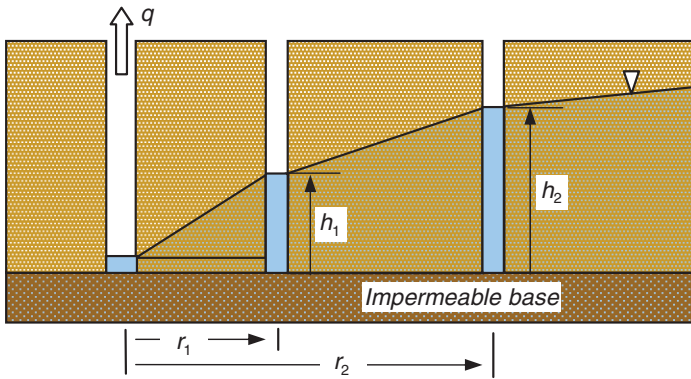
Fig. 3.10 Pumping test from a well with two observation wells in an unconfined permeable soil layer with an impermeable stratum underneath
