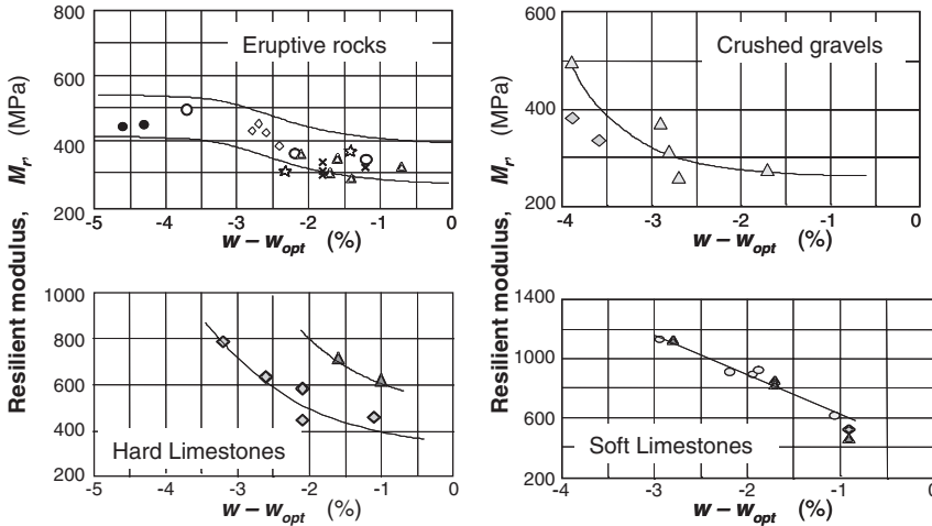
Fig. 10.12 Sensitivity to moisture of unbound granular materials of different origin (Hornych et al., 1998)
