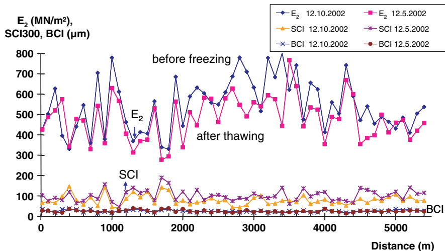
Fig. 8.10 FWD Measurements after thawing and before freezing for a Finnish pavement. SCI = Surface curvature index, BCI = Base Curvature Index, E_2 = stiffness modulus (see Section 10.3)
