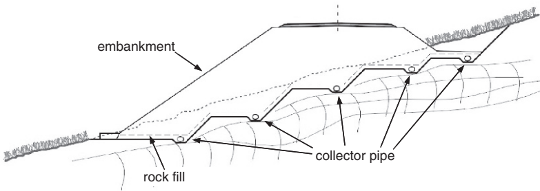
Fig. 13.25 Longitudinal drains in "1/2 hillside"
