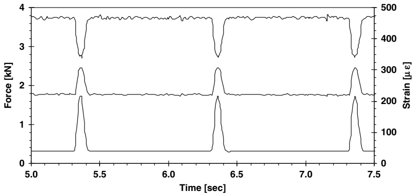
Fig. 10.2 Measured response of an unbound granular specimen (Erlingsson & Magnusdottir, 2002) Note: Three symmetric haversine load pulses (the lowest curve) are shown and the strain response from one of the vertical transducers (the top curve) as well as the horizontal transducer (the middle curve). The vertical transducer shows compression during the load pulses and the horizontal one shows extension.
