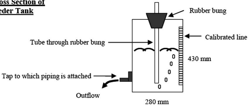
Fig. 5.3 Infiltrimeter used by Taylor (2004). Reproduced with permission of J. Taylor
