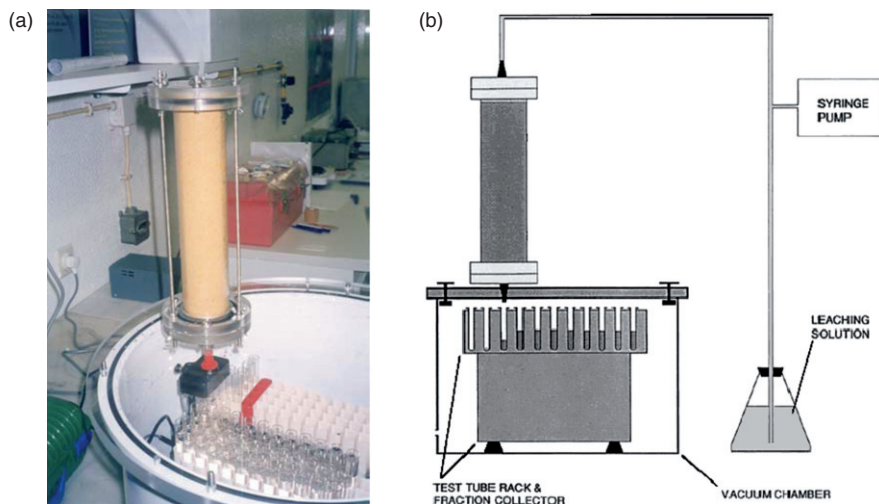
Fig. 7.10 Down-flow percolation test device; (a) photograph, (b) line diagram. Diagram reproduced by permission of Soil Measurement Systems.com
