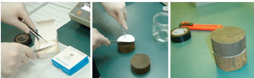
Fig. 3.17 Contact filter paper setup procedure (in laboratory). Reproduced with permission of R. Bulut
