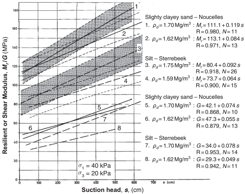
Fig. 10.18 Correlations between the resilient modulus and the suction for the two soils analyzed for a confining pressure of 20 kPa and a deviatoric stress of 20 kPa (Brüll, 1983). Figure courtesy of the Belgian Road Research Centre
