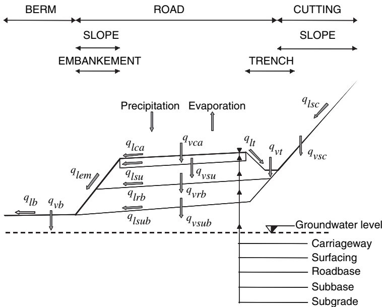
Fig. 2.1 Conceptual model of water balance on pavement – embankment system. v = vertical, l = lateral, ca = carriageway, su = surfacing, rb = roadbase, sub = sub-base, sc = slope/cutting, t = trench, em = embankment and b = berm
