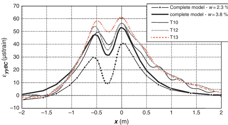
Fig. 11.15 Comparison of experimental and predicted transversal strain \epsilon_{yy} at the bottom of the bituminous layer – load 65 kN
