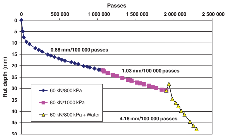
Fig. 8.5 Rut depth propagation rates during test SE01. Figure courtesy L. Wiman, reproduced by permission of VTI
