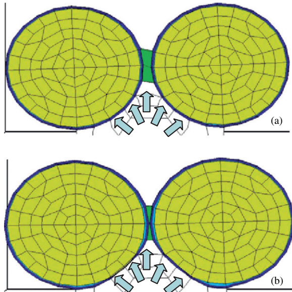
Fig. 5.13 Finite element simulation of (a) cohesive versus (b) adhesive failure (Kringos & Scarpas, 2005a)
