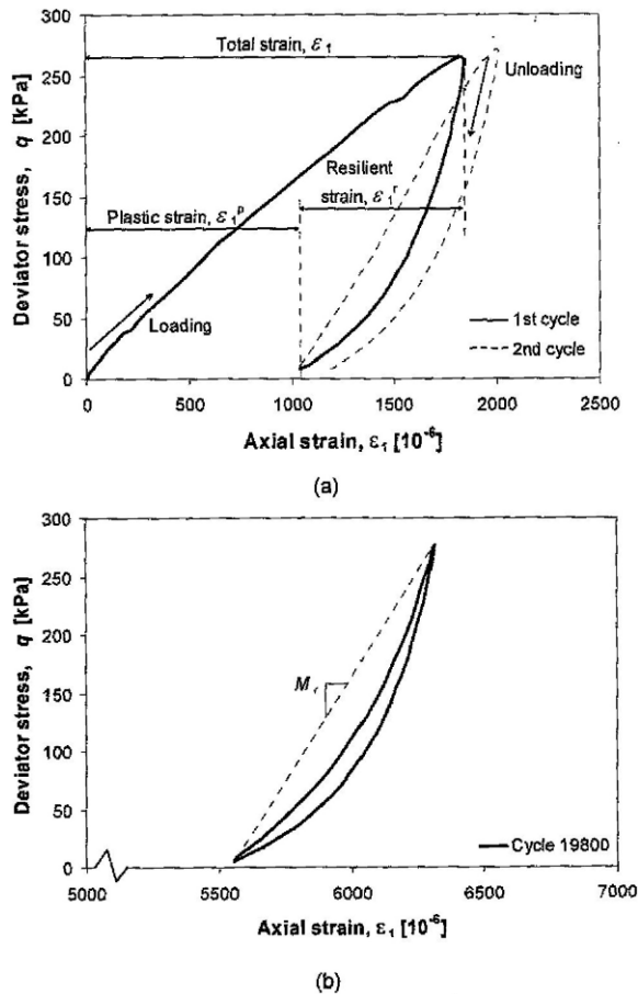
Fig. 9.3 Resilient behaviour shown as deviatoric stress versus axial strain during cyclic testing, (a) on initial loading (b) after a large number of cycles, after Ekblad (2004). Reproduced by permission of Jonas Ekblad
