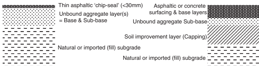
Fig. 1.5 Some typical pavement profiles ( left = low volume, right = higher volume)
