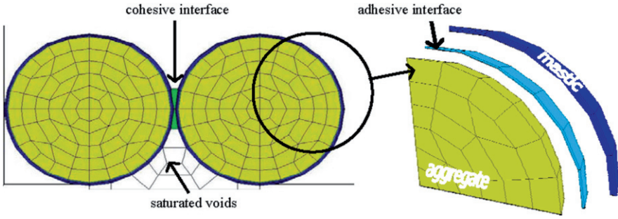
Fig. 5.12 Cohesive versus adhesive interface elements (Kringos & Scarpas, 2005a)
