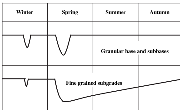
Fig. 8.7 Schematic overview of seasonal variation of stiffness
