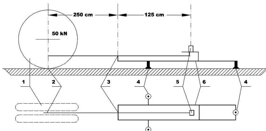
Fig. 10.4 Benkelman beam: (1) dual tyres of a loaded vehicle, (2) tip of the beam, (3) ball bearing, (4) adjustable support legs, (5) dial test indicator, (6) stand (Tehnicne specifikacije za ceste, TSC 06.630, 2002). Reproduced by permission of Direkcija Republike Slovenije za Ceste
