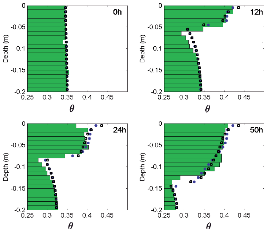
Fig. 11.7 Simulated ( symbols ) and measured values ( horizontal bars ) of the total volumetric water content 0, 12, 24 and 50 h after freezing started. A variable convective heat transfer coefficient, h_c , was used for the first simulation ( solid circles ) and a heat leakage bottom boundary for the second ( open circles ). Simulated values were averaged over 1-cm intervals
