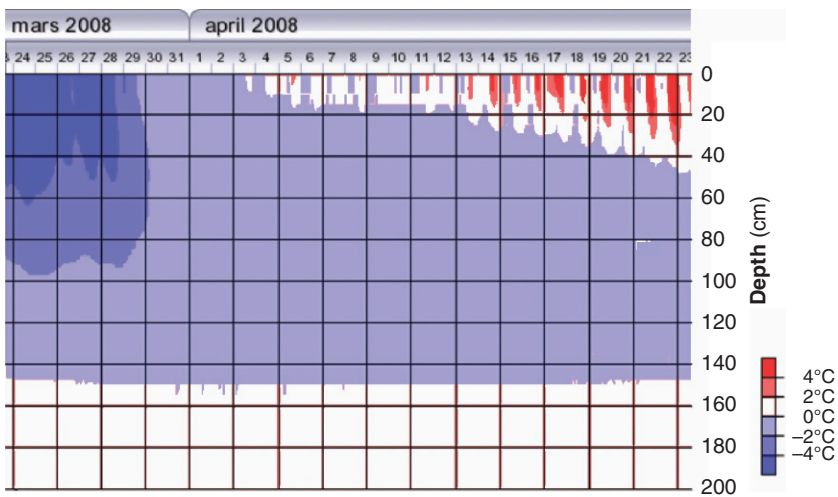
Fig. 8.13 Temperature profile monitored by the Swedish Tjäl2004, distributed via the Internet, see http://www3.vv.se/tjaldjup/
