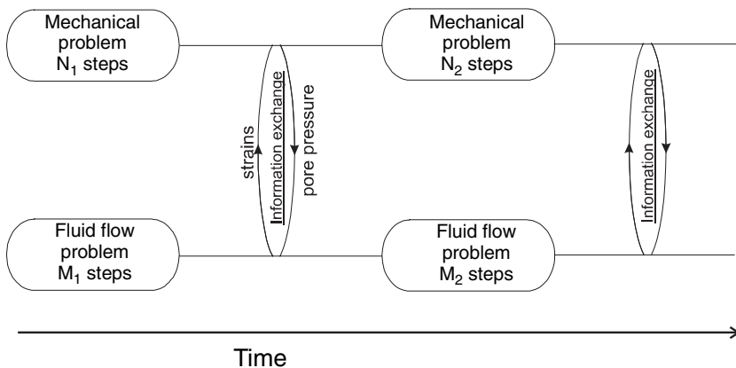
Fig. 11.3 Scheme of a staggered coupling
