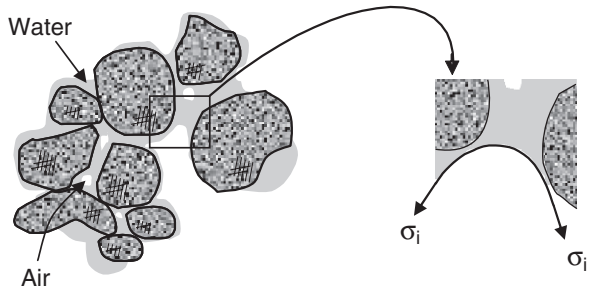
Fig. 2.8 (a) Distribution of water in a porous media. (b) Curved interface separating water and air phases
