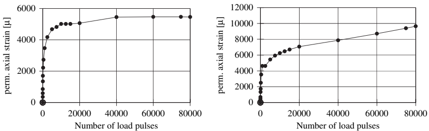
Fig. 10.3 Typical results from permanent deformation testing where the accumulated axial strain is shown as a function of the number of load pulses in the permanent deformation tests (Erlingsson, 2000)
