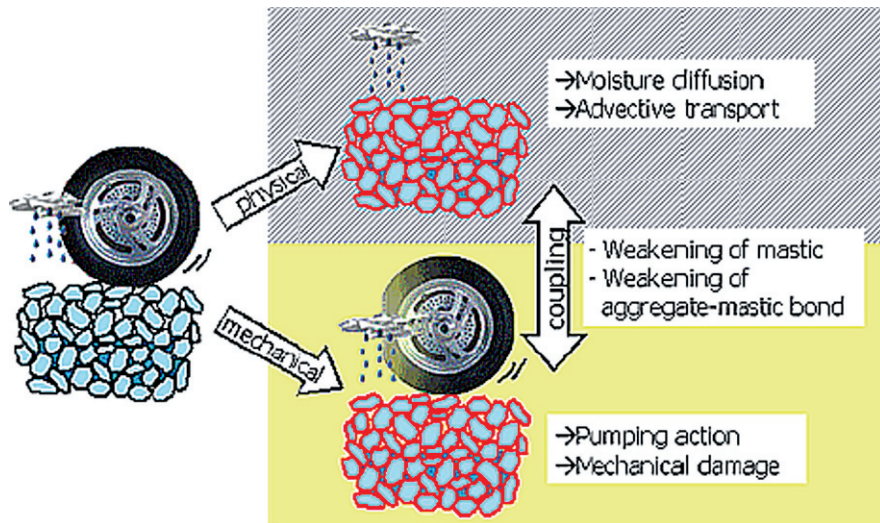
Fig. 5.7 Separation of water damage into physical and mechanical processes (Kringos, 2007)
