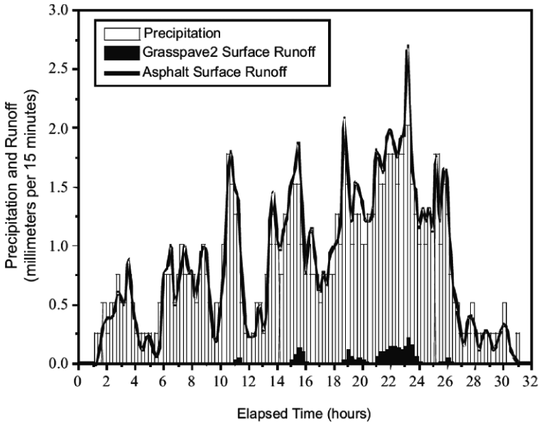
Fig. 13.12 Rainfall and runoff from two car park pavements (after Brattebo & Booth, 2002). Reproduced by permission of Derek Booth
