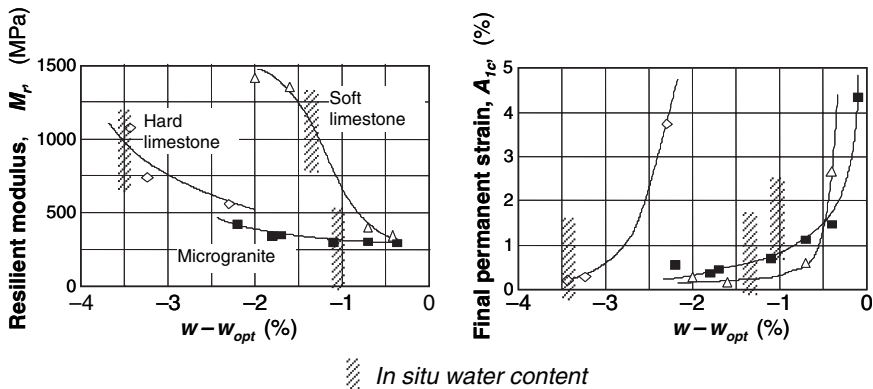
Fig. 10.10 Influence of water content, w , on the resilient modulus, M_r , and permanent axial strains, A_{1c} , of 3 French unbound granular materials: hard limestone, soft limestone and microgranite (Hornych et al., 1998)
