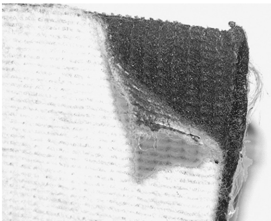
Fig. 13.37 A stress-absorbing membrane. In this case a bitumen-rich interlayer is contained between two geosynthetic sheets which have to be sealed to the old pavement and to the new overlay (sample courtesy of MacPave Corporation)
