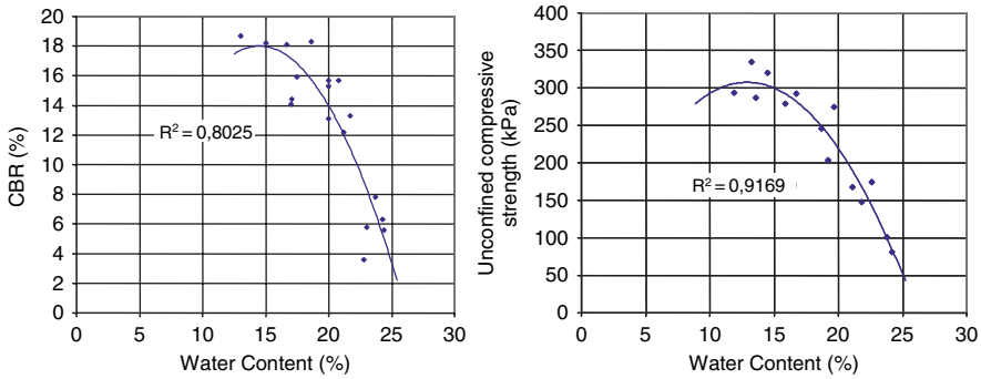
Fig. 10.9 CBR values and unconfined compression strength related to water content for a clay from the Lenart area in Slovenia (adapted from Petkovšek et al., 2003). Reproduced by permission of Direkcija Republike Slovenije za Ceste
