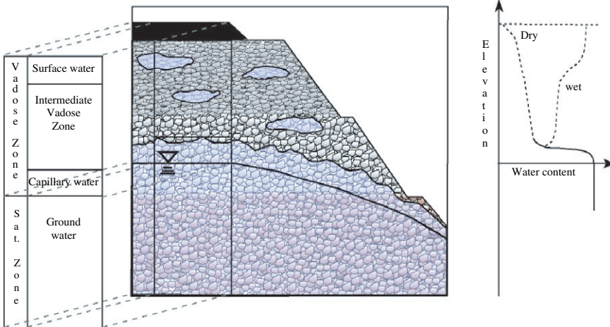
Fig. 2.2 Conceptual model of the relation between road and groundwater
