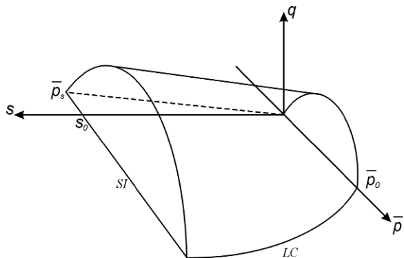
Fig. 9.10 BBM yield surface – coupling \bar{p} - q - s state variables
