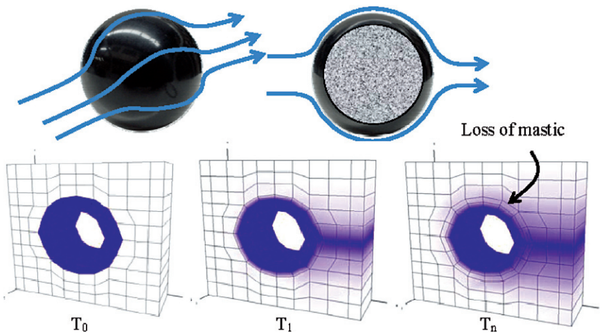
Fig. 5.9 Simulation of loss of mastic from around a coarse aggregate particle due to a fast water flow field Aggregate is omitted in Finite Element model shown in the lower part of the figure.
