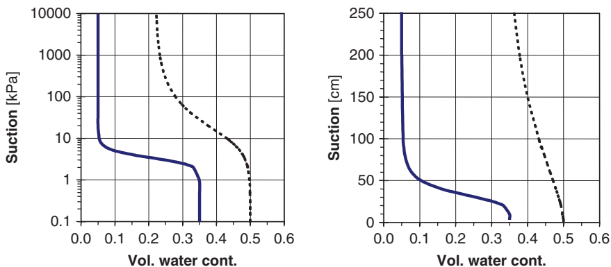
Fig. 2.10 Typical SWCC for a coarse (unbroken line) and fine grained (dotted line) soil using the van Genuchten’s model. The parameter used to plot the curves are given in Table 2.2
