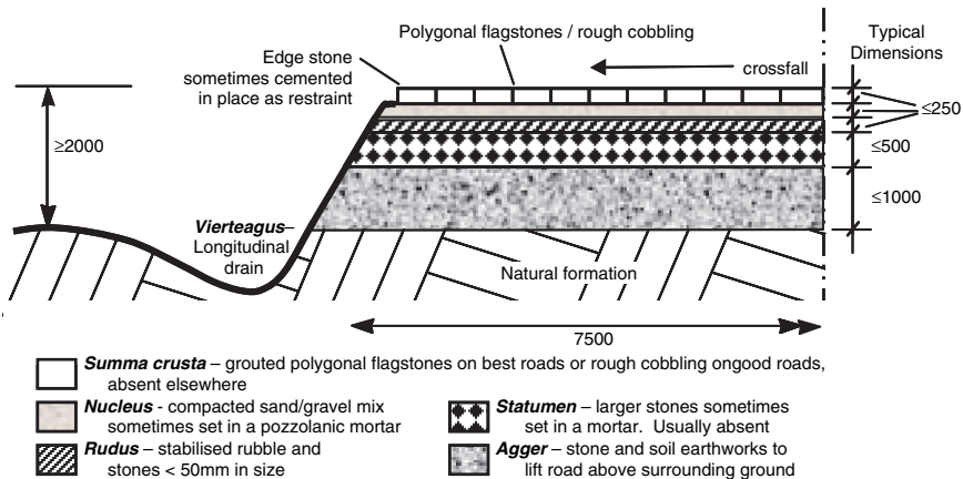
Fig. 1.2 Cross-section of a high quality Roman pavement (dimensions in mm)
