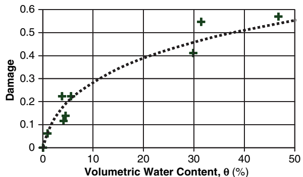
Fig. 5.11 Aggregate-mastic bond strength as a function of water (adapted from Copeland et al., 2007)
