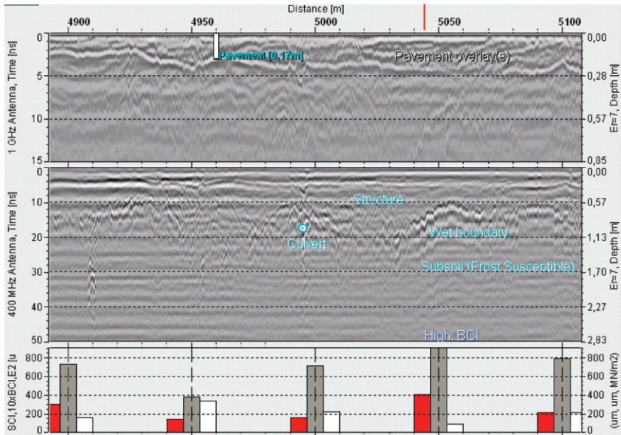
Fig. 3.4 Ground penetrating radar images using a 1 GHz antenna ( top ) and 400 MHz antenna ( middle ) along with FWD parameters (SCI, 10×BCI, E_2 ) ( bottom ) from a 200 m long section on a low volume road in Finland. SCI and BCI are the Surface and Base Curvature Indices, respectively, and E_2 is the stiffness of the pavement structure. See text for explanation
