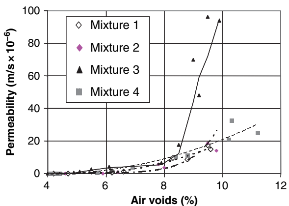
Fig. 5.1 Laboratory determination of permeability of laboratory moulded cylinders of asphaltic mixtures (see Table 5.1 [Vivar & Haddock, 2007]). Reproduced with permission of J. Haddock
