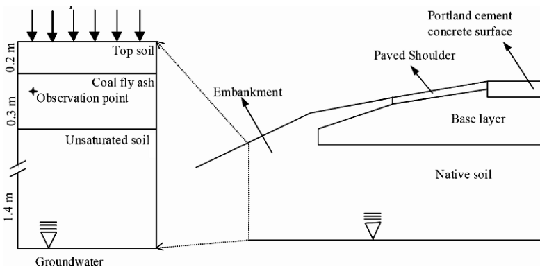
Fig. 11.20 (a) Cross section of MnROAD test Section 12; (b) conceptual model of the MnROAD embankment (Apul et al., 2003). Reproduced by permission of ISCOWA
