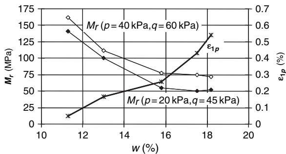
Fig. 10.16 Variations of resilient modulus, M_r , and permanent axial strains with moisture content for a silt (Hornych et al., 1998)
