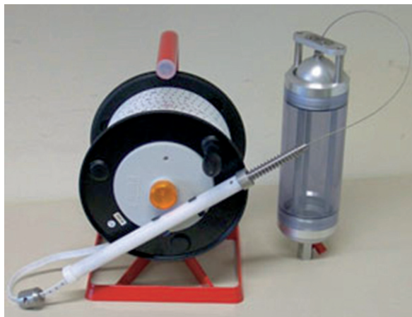
Fig. 7.6 Example of a groundwater sampler: a bailer filled by lowering beneath water surface so that tube fills from the top. Reproduced by permission of Hydrokit
