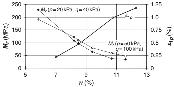
Fig. 10.15 Variations of resilient modulus M_r and permanent axial strains with moisture content for a clayey sand (Hornych et al., 1998)
