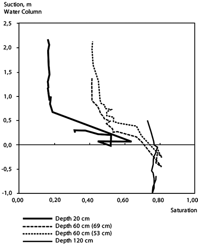
Fig. 10.23 Soil suction measured with tensiometers and saturation measured with the moisture/density probe (Krarpur, 1995). Reproduced by permission of the Danish Road Institute Note: Where measurements were carried out at different depths, the depths of the tensiometer are given in brackets (69 cm). The curves are time series beginning from the left (high suction).
