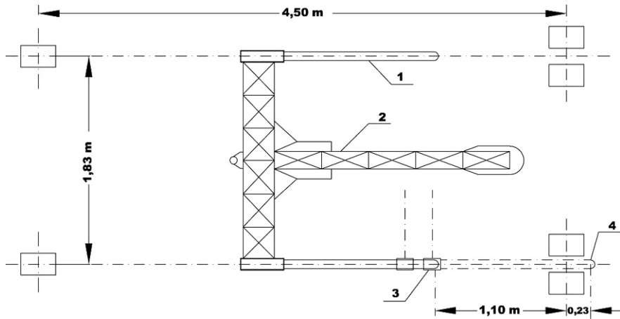
Fig. 10.5 Deflectograph Lacroix equipment: (1) measuring beam, (2) T frame, (3) starting position of tip of measuring beam, (4) end position of tip of measuring beam (Tehnicne specifikacije za ceste, TSC 06.630, 2002). Reproduced by permission of Direkcija Republike Slovenije za Ceste
