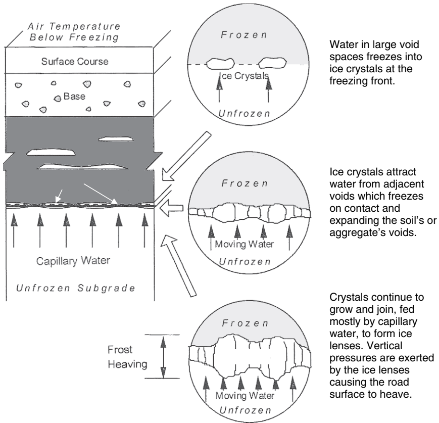
Fig. 4.3 Formation of ice lenses in a pavement structure (WSDOT, 1998)
