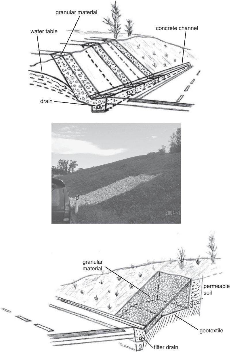
Fig. 13.22 Drainage spurs
