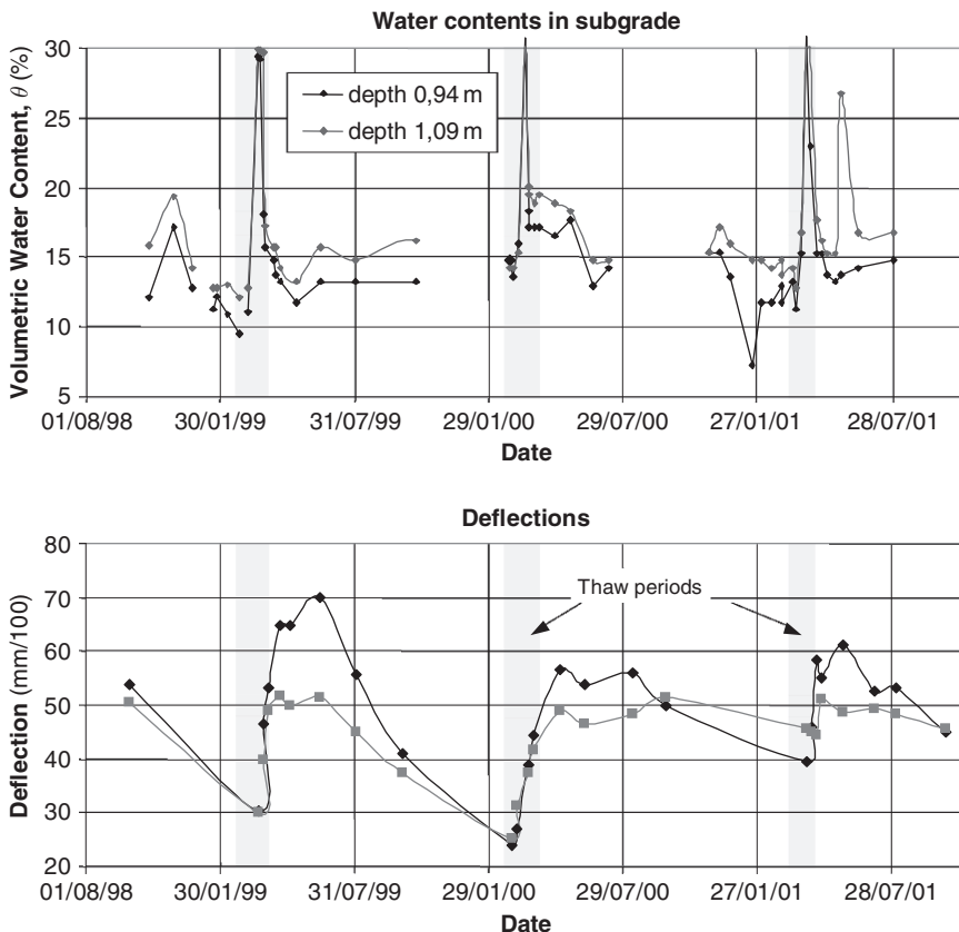
Fig. 8.8 Deflection (caused by loading of pavement) and water content as a function of time – example from Quebec. Grey = Thaw periods
