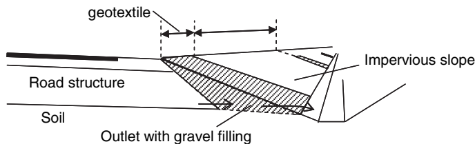
Fig. 13.9 Outlet with gravel filling on a low permeability slope
