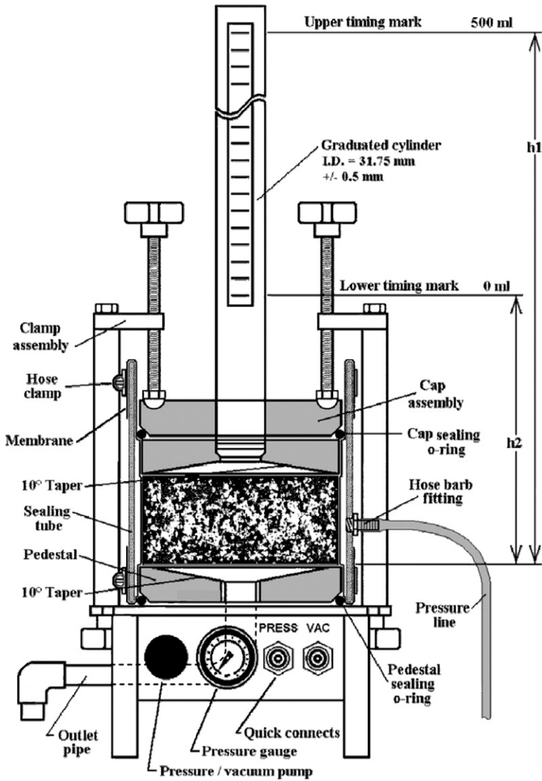
Fig. 5.2 Laboratory permeameter for cores of asphaltic mixtures (FDOT, 2006). Reproduced courtesy of the Florida Department of Transportation
