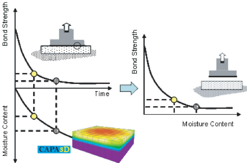
Fig. 5.10 Experimental-computational methodology for determination of the aggregate-mastic bond strength as a function of water content (Kringos & Scarpas, 2005b). Reproduced by permission of N. Kringos
