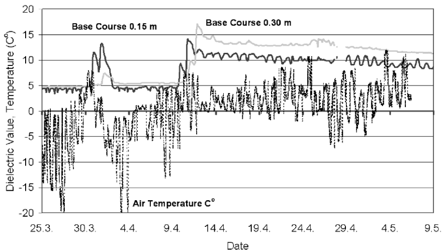
Fig. 8.12 Dielectric values and air temperature monitored by the Koskenkylä Percostation during spring 2000 (Saarenketo et al., 2002). Reproduced by permission of T. Saarenketo
