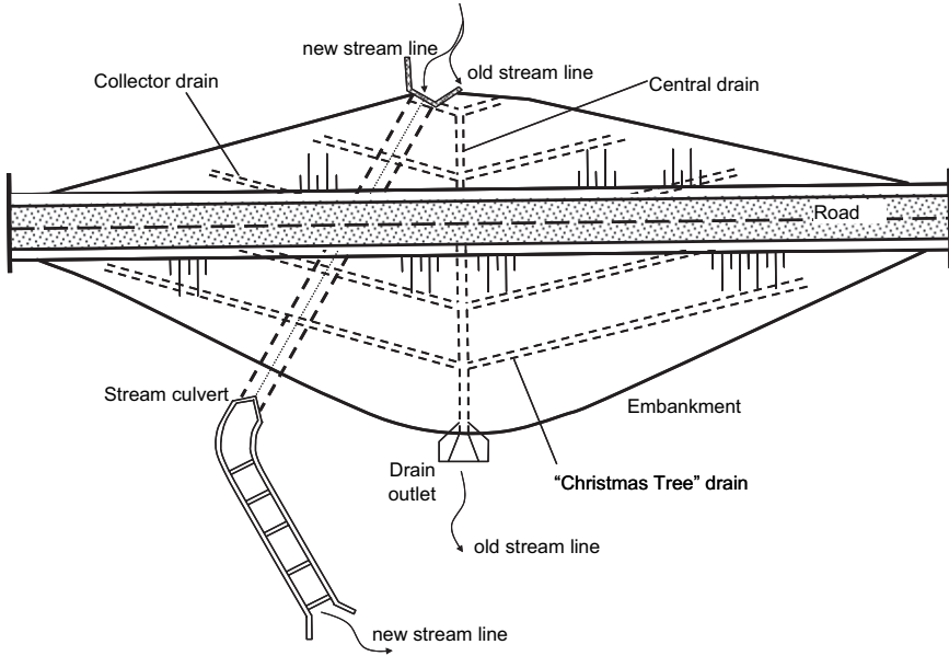
Fig. 13.20 "Christmas tree" drain
