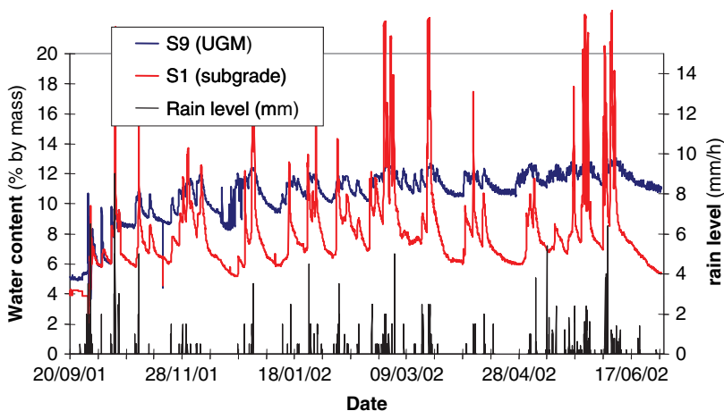
Fig. 8.3 Water content variations in the granular base and subgrade of a low traffic pavement (near the pavement edge)
