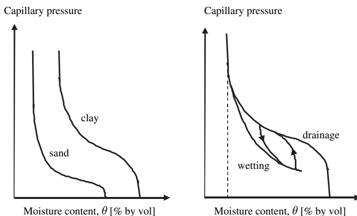
Fig. 2.9 (a) Typical characteristic curves for coarse grained (gravel, sand) and fine grained soils (clay, silt). (b) Soil water characteristic curve showing drainage, wetting and scanning (intermediate) curves. The dotted line represents the irreducible (residual) water content
