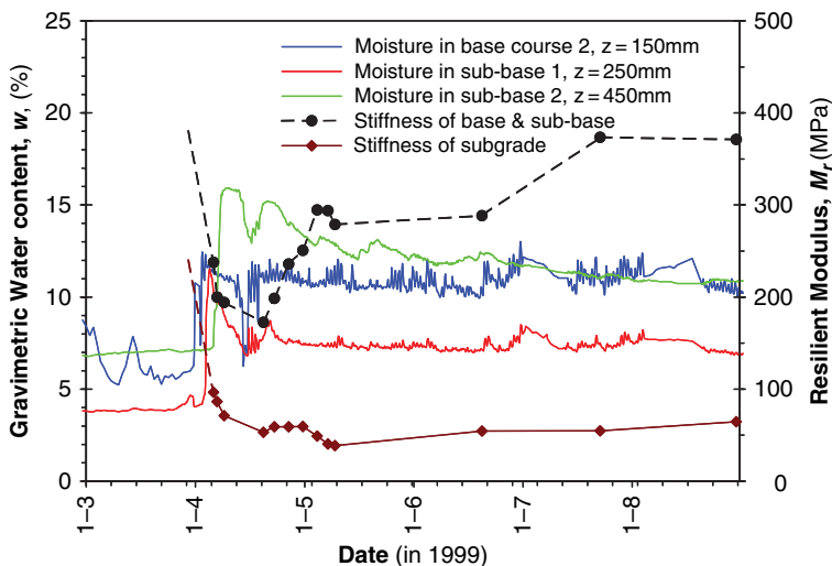
Fig. 8.6 Stiffness and gravimetric water content at one section in SW Iceland
