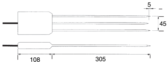
Fig. 3.2 Schema of a TDR-probe. Dimensions are in mm (Ekblad, 2004). Reproduced by permission of Jonas Ekblad
