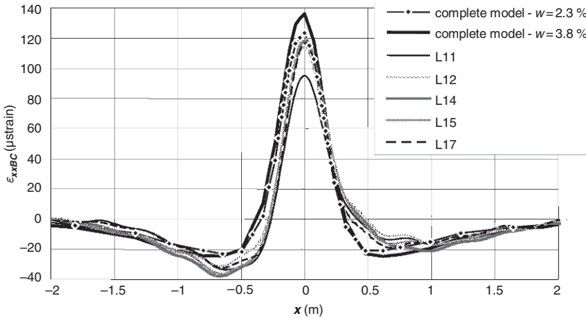
Fig. 11.14 Comparison of experimental and predicted longitudinal strain \epsilon_{xxx} at the bottom of the bituminous layer – load 65 kN
