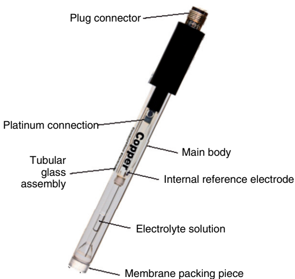
Fig. 7.12 Ion selective electrode (Medek, 1993, Zýka, 1991). In this version, adapted from, and reproduced by permission of van London – pHoenix company
