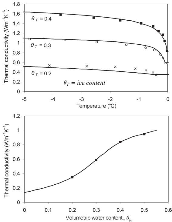
Fig. 4.2 Typical relationships between thermal conductivity and ice content ( top ) and between thermal conductivity and water content ( bottom ) (Hansson et al., 2004). Credit: the Vadose Zone Journal, published by the Soil Science Society of America
