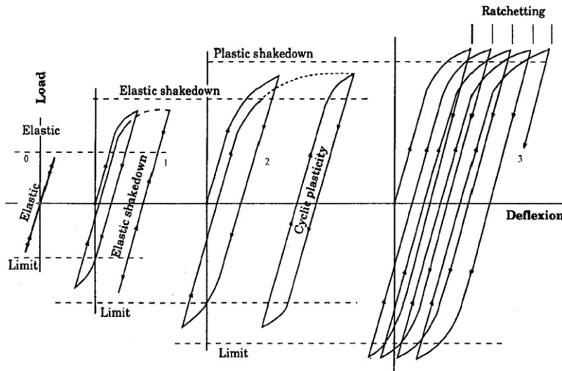
Fig. 9.8 Classical elastic/plastic shakedown behaviour under repeated cyclic tension and compression. Reprinted from Wong et al. (1997), © 1997, with permission from Elsevier
