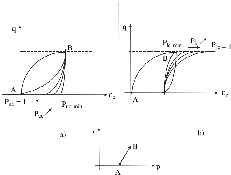
Fig. 9.6 Representation of the influence of the P_{uc/lc} parameters on plastic strains when an unloading and a reloading occur (Chazallon et al., 2006) With permission from ASCE
