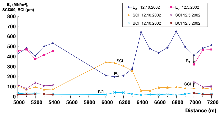
Fig. 8.11 FWD measurement after thawing and before freezing for a poorly performing pavement
