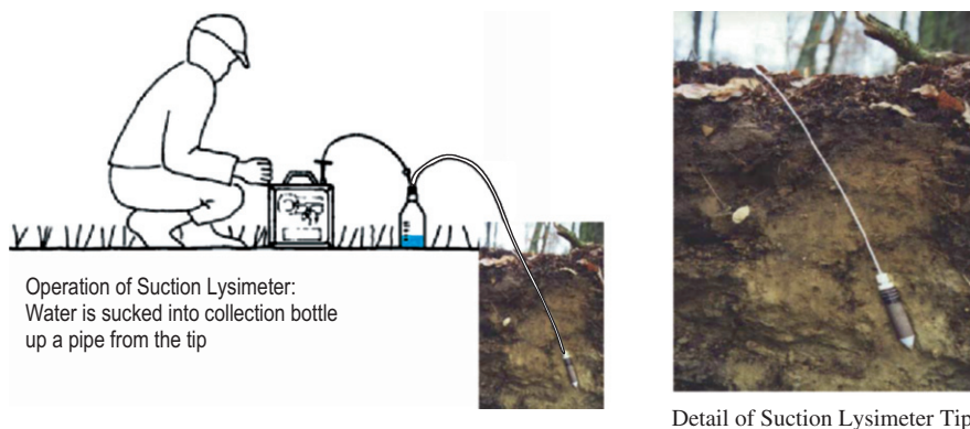
Fig. 7.7 Example of a lysimeter. Reproduced by permission of Prenart Equipment ApS
