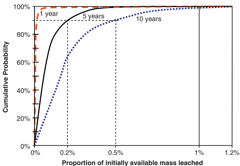
Fig. 11.21 Cumulative probabilities of percentages of initial available mass leached (as observed 0.01m below coal fly ash) after 1, 5 and 10 years. (Apul et al., 2005). Courtesy of D. Apul
