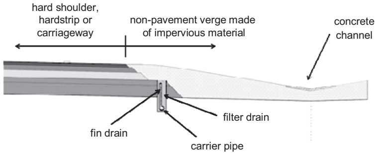
Fig. 13.43 Cuttings – Combined surface water and groundwater filter drain, pavement capping layer with low permeability
