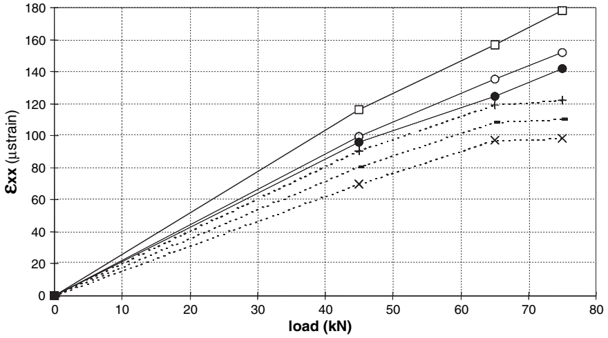
Fig. 11.12 Comparison of experimental and predicted maximum longitudinal strains at the bottom of the bituminous layer, for 3 load levels
