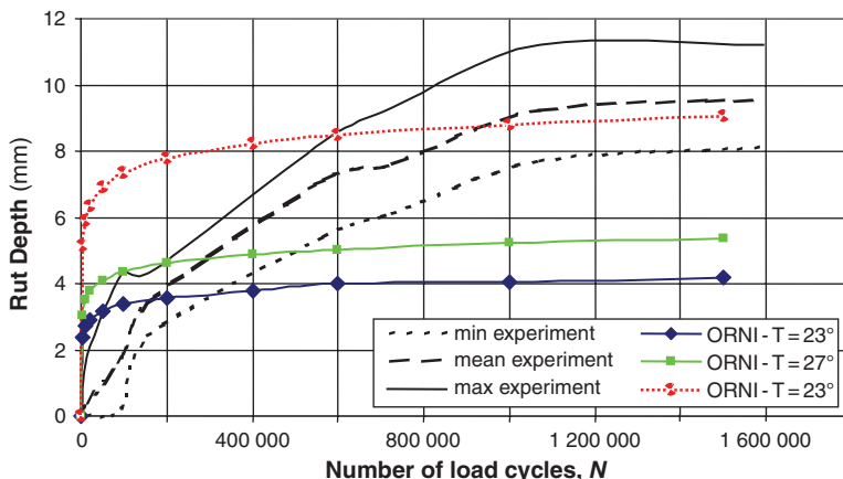
Fig. 11.18 Comparison of maximum rut depths measured on the experimental pavement and predictions with ORNI (rutting of UGM only, different temperatures)
