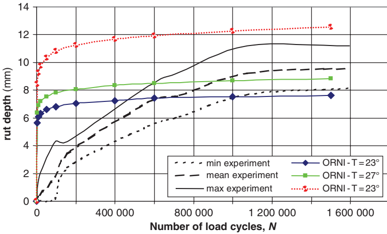
Fig. 11.19 Comparison of maximum rut depths measured on the experimental pavement and predictions with ORNI (rutting of UGM and subgrade, different temperatures)
