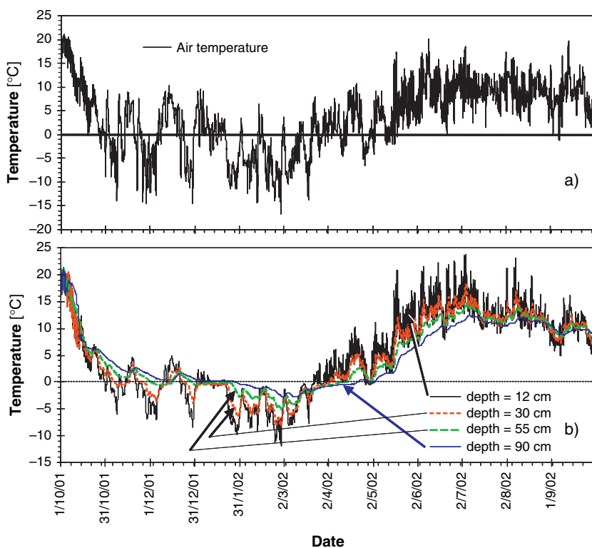
Fig. 4.1 Hourly measurement during one year in SW Iceland (a) of air temperature and (b) at four depths in a pavement structure
