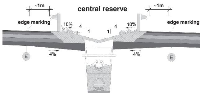
Fig. 13.6 Typical pavement cross-falls. E = position 1 m inwards from the edge of the pavement. Similar cross-falls will exist at road edges
