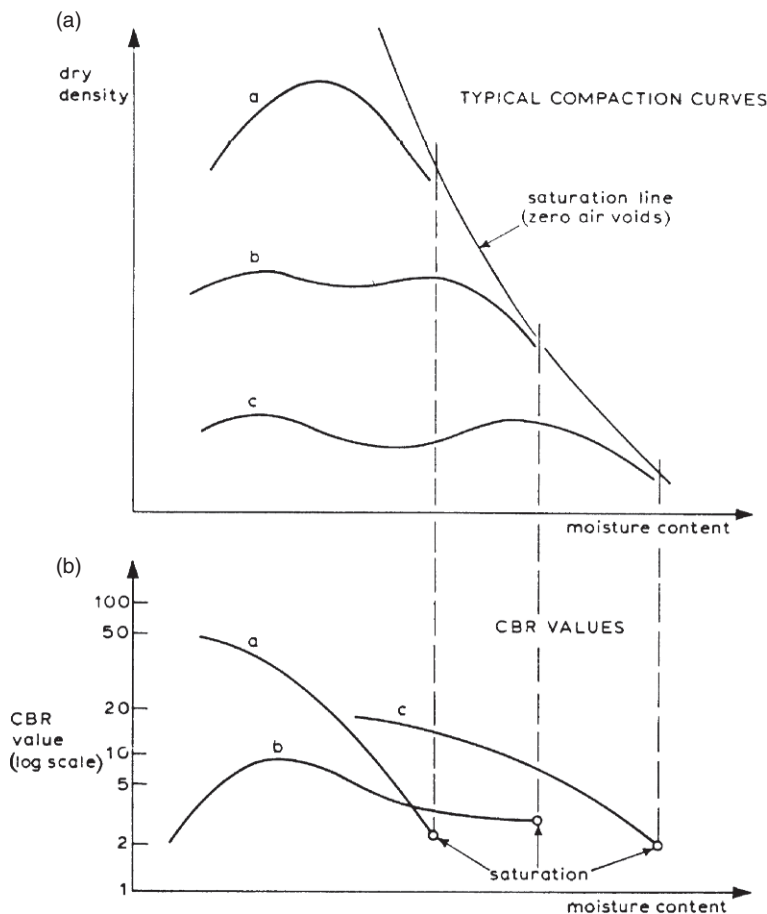
Fig. 10.8 CBR values related to moisture (water) content and compaction curves for typical soils: (a) well-graded silty sand with clay, (b) uniform fine sand, (c) heavy clay (Head 1994). © 1996, copyright John Wiley & Sons Limited. Reproduced with permission
