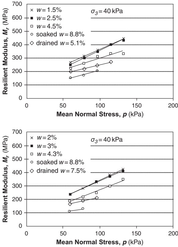
Fig. 10.13 Resilient response at different water contents for grading 0.4 or 0.3 (Ekblad and Isacson, 2006). Reproduced with permission of Lavoisier
