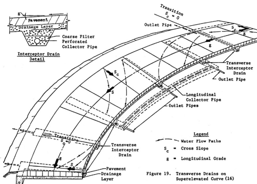
Fig. 13.18 Transverse drains on super-elevated curve. Courtesy of the FHWA (1980)
