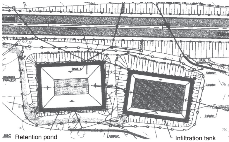
Fig. 13.33 Plan of environment with extremely high sensitivity. A combination of various types of water treatment is included
