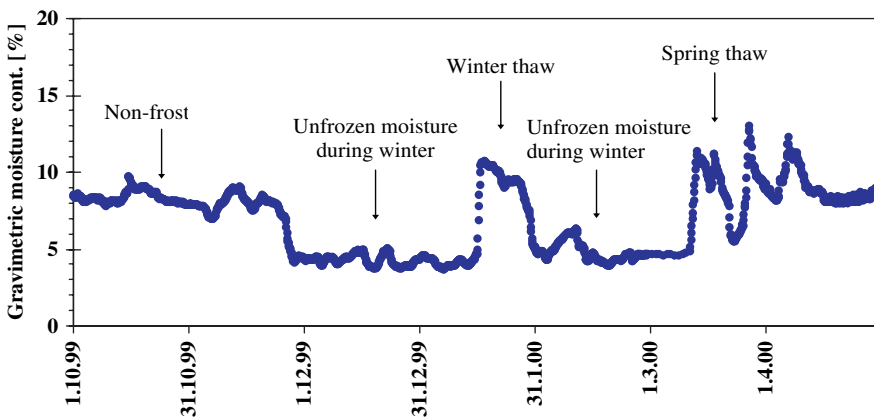
Fig. 3.3 Gravimetric water content in a sub-base layer at 25 cm depth in a low volume road. The readings were carried out at three hour intervals
