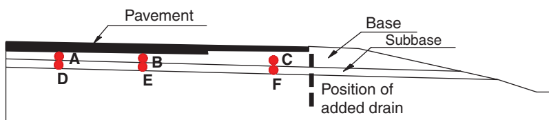
Fig. 11.4 Degree of saturation at equilibrium when a drain is installed at the pavement – shoulder contact, adapted from Alonso et al. (2002)
