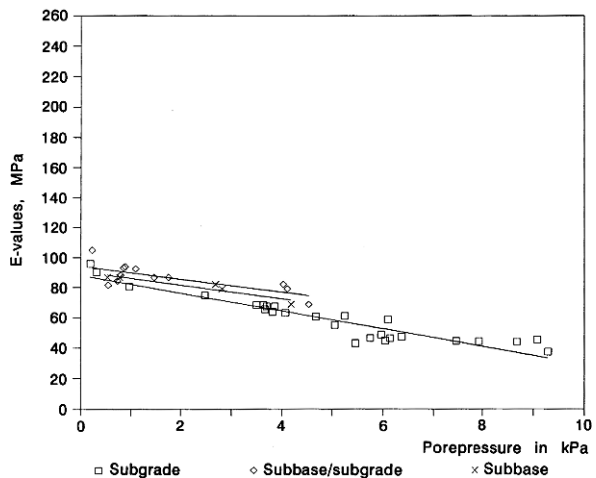
Fig. 10.21 E-values versus positive pore water pressure (Krarp, 1995). Reproduced by permission of the Danish Road Institute
