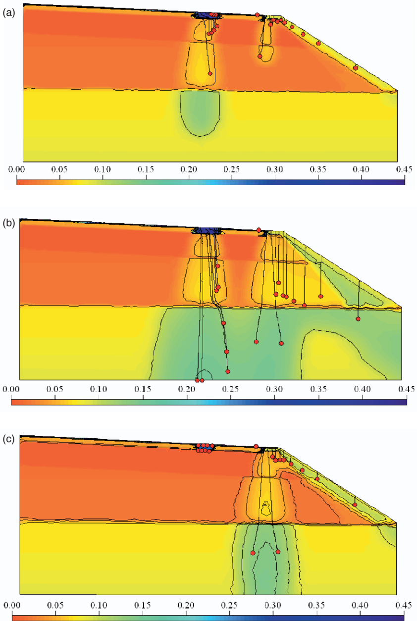
Fig. 11.6 The simulated volumetric water content, \theta , in a model road (a) after a light rainfall event (top), (b) after a heavy rainfall event (middle), (c) after a moderate rainfall event using small fracture-zone permeability (bottom) The particles illustrate the flow paths of the infiltrated rainwater. The vertical scale is exaggerated for clarity
