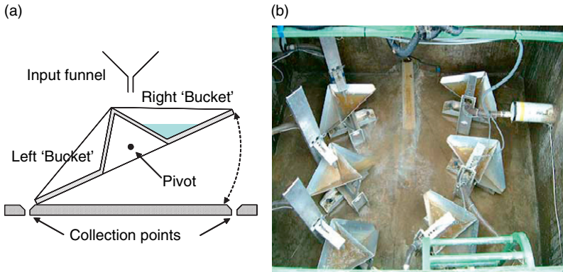
Fig. 7.2 Tipping bucket system to measure flow: (a) principle of operation; (b) with adjacent, periodic, sampling system (from Hendry et al., 2004). Photo. credit: Lincoln University, New Zealand
