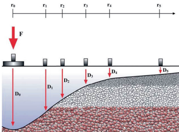
Fig. 10.6 Schematic overview of Falling Weight Deflectometer testing
