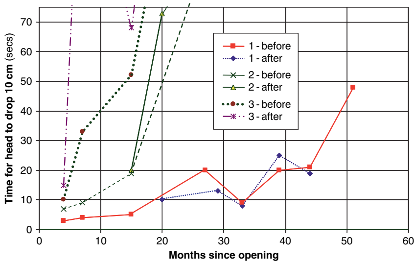
Fig. 5.16 Out-flow time (s/10 cm) in the wheel-track as a function of pavement age in months before and after cleaning (adapted from Bendtsen et al., 2005)
