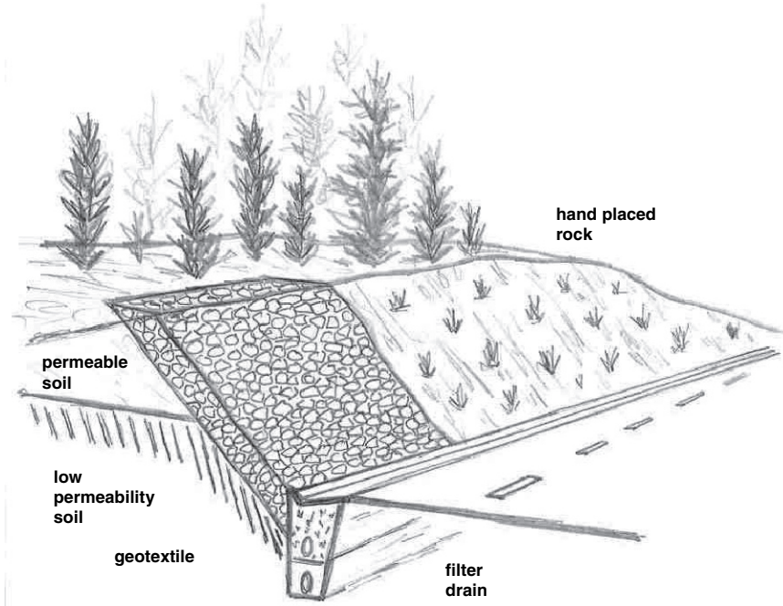
Fig. 13.21 Drainage masks
