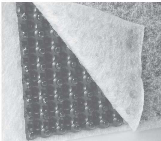
Fig. 13.16 Examples of geocomposites used in fin drainage systems
