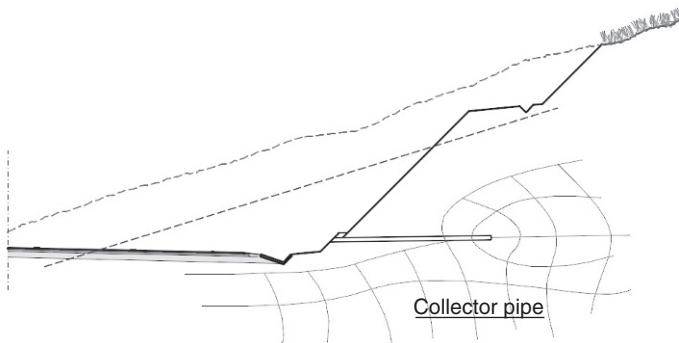
Fig. 13.17 “Californian drain”
