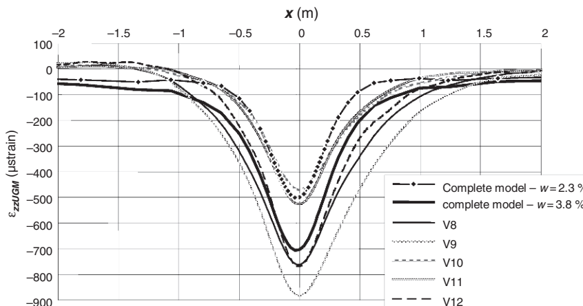
Fig. 11.16 Comparison of experimental and predicted vertical strain \varepsilon_{zz} at the top of the granular layer – load 65 kN
