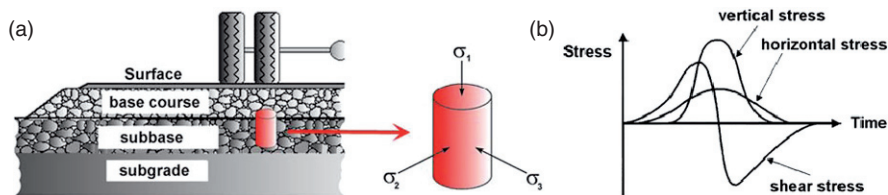
Fig. 10.1 Stresses in an unbound granular material layer. (a) Typical pavement structure and stresses, (b) induced stresses in a pavement element due to moving wheel load (Erlingsson, 2007)
