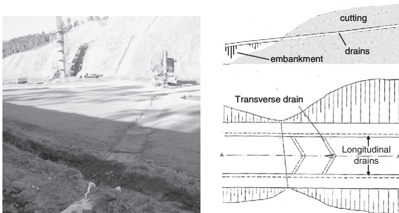
Fig. 13.26 Transverse drains
