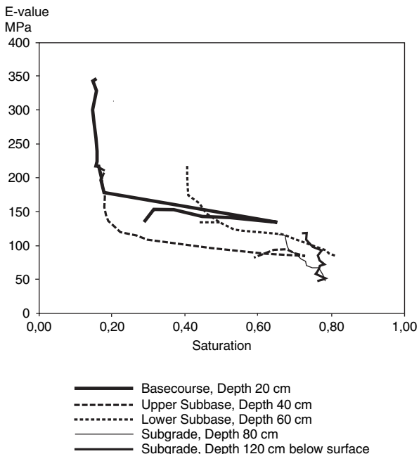
Fig. 10.22 Measured saturation (nuclear probe) and E-values (ELMOD) (Krarup, 1995). Reproduced by permission of the Danish Road Institute
