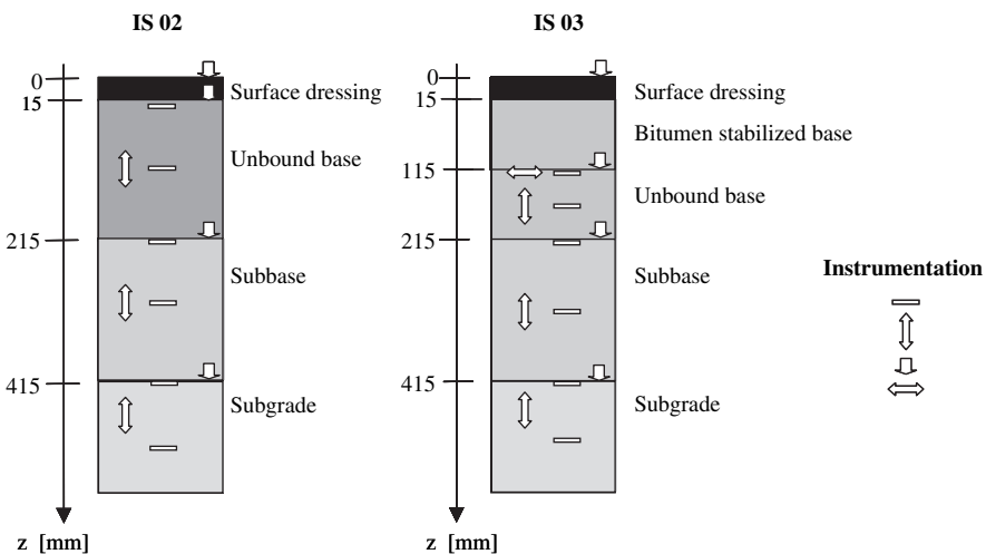
Fig. 11.8 Two test pavement structures: (a) IS02 is an unbound structure and (b) IS03 is a bitumen stabilized structure Note: The instrumentation used for the response measurements is shown as well.
