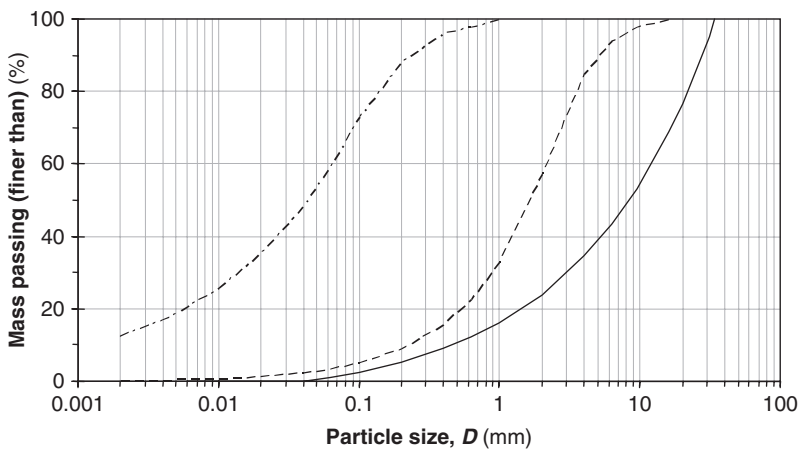
Fig. 2.4 Three different grain size distribution curves
