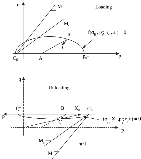
Fig. 9.5 Yield surfaces during loading and unloading in the p - q space (Chazallon et al., 2006). With permission from ASCE
