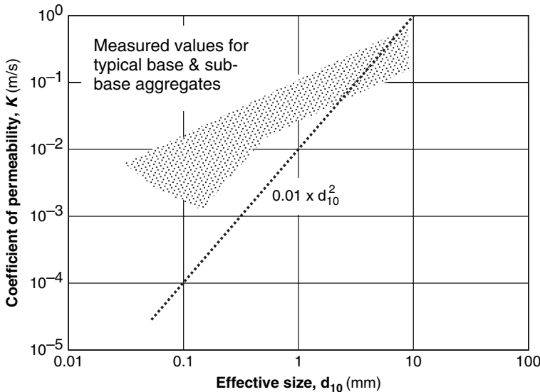
Fig. 2.7 Illustration of mis-match between Hazen’s estimation and measured values from road aggregates (adapted from Jones and Jones, 1989)
