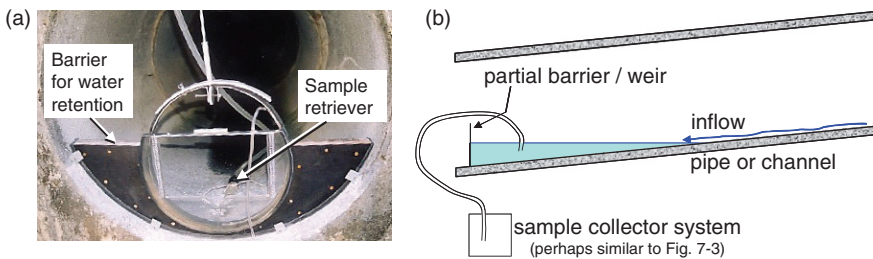
Fig. 7.1 Device for runoff sampling in a (a) road ditch section or drainage pipe and (b) principle of implementation
