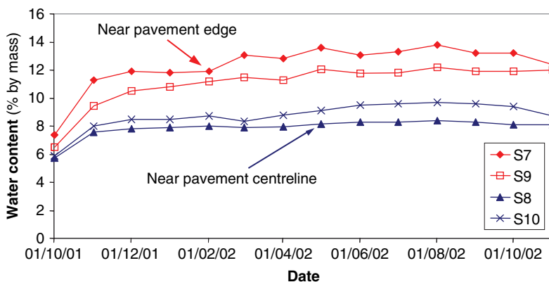
Fig. 8.4 Monthly average water contents in the granular base, at the centre and near the edge of the pavement
