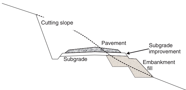
Fig. 1.4 Indicative highway cross section
