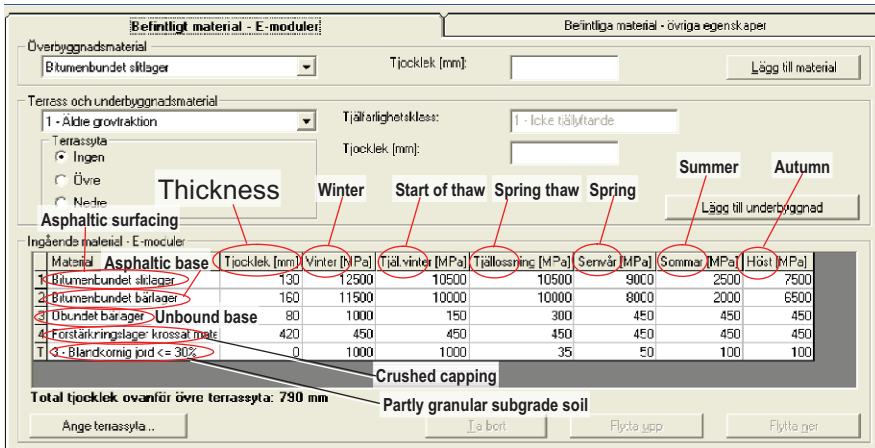
Fig. A.2 Road design dependent on season and layer – Swedish case using PMSObjekt (Vägverket, 2005) showing moduli of pavement layers in 6 “seasons”
