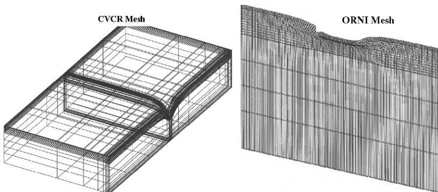
Fig. 11.17 Finite element meshes used for the modelling of the experimental pavement
