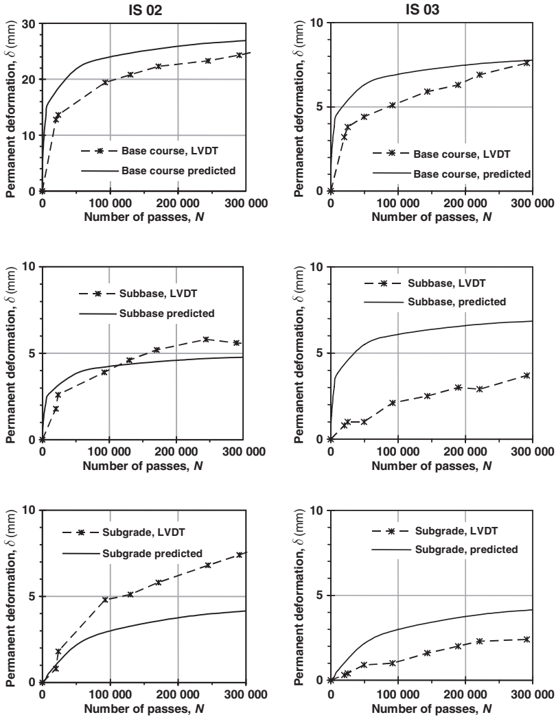
Fig. 11.10 Prediction versus measurements of permanent deformation development for the three unbound layers as a function of load repetition for both pavement structures IS02 and IS03
