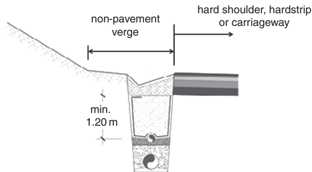
Fig. 13.40 Cuttings – Standard concrete channel in verge with drain and pipe
