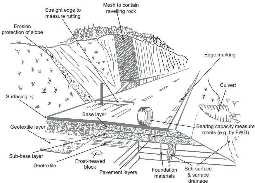
Fig. 13.8 The drainage layer is often directly connected to the longitudinal drains, but can also continue to the open slope side. In this example, surface water runoff also arrives at the drainage layer at the side of the road. Therefore the figure shows a sub-base drainage layer where water can flow either way (from Vägverket, 2004). Courtesy of the Swedish Road Administration
