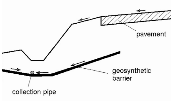
Fig. 13.35 Application of geosynthetic barrier (GBR)
