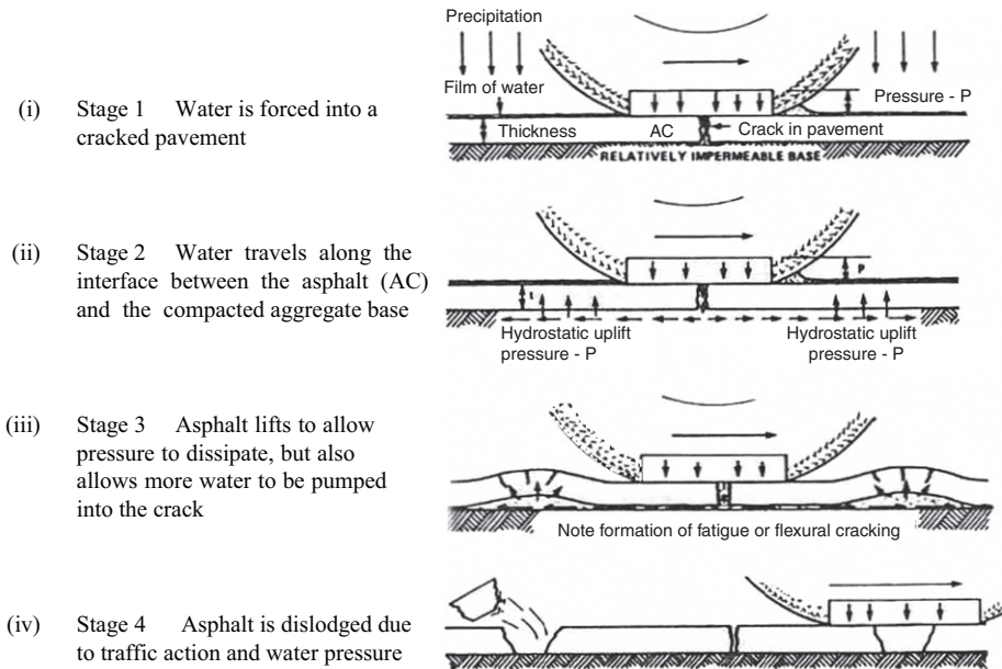
Fig. 8.1 Layer separation and pothole formation (from Gerke, R.J. (1979), cited by Lay (1986)). Reproduced by permission of M. G. Lay
