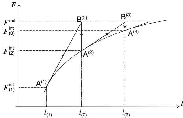
Fig. 11.1 Illustration of the Newton-Raphson process
