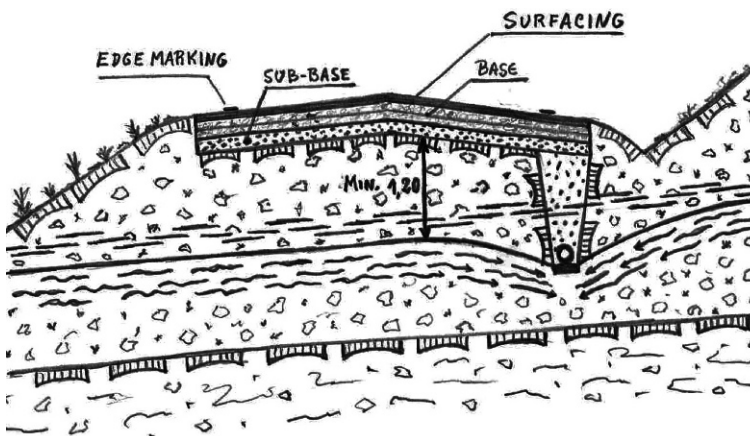
Fig. 13.13 Conventional trench drain
