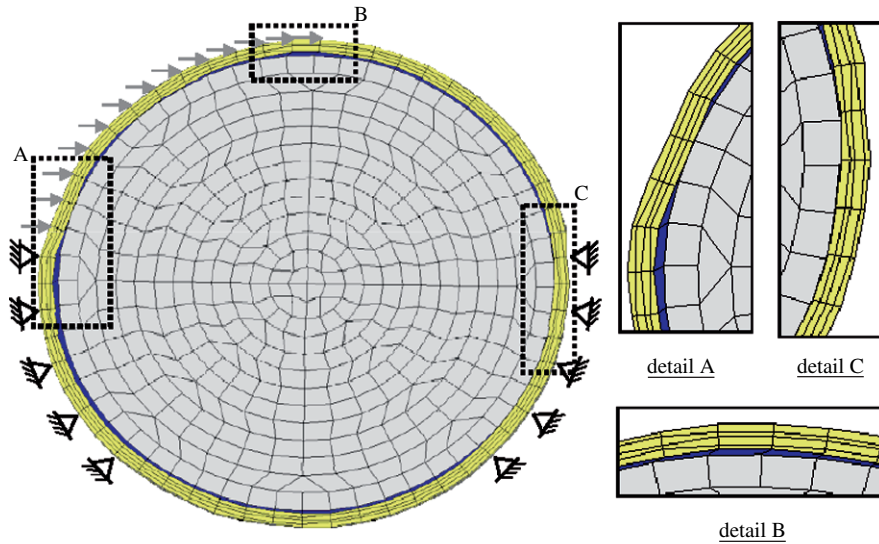
Fig. 5.14 Simulation of ravelling in an aggregate coated in a mastic film, subjected to a mechanical and water-induced damage (Kringos & Scarpas, 2006) The dark areas in the details are areas of de-bonding.
