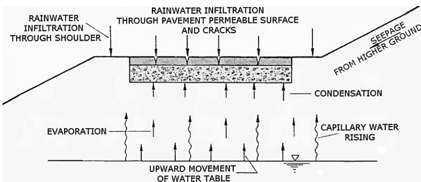
Fig. 8.2 Possibilities of water movements into the pavement zone (from Moris & Gray, (1976) cited by Lay (1986)). Reproduced by permission of M. G. Lay
