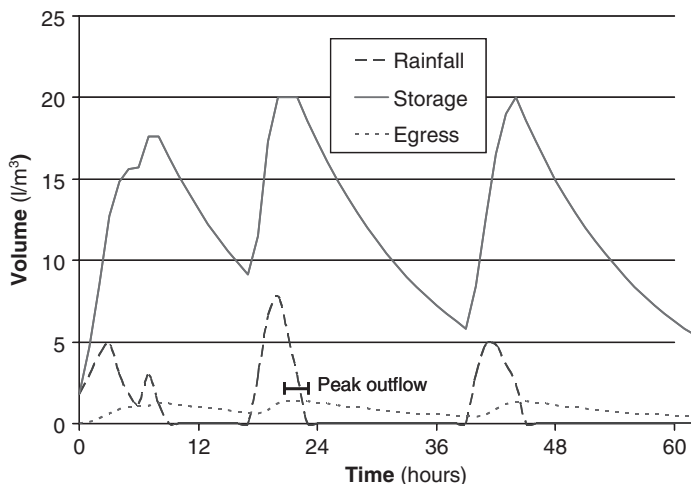
Fig. 13.11 Sample rainfall, storage and outflow hydrograph
