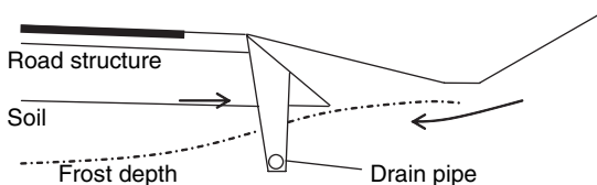
Fig. 13.27 A deep drain example from Finland
