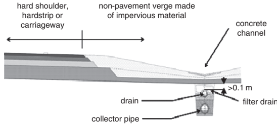
Fig. 13.42 Cutting – Combined surface water and groundwater filter drain and drain pipe
