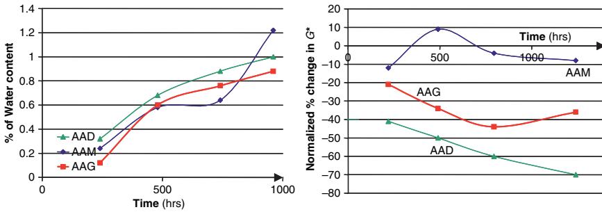
Fig. 5.6 (a) water absorption in three SHRP binders (b) reduction of binder stiffness, G^* , due to water infiltration (Huber, 2005). Reproduced by permission of N. Kringos
