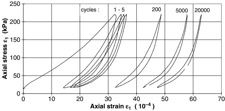
Fig. 9.4 Example of stress-strain cycles obtained in a repeated load triaxial test on a granular material (Hornych et al., 1998)
