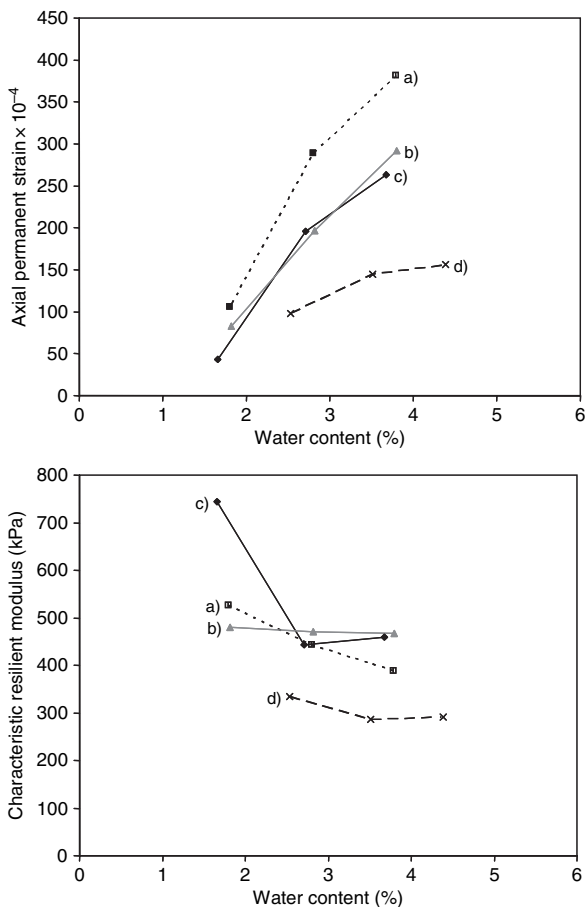
Fig. 10.11 Influence of water content on permanent deformations and modulus of elasticity for some unbound granular materials. (a) Crushed gravel from gravel pit Hrušica, (b) dolomite from quarry Lukovica, (c) dolomite from quarry Kamna Gorica, (d) gravel from Hoče (Pavšič, 2006)
