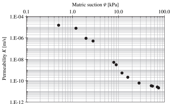
Fig. 3.12 Permeability as a function of matric suction in an unsaturated soil specimen
