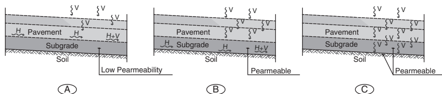
Fig. 13.4 Cases for water infiltration and flow in the pavement sub-surface
