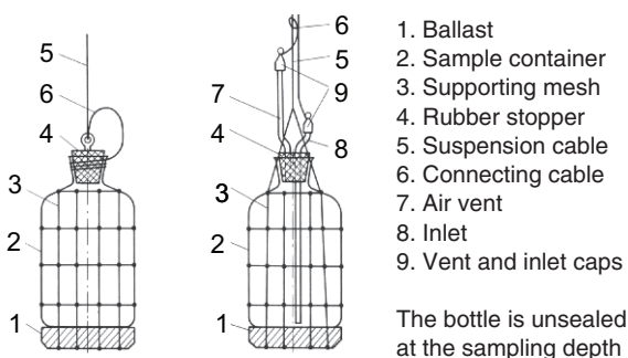
Fig. 7.4 Simple bottle type samplers. Left: Meyer's submersible bottle; Right: Submersible bottle based on Dussart's principle
