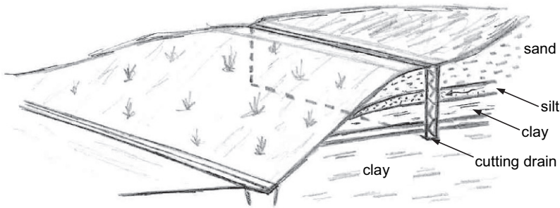
Fig. 13.24 Cutting drain
