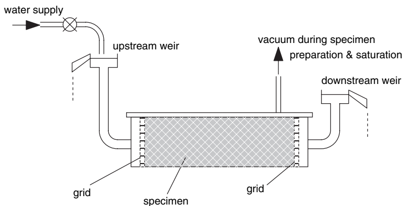
Fig. 3.6 Department of Transport (1990) horizontal aggregate permeameter
