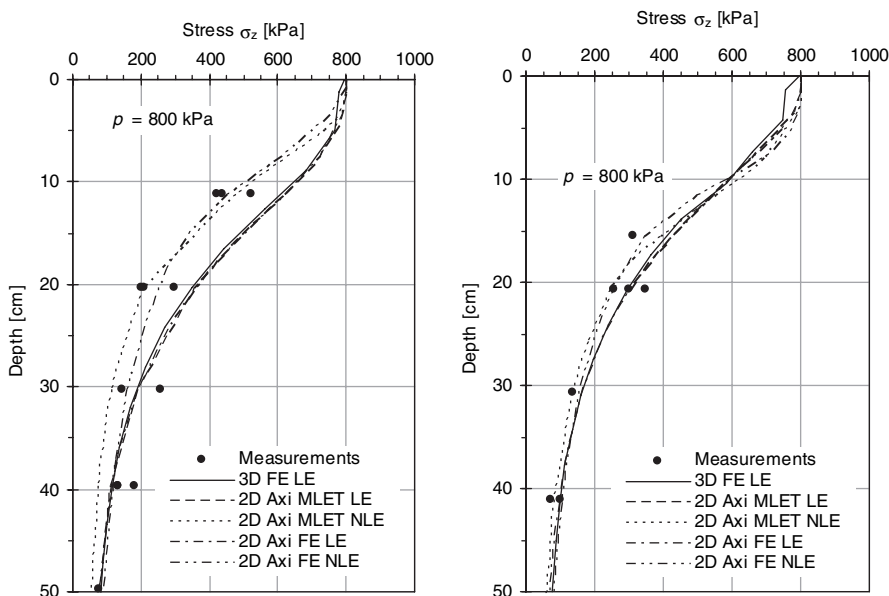
Fig. 11.9 Comparison of measured and calculated vertical induced stresses under the centre of a single tyre as a function of depth for both pavement structures IS02 and IS03
