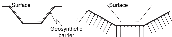
Fig. 13.36 Elementary mis applications of geosynthetic barriers
