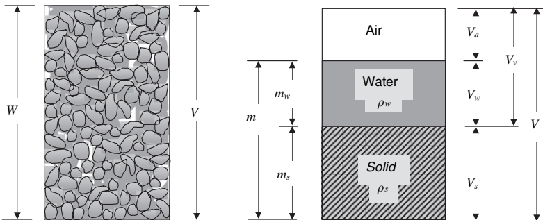
Fig. 2.5 A three phase diagram of an unsaturated element of aggregates
