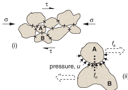
Fig. 9.1 Schematic of inter-particle forces. (i) an assembly of particles is subjected to some external normal, \sigma , and shear, \tau , stresses, which are carried through the assembly at the contact points as shown by the black bars; (ii) when the pore space between particles A and B is pressurised by a fluid at pressure, u , particles A and B experience a pressure on them (illustrated only for A, not illustrated for B) which reduces the inter-particle force, f_n , and makes shear, f_s , more easy to take place because of reduced friction at the contact between the particles
