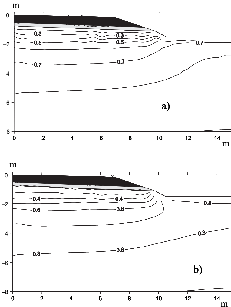
Fig. 11.5 Distribution of degree of saturation for a pavement in a Mediterranean climate. Evaporation through pavement allowed. (a) 1st July, (b) 1st December, adapted from Alonso et al. (2002)
