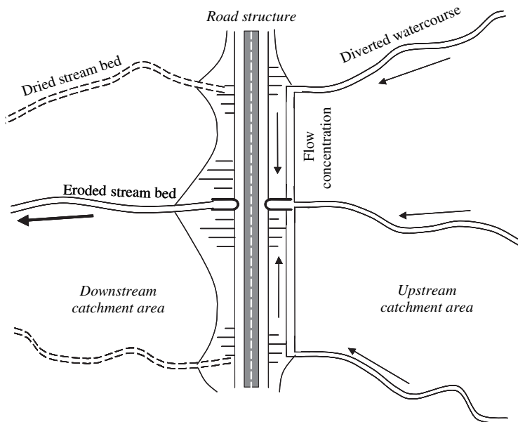
Fig. 12.3 Interrelation between road and streams
