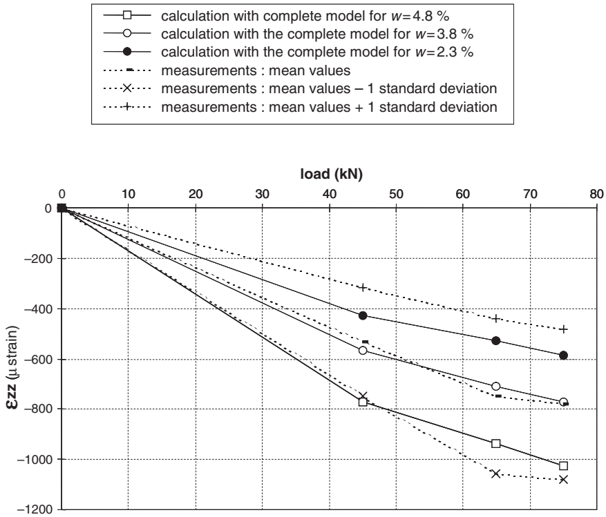
Fig. 11.13 Comparison of experimental and predicted maximum vertical strains at the top of the granular layer, for 3 load levels
