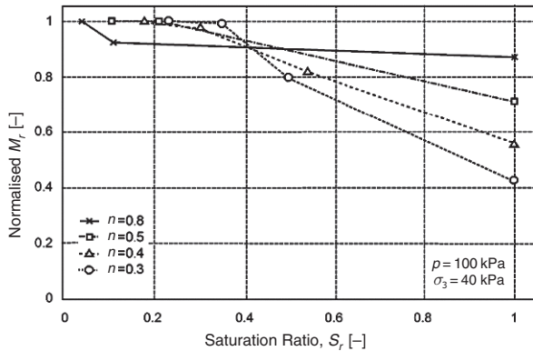
Fig. 10.14 Normalized resilient modulus as a function of degree of saturation ( p = 100 kPa and \sigma_3 = 40 kPa) (Ekblad and Isacson, 2006). Reproduced with permission of Lavoisier
