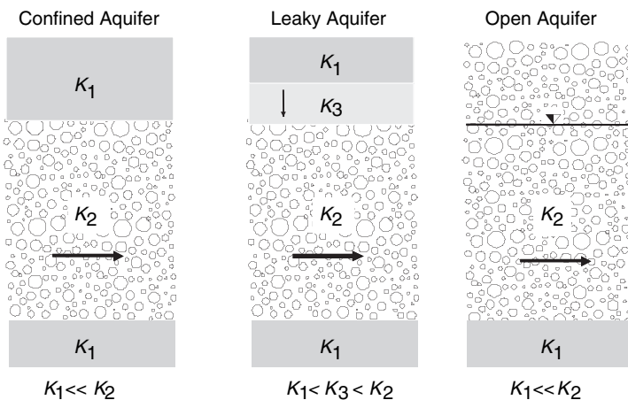
Fig. 2.3 Hydrodynamic classification of aquifers. K is permeability
