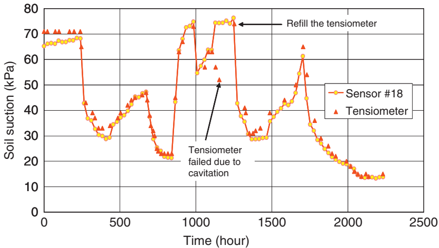
Fig. 3.15 Comparison between laboratory soil suction measurements with tensiometers and TCS. Reproduced with permission of D. Fredlund
