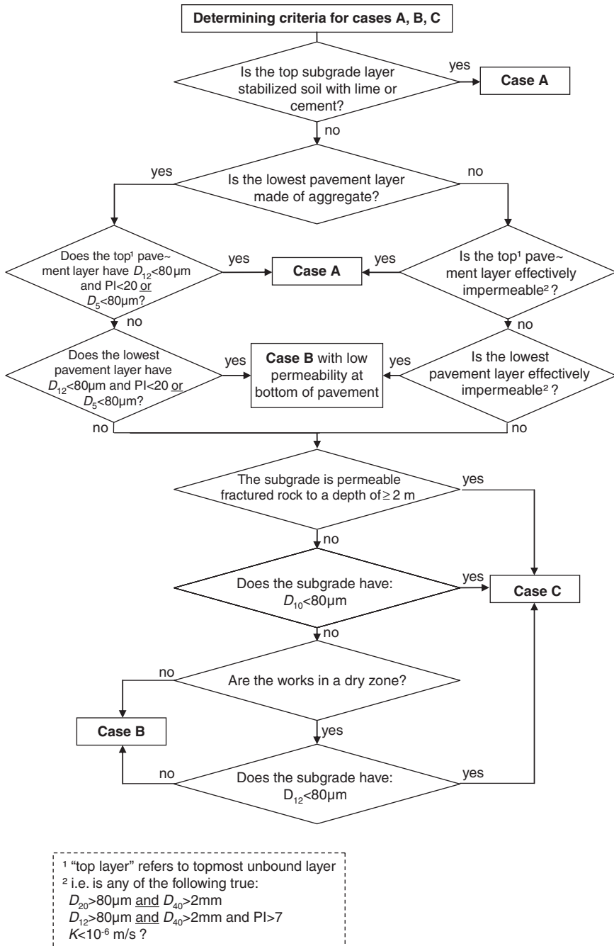
Fig. 13.5 Selection of appropriate drainage approach as per Fig. 13.4. For explanation of the D_n notation, see Chapter 2, Section 2.4.1
