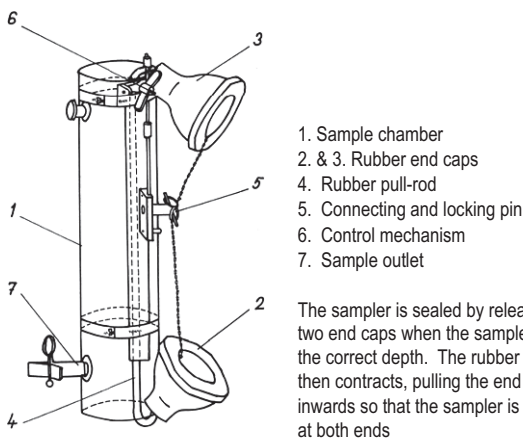
Fig. 7.5 Van Dorn's water bottle (or flushed sampler), vertical sampling model
