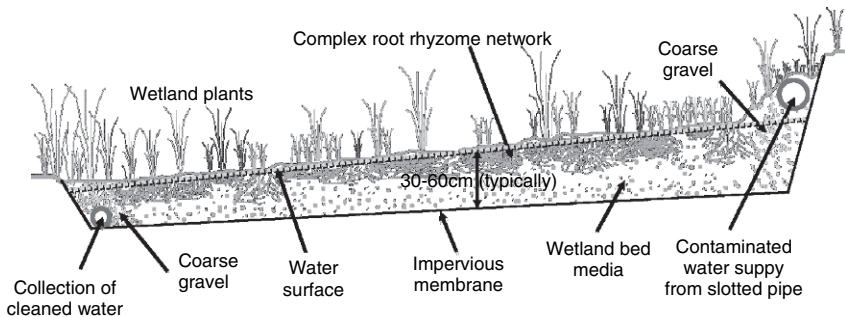
Fig. 12.2 A horizontal subsurface-flow constructed wetland (NAVFAC, 1998)
