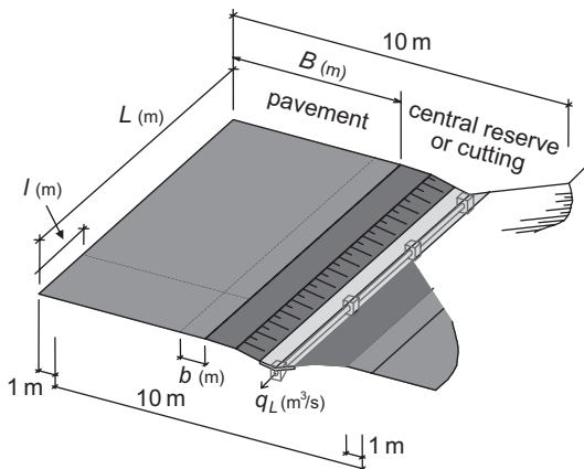
Fig. 13.39 Drainage zones for a section of carriageway and hinterland (adapted from Carreteras (2004))
