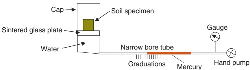
Fig. 3.16 Suction plate device
