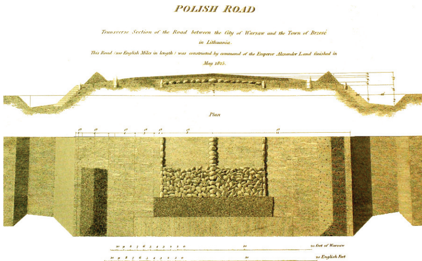
Fig. 1.3 Facsimile of Telford's design for a road from Warsaw to Brzesć 1 (Telford, 1838)
