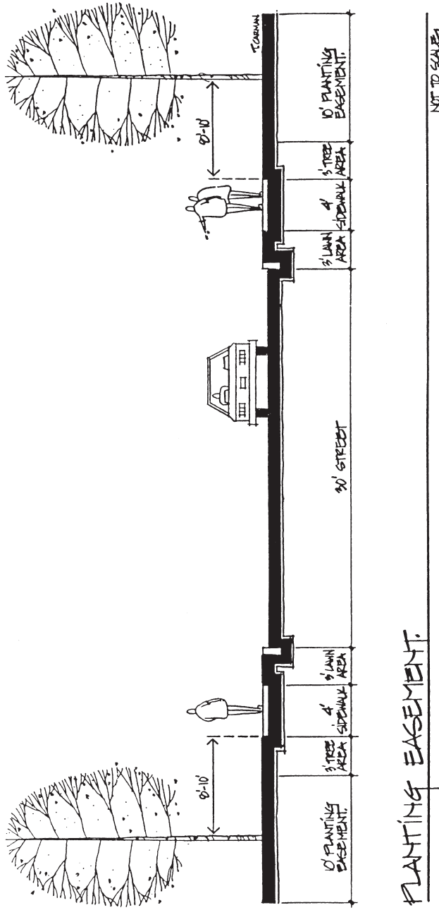
FIGURE 3. Planting easement sketch. Sketch, Tom Carman.
