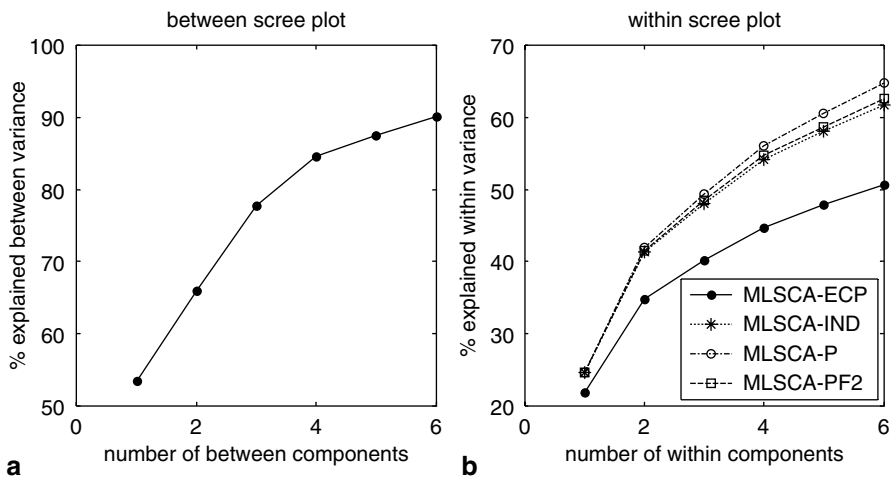
Fig. 14.2 Percentage of (a) explained between-variance for MLSCA solutions with the number of between-components varying from 1 to 6, and (b) explained within-variance for MLSCA-ECP, MLSCA-IND, MLSCA-PF2, and MLSCA-P solutions with the number of within-components varying from 1 to 6
