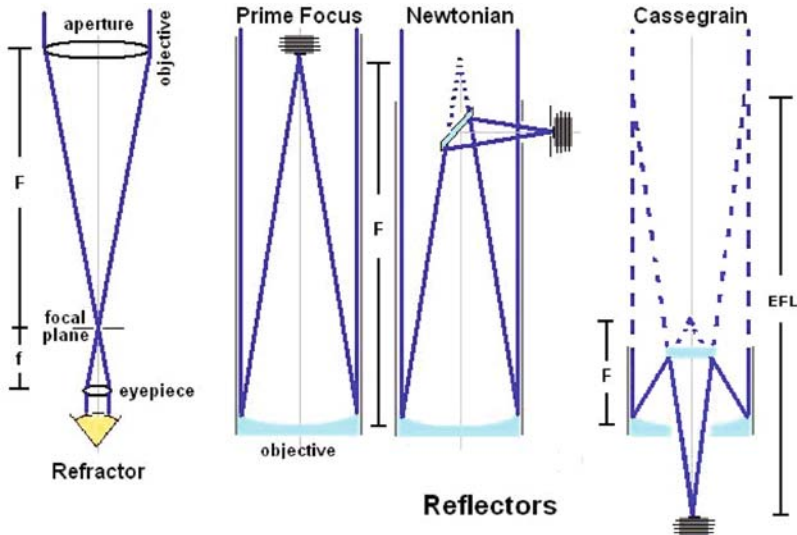
Fig. 3.18. Schemes of the different types of telescopes.
