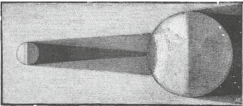
Fig. 4.3. Graphical explanation of total solar eclipses, from Guillemin (1883).
