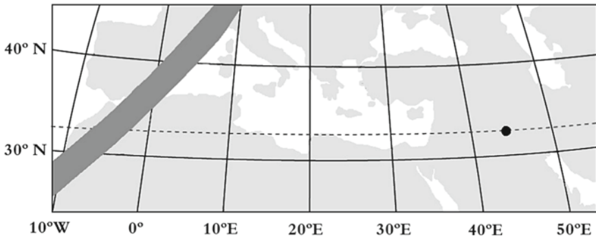
Fig. 4.10. Computed track of totality for the eclipse of 15 April 136 BC (shadow band) assuming \Delta T = 0 . Totality phase was observed from Babylon. The latitude of this place is marked with a dashed line (adapted from Stephenson, 2003).
