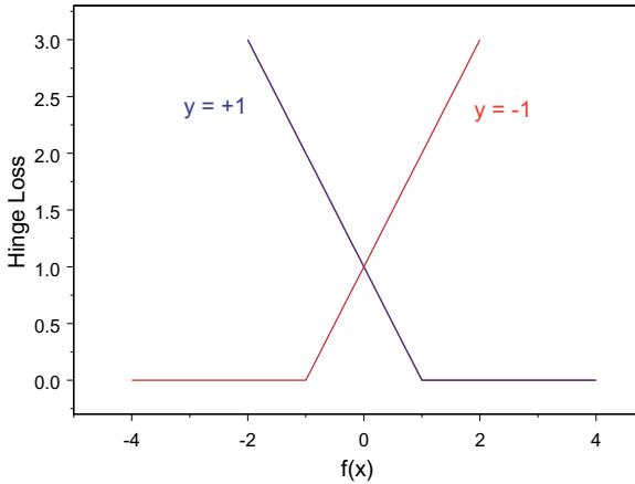
FIGURE 11.4. Hinge loss function (1 - yf(\mathbf{x}))_+ for y = -1 and y = +1 .
