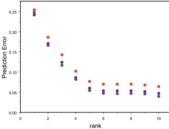
FIGURE 6.5. Prediction errors for PAH example ( n = 50, r = 27, s = 10 ) plotted against rank of the regression coefficient matrix. The PEs were computed using cross-validation: CV/5 (red dots), CV/10 (blue dots), and CV/n (purple dots). The results show a leveling-off of the PE at rank t = 5 .
