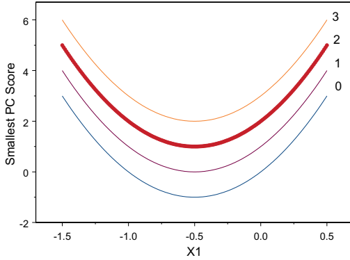
FIGURE 16.2. Graphs of X_2 = 4X_1^2 + 4X_1 + a , where a = 0, 1, 2, 3 . Superimposed on these graphs are the scores (red points) from the smallest PC (actually, PC_5/0.0174 + X_2 ) derived from a quadratic PCA on the generated data.
