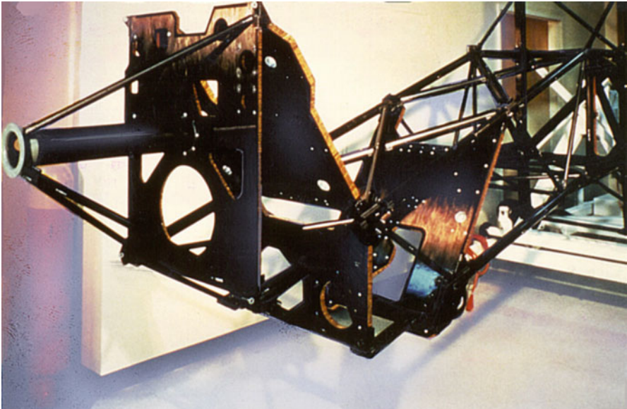
Fig. 5.26 Intelsat 5 has a primary structure and several antennas made of carbon fiber PMCs (courtesy of Fiberite Co.)
