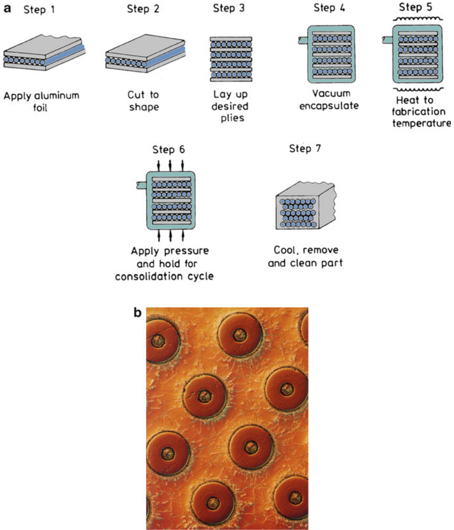
Fig. 6.8 (a) Schematic of diffusion bonding process. (b) The microstructure of SiC fiber/titanium matrix composite made by diffusion. Each fiber is 142 \mu\text{m} in diameter. [Courtesy of J. Baughman]
