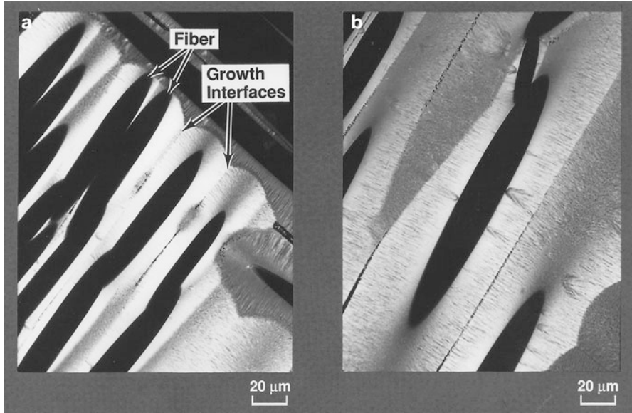
Fig. 7.7 An example of the microstructure of a Nicalon fiber/SiC matrix composite obtained by CVI. (Courtesy of R.H. Jones). Note the growth interfaces within the matrix indicated by arrows
