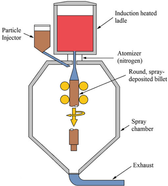
Fig. 6.7 Schematic of the spray forming process
