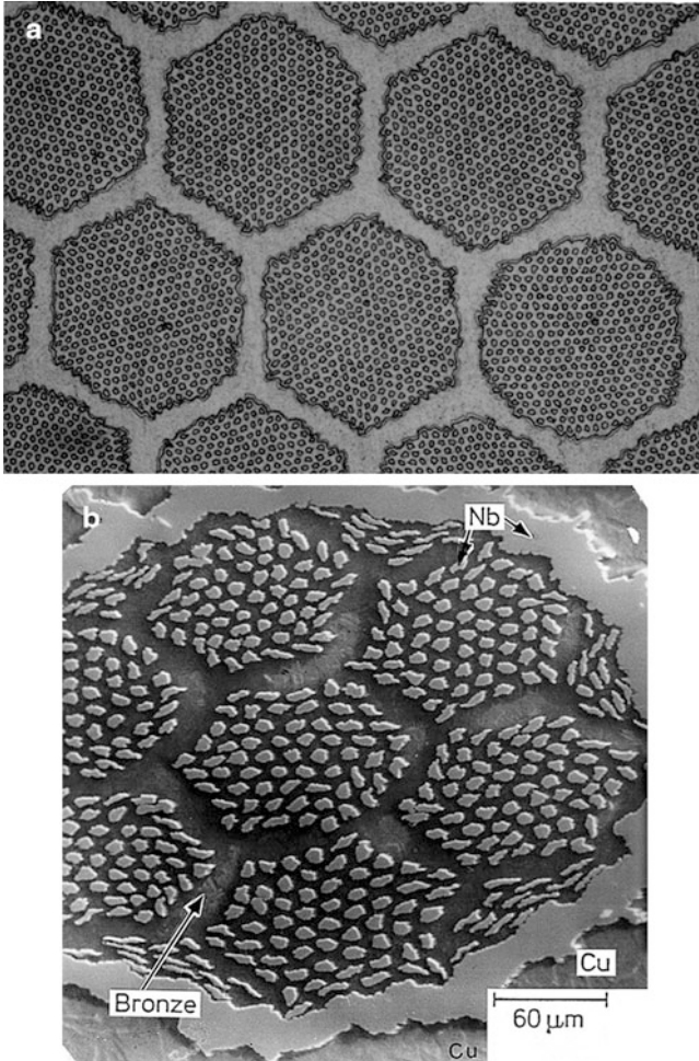
Fig. 9.9 (a) An Nb 3 Sn/Cu composite superconductor used in high-field magnets. Each little dot in this picture is a 4- \mu m diameter Nb 3 Sn filament. Hexagonal strips are niobium diffusion barriers for tin (courtesy of Hitachi Cable Co.). (b) Scanning electron micrograph of a niobium/bronze composite before the heat treatment to form Nb 3 Sn
