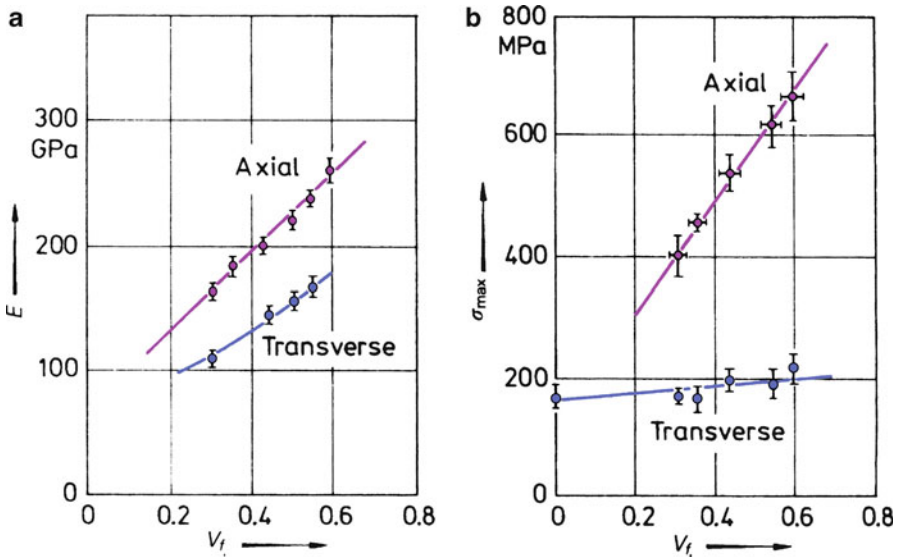
Fig. 6.19 Properties of Al_2O_3/Al-Li composites as a function of fiber volume fraction ( V_f ): (a) axial and transverse Young’s modulus vs. fiber volume fraction, (b) axial and transverse ultimate tensile strength vs. fiber volume fraction. [From Champion et al. (1978), used with permission]
