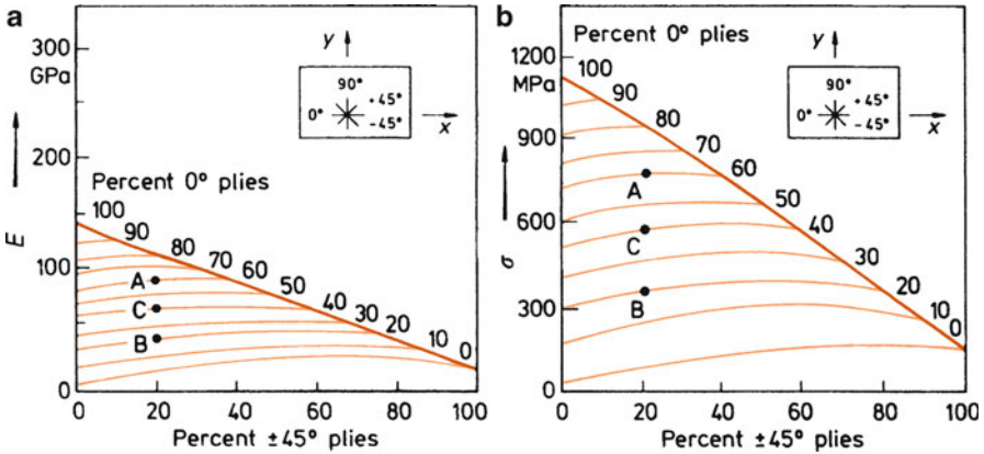
Fig. 14.1 Carpet plots for 65 % V_f carbon/epoxy with a 0^\circ/\pm 45^\circ/90^\circ stacking sequence: (a) Young’s modulus, (b) tensile strength. [From Kligler (1979), used with permission]
