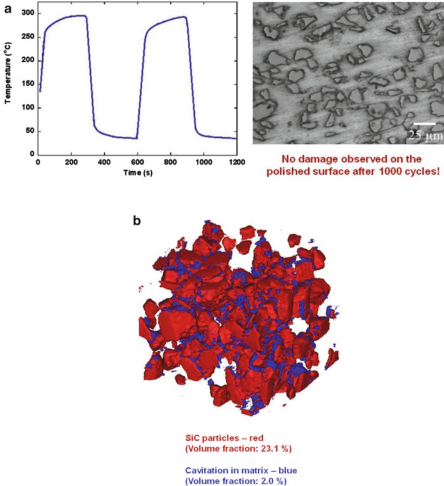
Fig. 13.15 (a) Surface of SiC p /Al composite after thermal cycling. No damage is visible on the surface. (b) Same sample examined by X-ray tomography shows damage in the interior. Blue color shows cavitation, about 2 % by volume. The SiC particles are about 25–30 μm in diameter and 20 vol.% [courtesy of N.C. Chapman and N. Chawla, Arizona State University]
