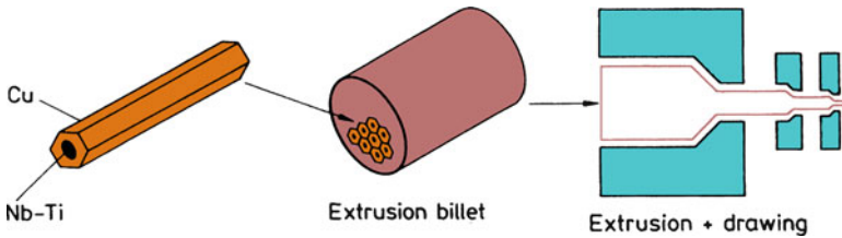
Fig. 9.5 Fabrication route for Nb-Ti/Cu composite superconductors
